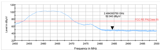
802.11g-Channel 11 Peak
