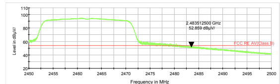
802.11n HT20 -Channel 11 Average
