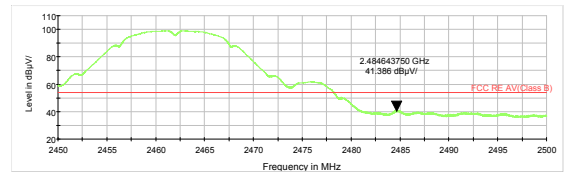
802.11g-Channel 11 Average
