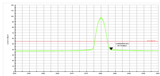
3DH5-Channel 78: Average
