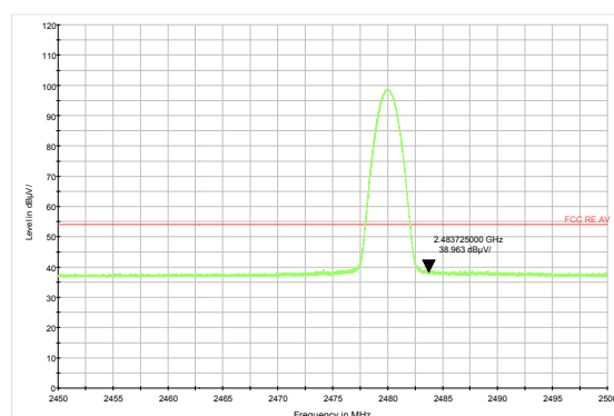
DH5-Channel 78: Average
