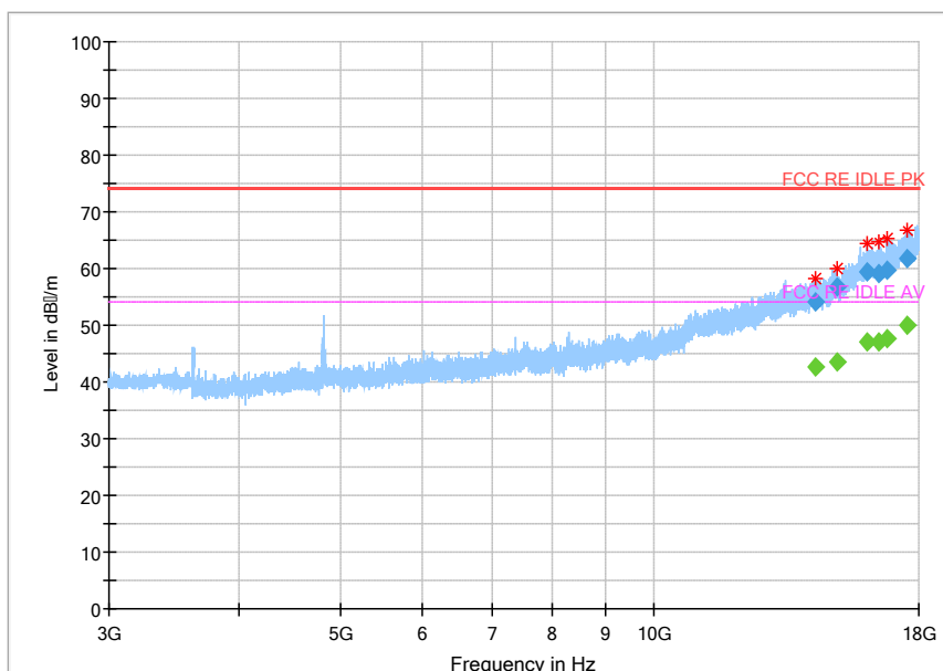
Fig.106 Radiated Spurious Emission (802.11g,Ch1,3GHz~18GHz)
