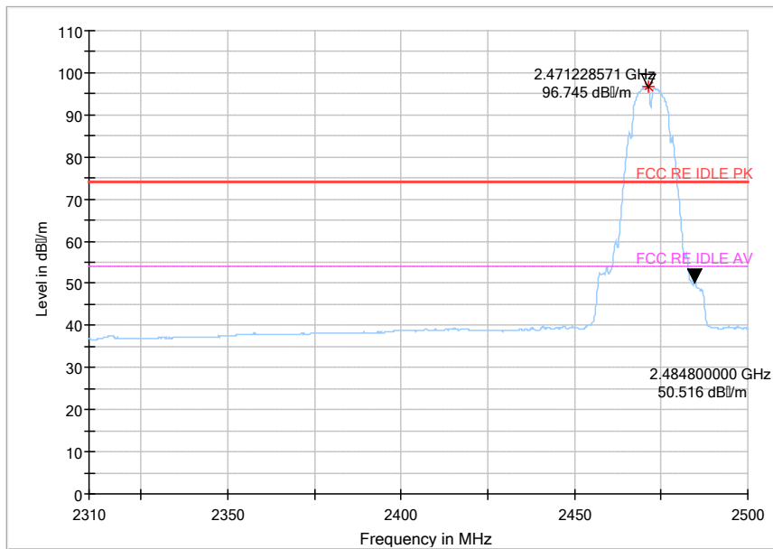
Fig.122 Radiated emission (Power): 802.11b, Ch13
