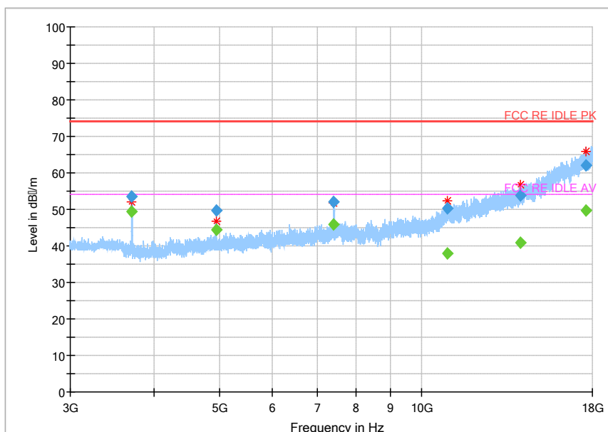
Fig.136 Radiated Spurious Emission (802.11g, Ch13, 3GHz~18GHz)
