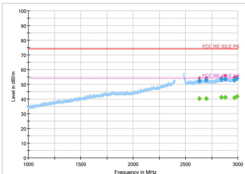
Fig.140 Radiated Spurious Emission (802.11 n-20Mhz,Ch12,1GHz~3GHz)
