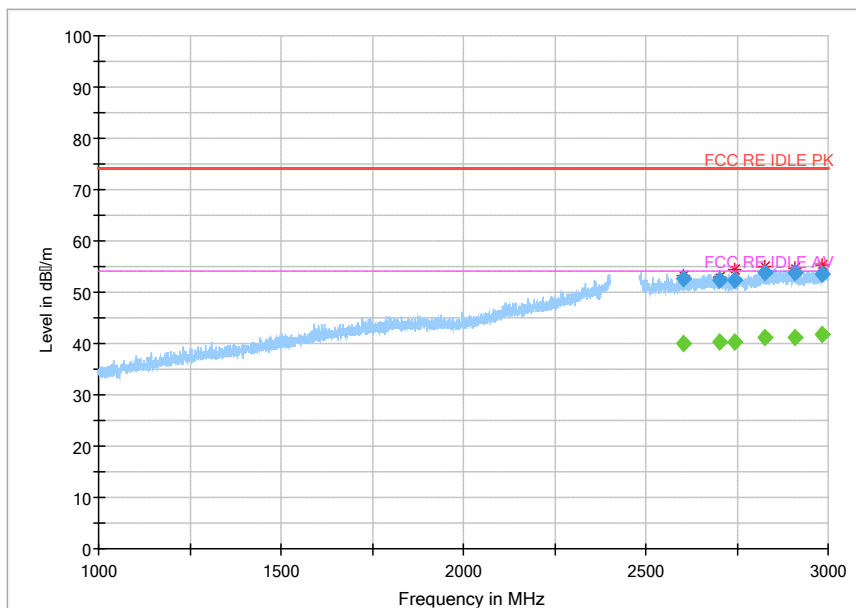
Fig.130 Radiated Spurious Emission (802.11g, Ch12, 1GHz~3GHz)
