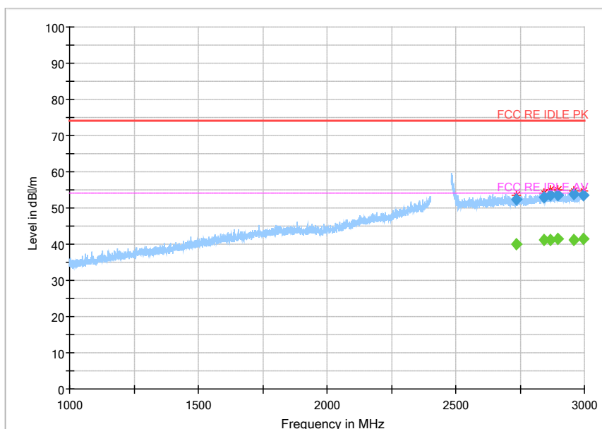
Fig.145 Radiated Spurious Emission (802.11 n-20Mhz,Ch13,1GHz~3GHz)
