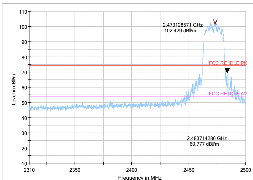
Fig.133 Radiated emission (Power): 802.11g,Ch13
