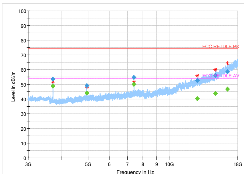
Fig.126 Radiated Spurious Emission (802.11b, Ch13, 3GHz~18GHz)
