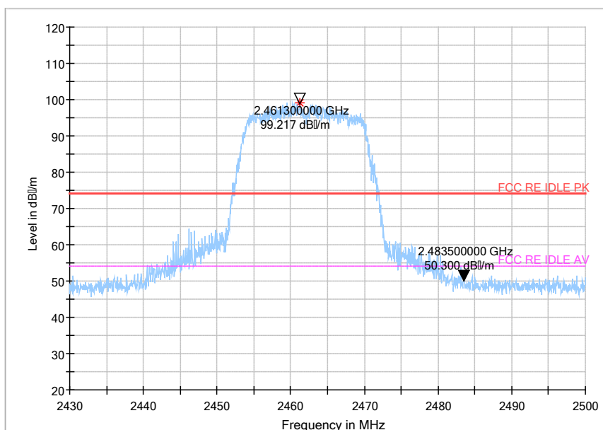
Fig.103 Radiated emission (Power): 802.11g, high channel
