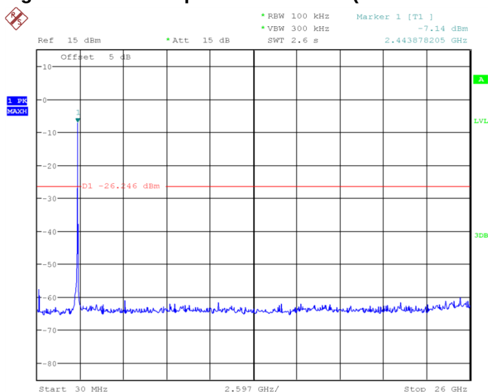
Fig.95 Conducted Spurious Emission (802.11n-40MHz, Ch11)
