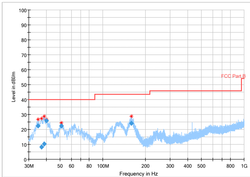
Fig.149 Radiated Spurious Emission (802.11 n-40Mhz,Ch10,30MHz~1GHz)
