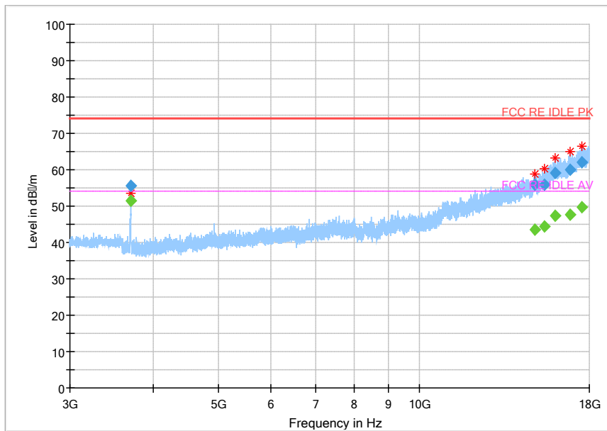
Fig.121 Radiated Spurious Emission (802.11b, Ch12, 3GHz~18GHz)
