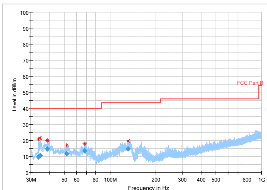
Fig.153 Radiated Spurious Emission (802.11 n-40Mhz,Ch11,30MHz~1GHz)
