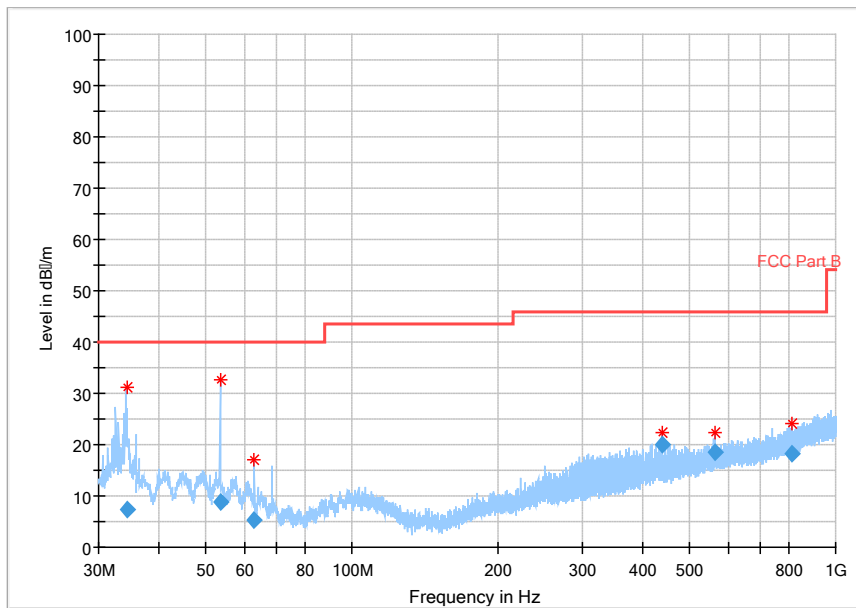
Fig.129 Radiated Spurious Emission (802.11g, Ch12, 30MHz~1GHz)
