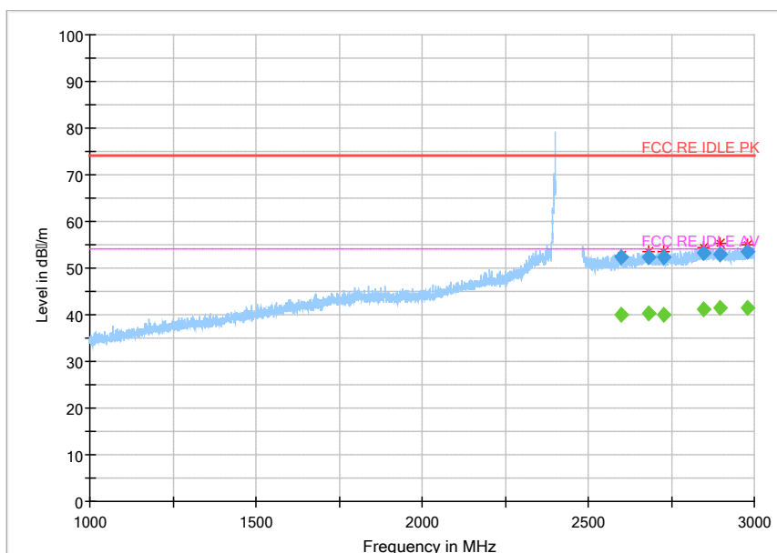
Fig.105 Radiated Spurious Emission (802.11g,Ch1,1GHz~3GHz)
