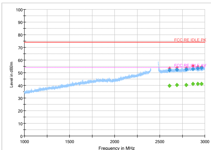
Fig.135 Radiated Spurious Emission (802.11g, Ch13, 1GHz~3GHz)
