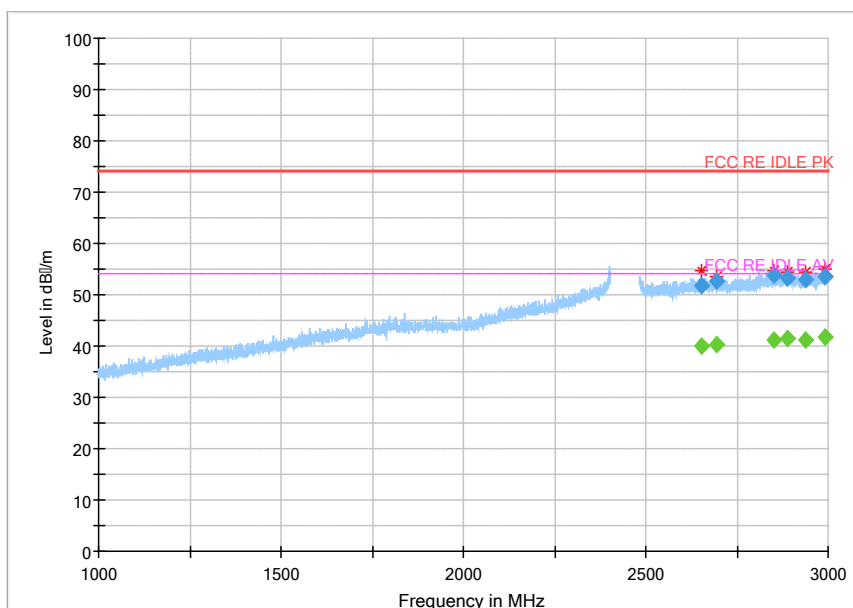
Fig.115 Radiated Spurious Emission (802.11 n-40MHz,Ch3,1GHz~3GHz)
