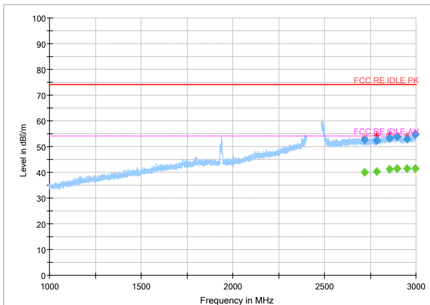
Fig.150 Radiated Spurious Emission (802.11 n-40Mhz,Ch10,1GHz~3GHz)
