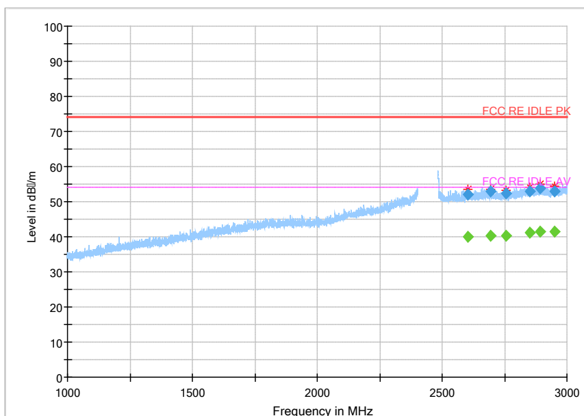
Fig.125 Radiated Spurious Emission (802.11b, Ch13, 1GHz~3GHz)
