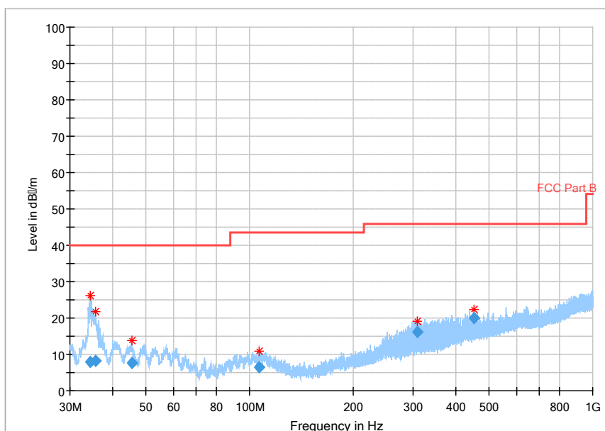
Fig.99 Radiated Spurious Emission (802.11b,Ch1,30MHz~1GHz)
