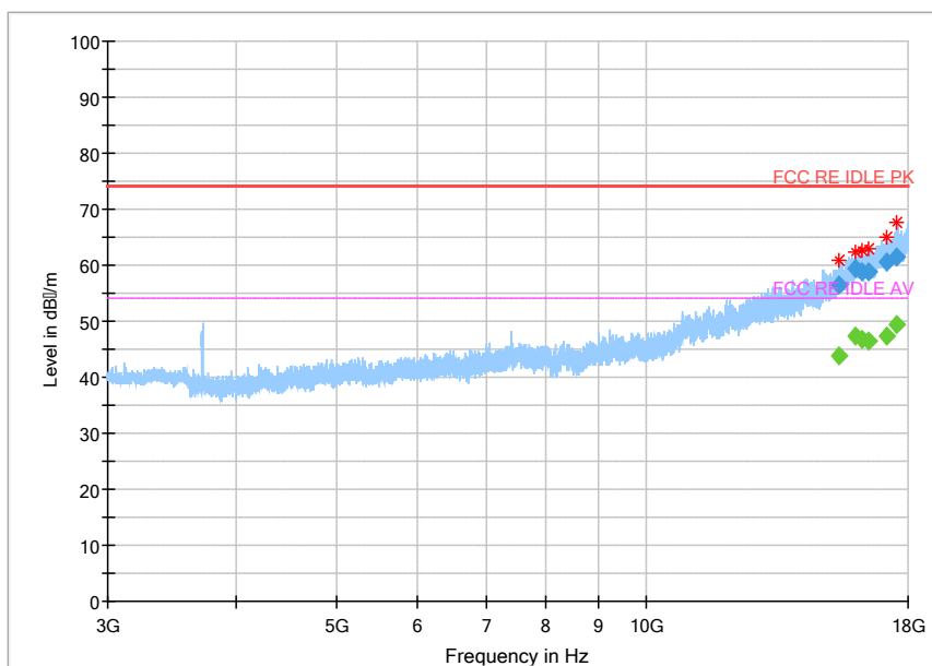
Fig.146 Radiated Spurious Emission (802.11 n-20Mhz,Ch13,3GHz~18GHz)
