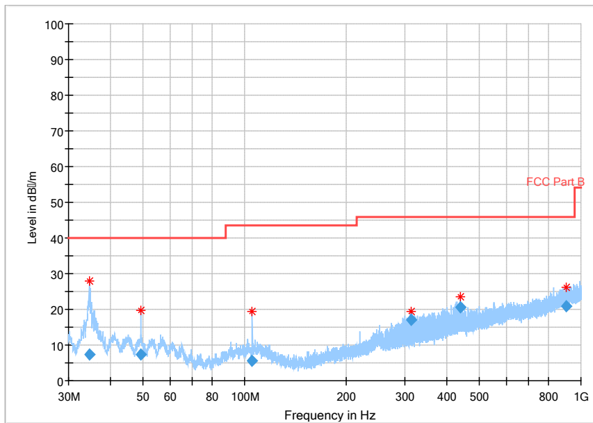
Fig.109 Radiated Spurious Emission (802.11 n-20MHz,Ch1,30MHz~1GHz)
