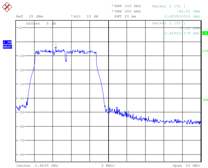
Fig.51 Band Edges (802.11b-20MHz, Ch12)
