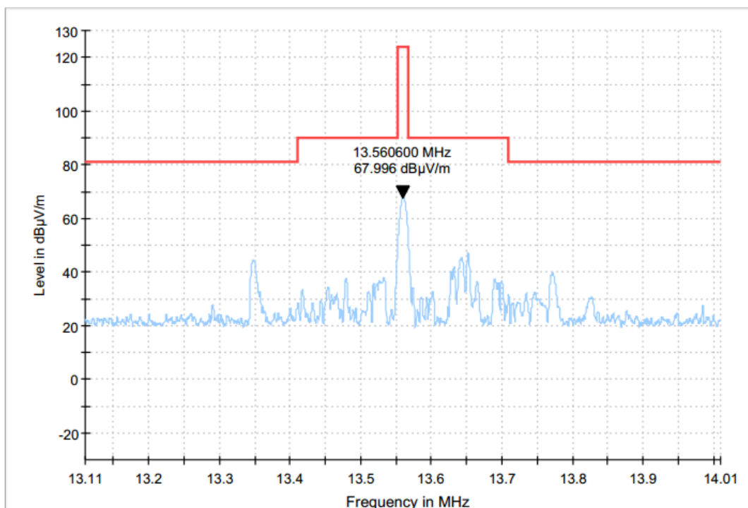
Figure 1 TX mode
