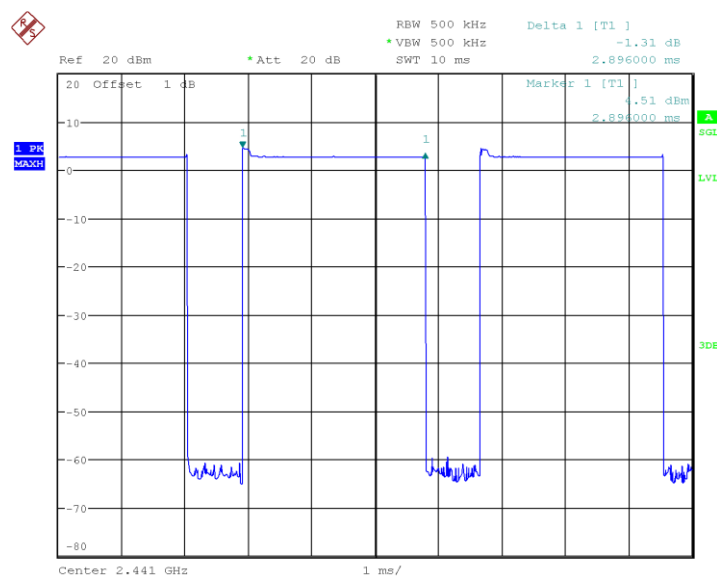
Fig.70 Number of Transmissions Measurement: Ch39, Packet 3-DH3
