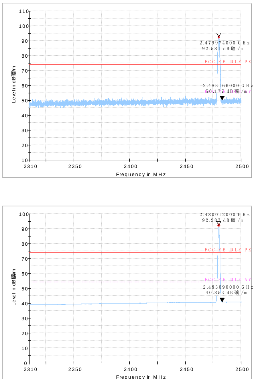
Fig.44 Radiated emission (High): GFSK, high channel
