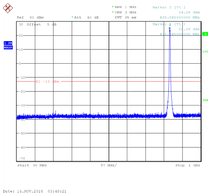
Fig.69 Channel 4183: 30MHz~1GHz
