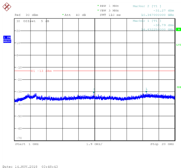
Fig.70 Channel 4183: 1GHz~20GHz
