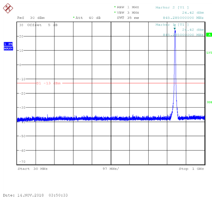
Fig.71 Channel 4233: 30MHz~1GHz
