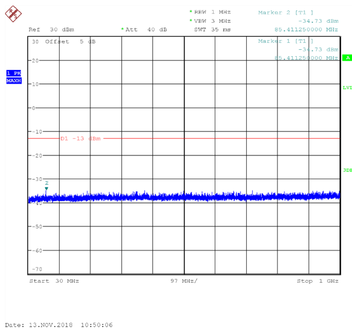
Fig.49 Channel 128: 30MHz~1GHz
