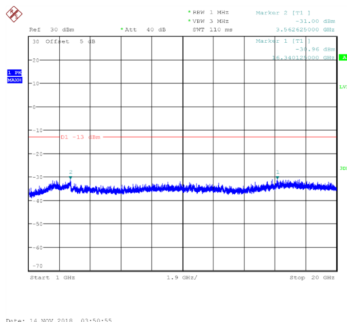
Fig.72 Channel 4233: 1GHz~20GHz
