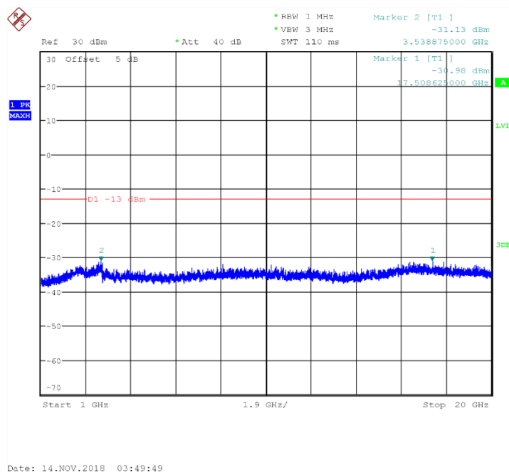
Fig.68 Channel 4132: 1GHz~20GHz
