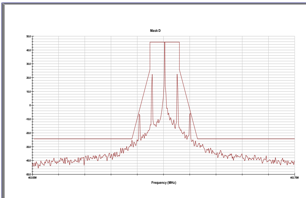
Emission Mask D Plot 463.7 MHz
