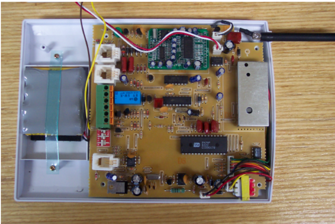
<Internal photo>
