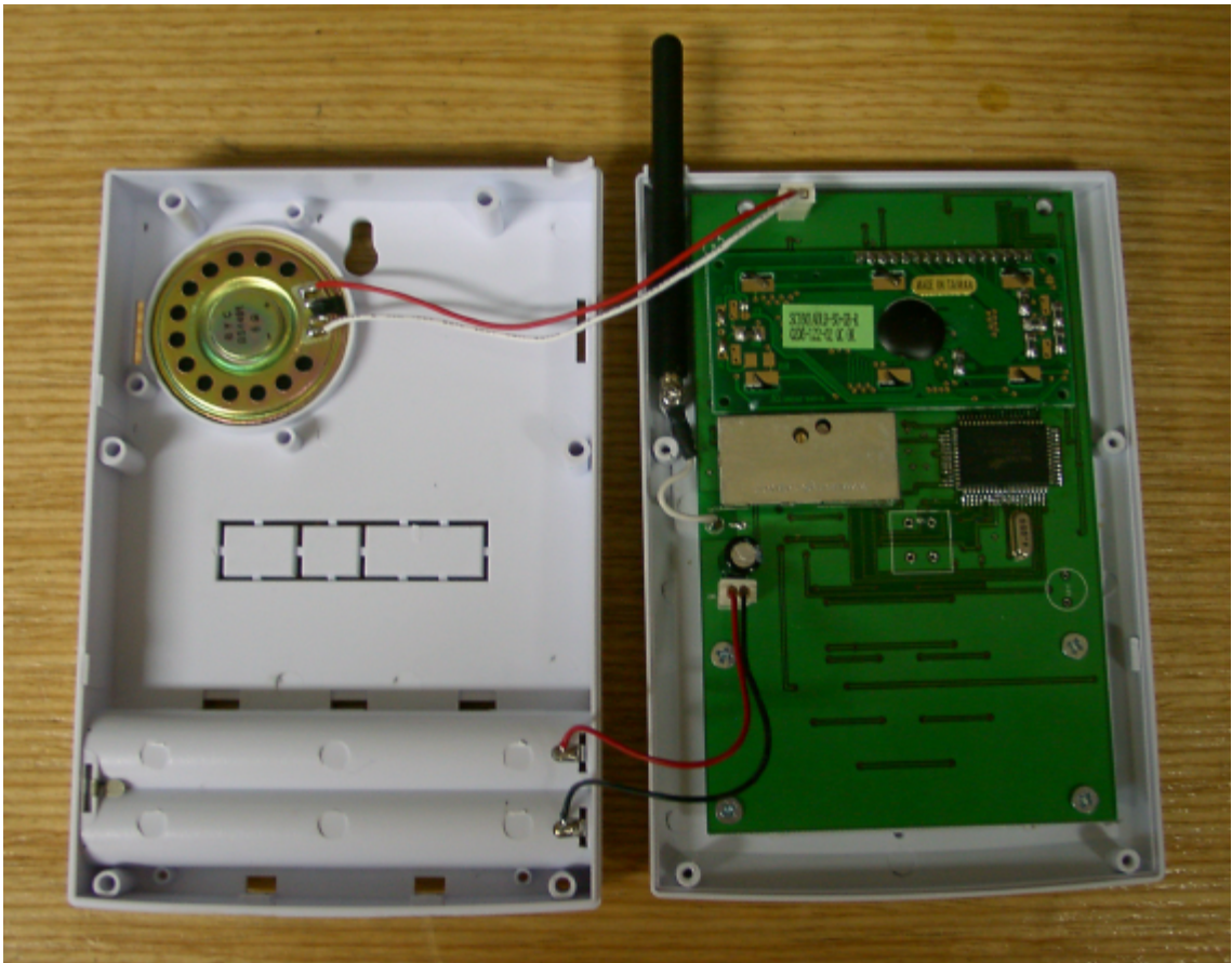
< Inside view – Overall >
