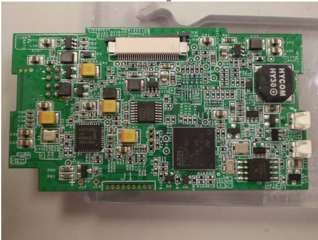
Main PCB_Front
