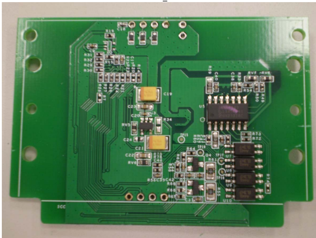
ICC PCB_Front
