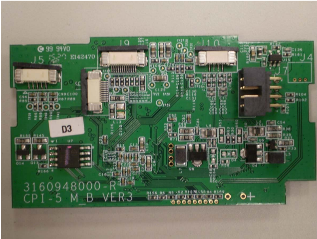
Main PCB_Back
