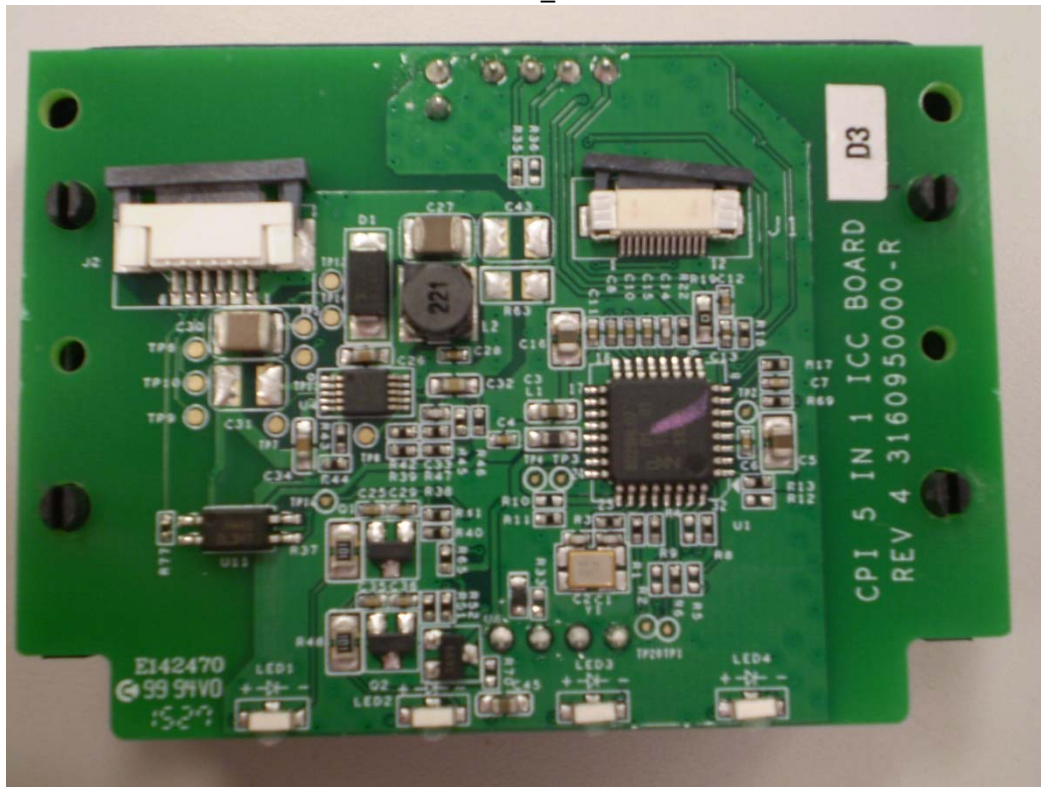
ICC PCB_Back
