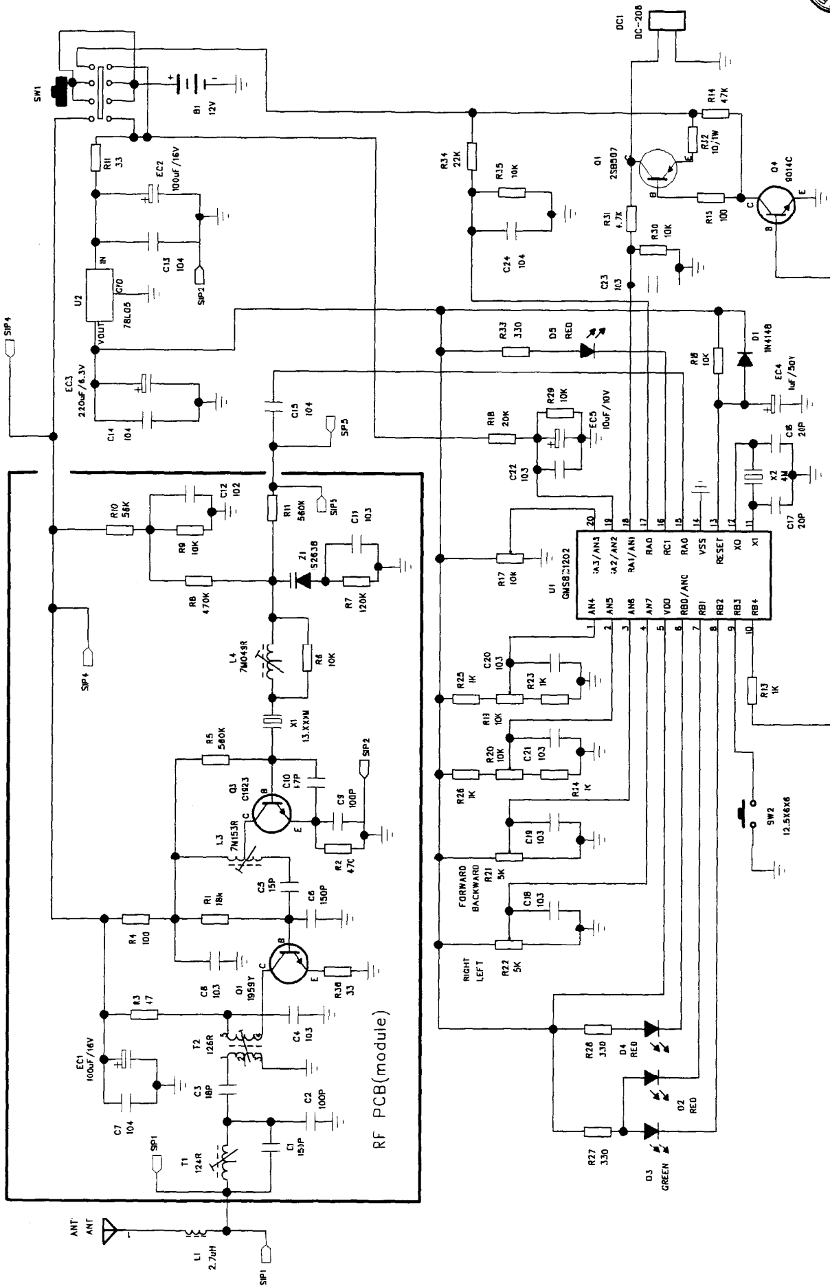
CPU PCB
