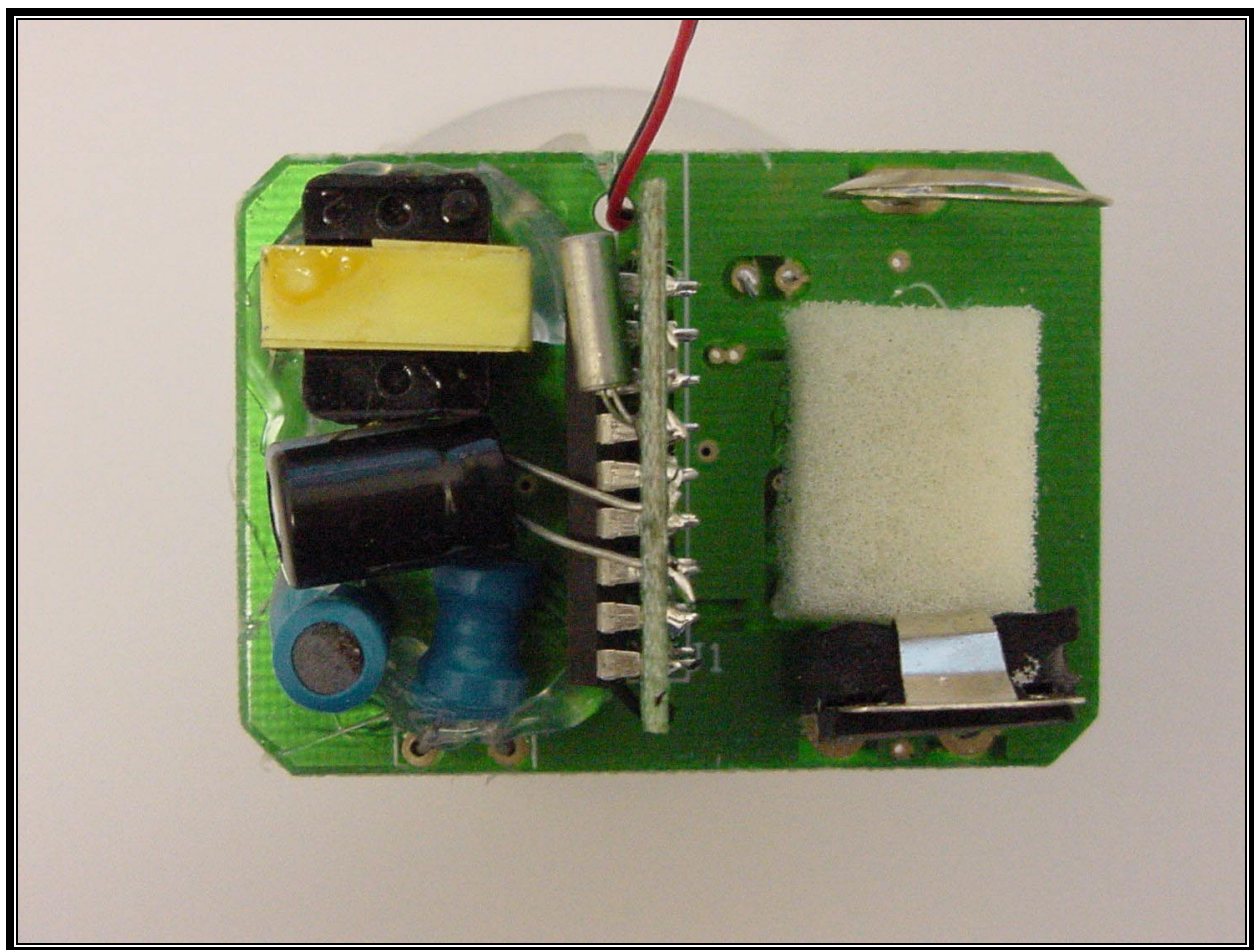
PHOTOGRAPH 24: RECEIVER PCB – TOP VIEW
