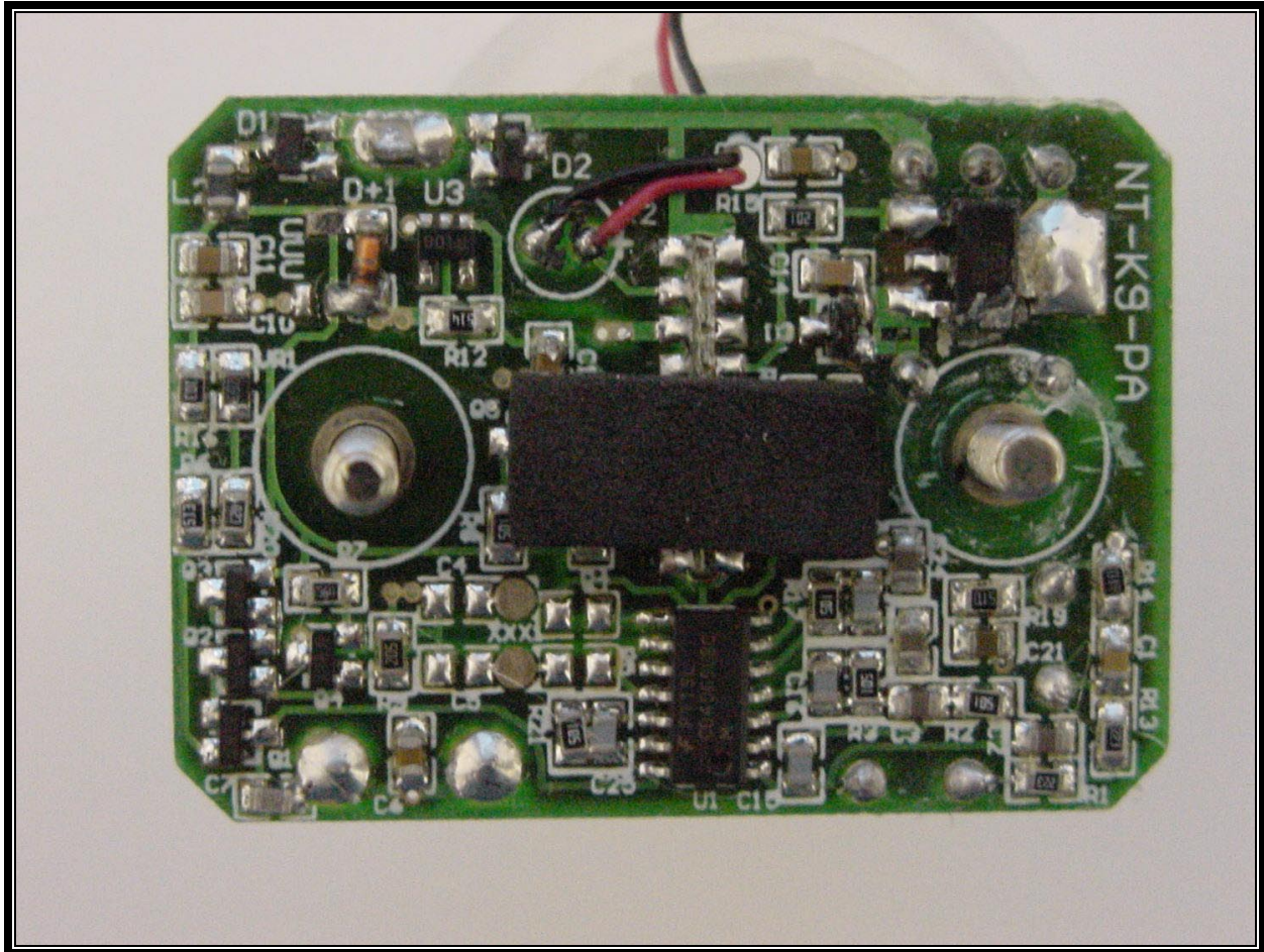
PHOTOGRAPH 25: RECEIVER PCB – BOTTOM VIEW
