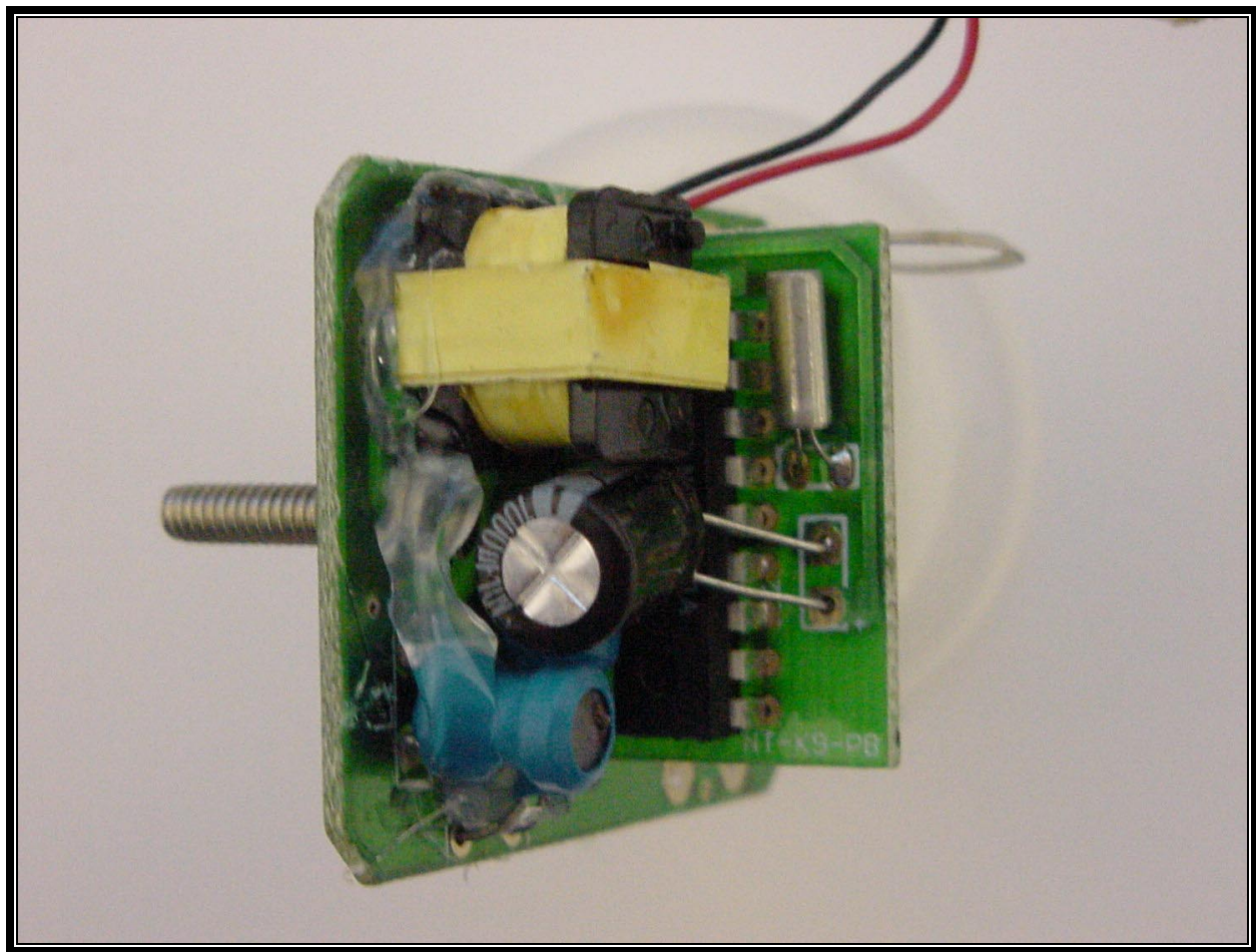
PHOTOGRAPH 26: RECEIVER PCB – SIDE VIEW
