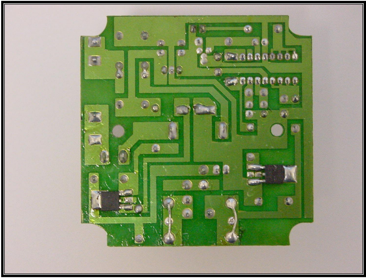
PHOTOGRAPH 23: TRANSMITTER PCB – SOLDER SIDE
