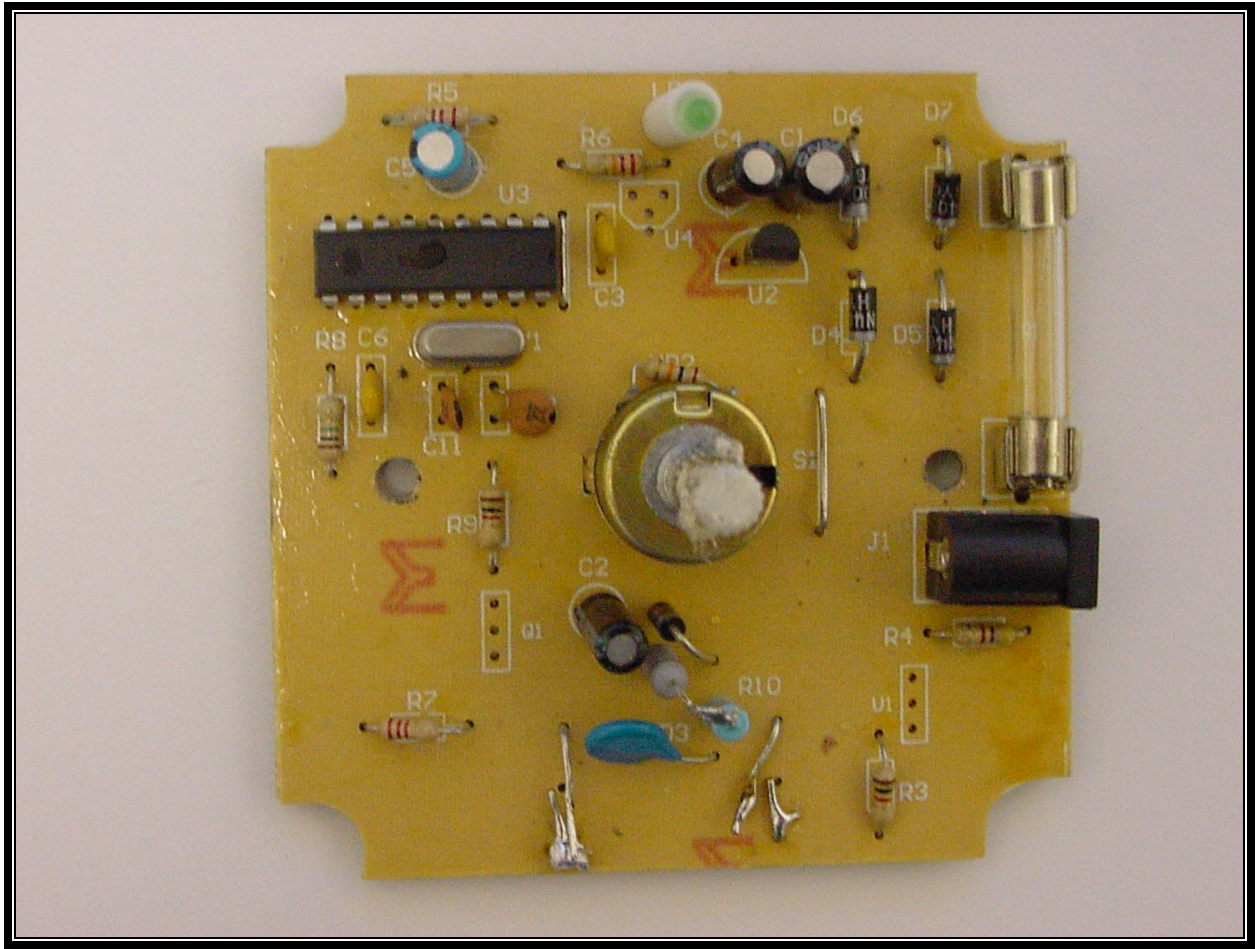
PHOTOGRAPH 22: TRANSMITTER PCB – COMPONENT SIDE
