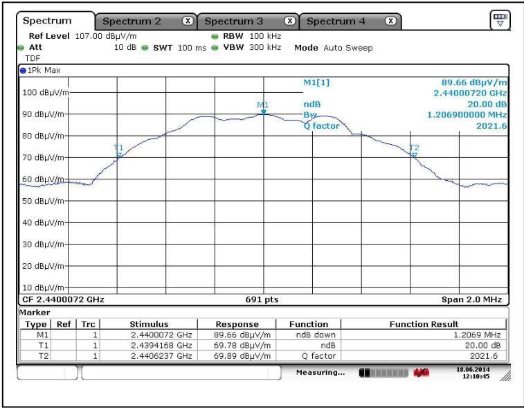
Bandwidth 2 (2440MHz)
