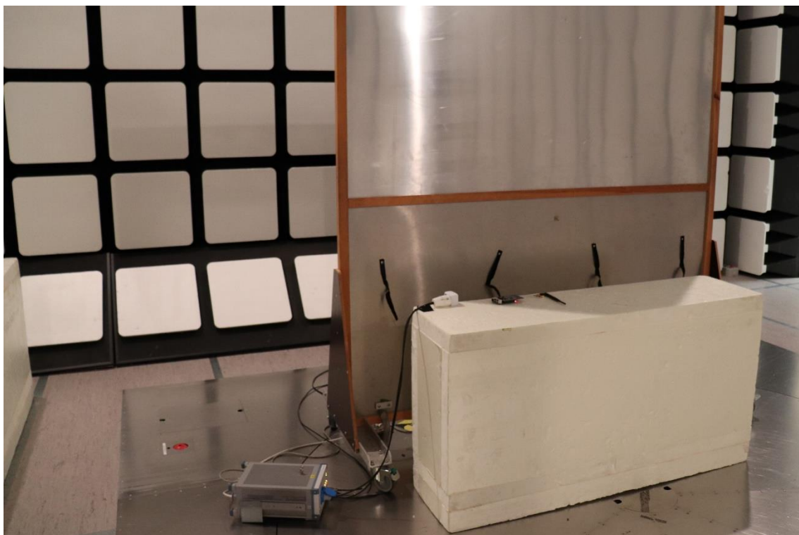
Photograph 11. Conducted Emissions
