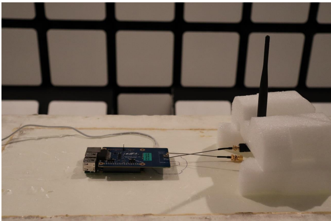
Photograph 10. EUT position during radiated tests
