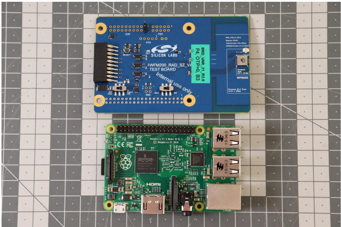
Photograph 3. EUT 2, (Raspberry Pi was used during tests)
