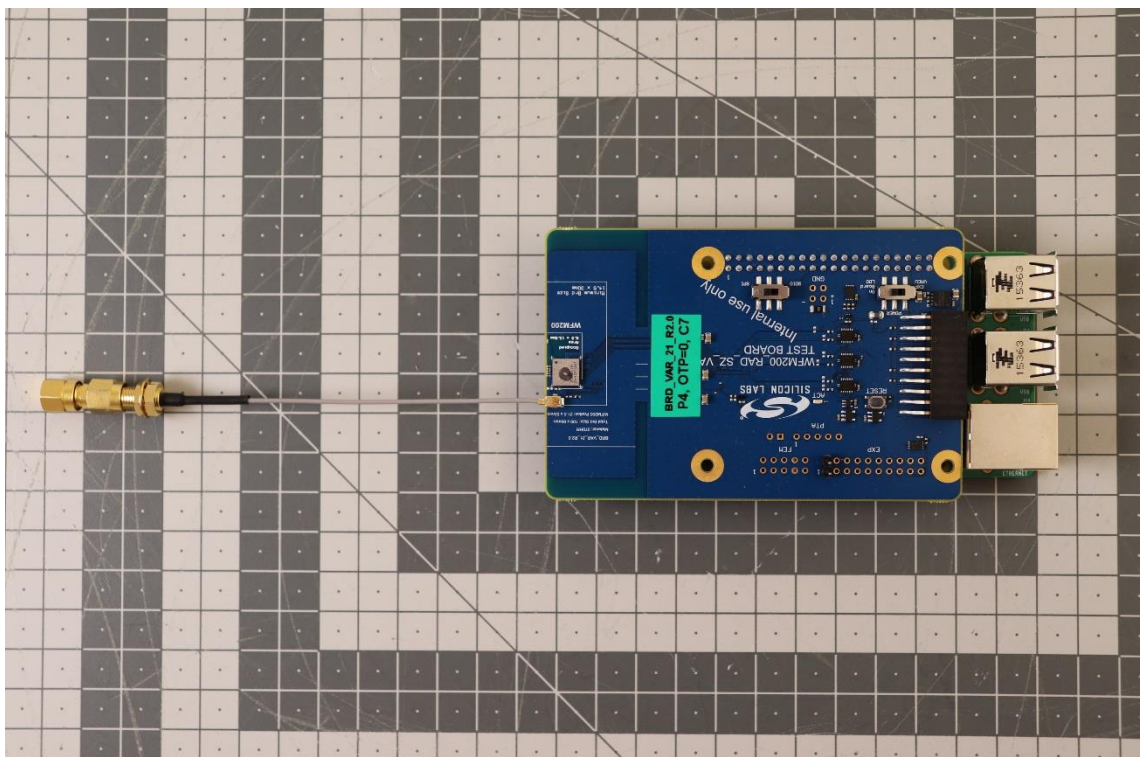
Photograph 4. EUT 1, C7 (internal antenna)
