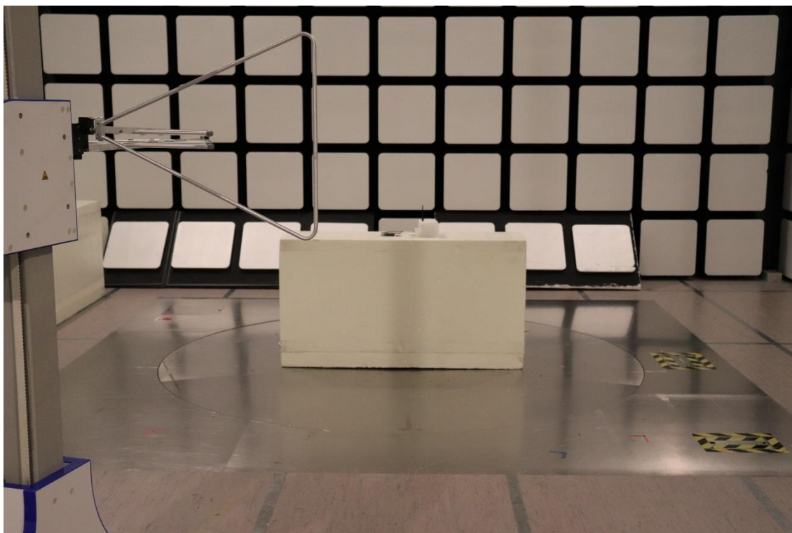
Photograph 7. Radiated Spurious Emissions 30 MHz – 1000 MHz
