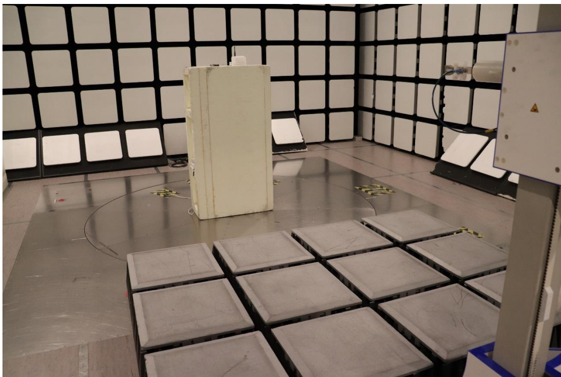
Photograph 9. Radiated Spurious Emissions 18 GHz – 26.5 GHz
