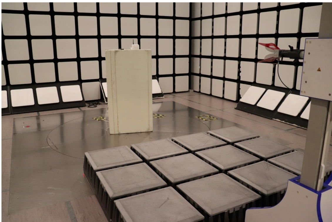
Photograph 8. Radiated Spurious Emissions 1 GHz – 18 GHz
