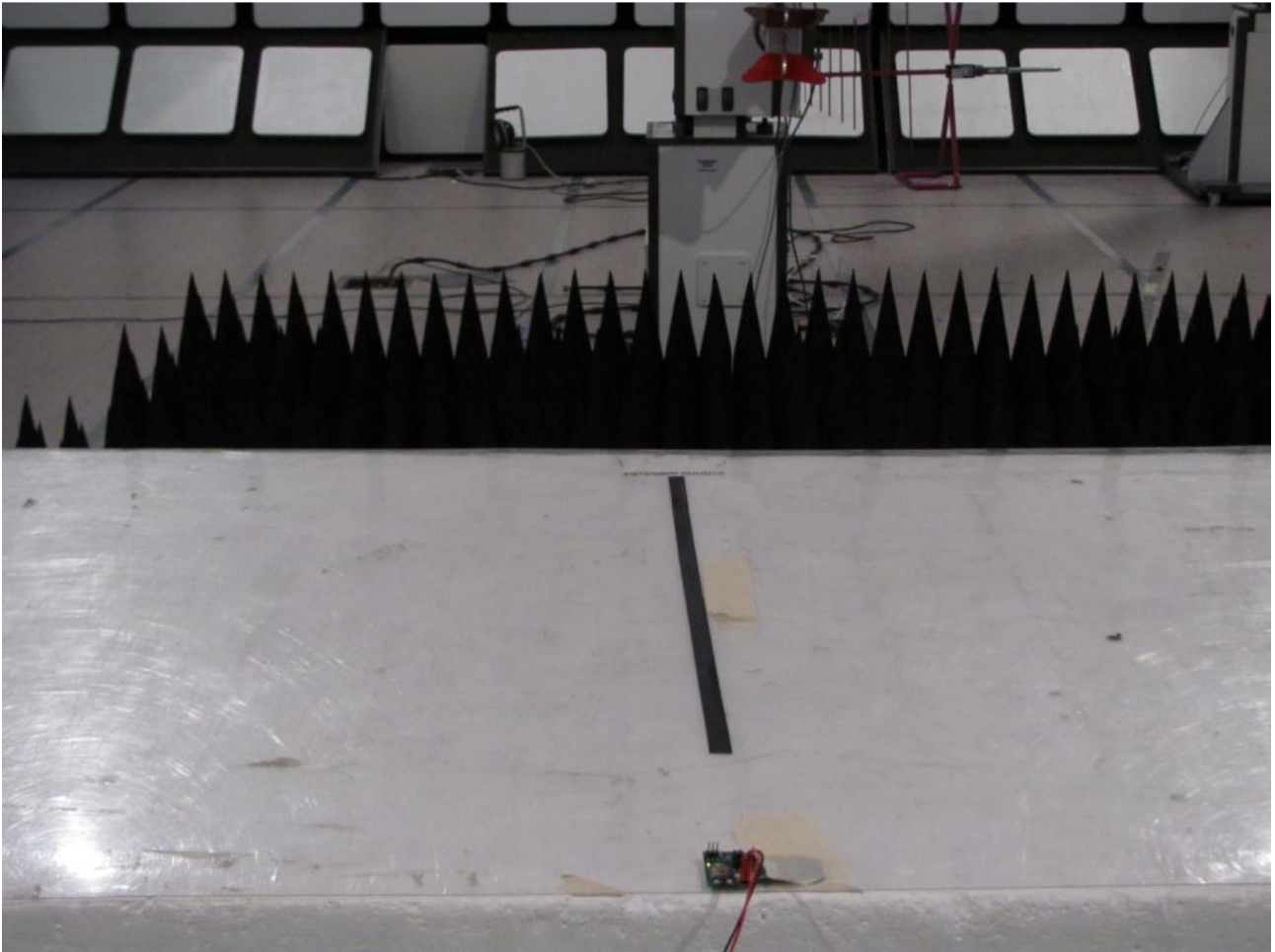
Radiated emission test setup model WF111-A
