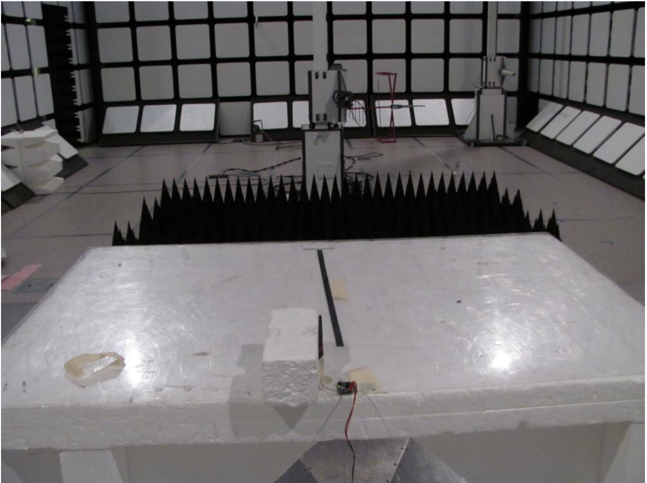
Radiated emissions test setup model WF111-E
