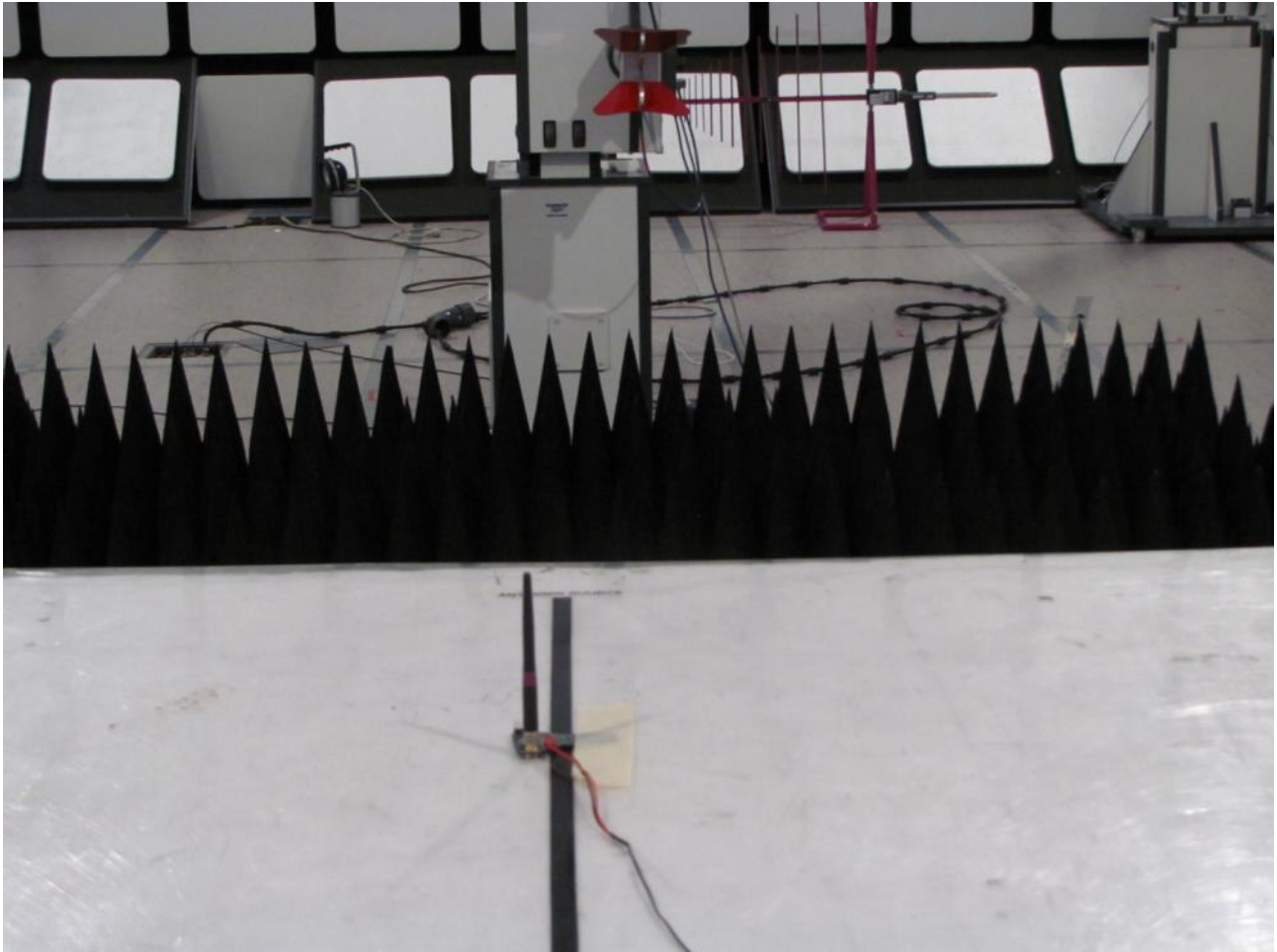
Radiated emissions test setup model WF111-N
