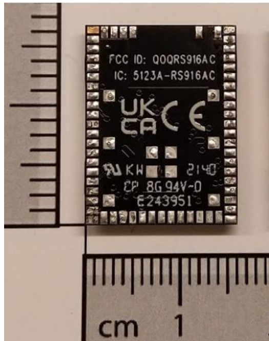
Back view of Model RS916AC1
