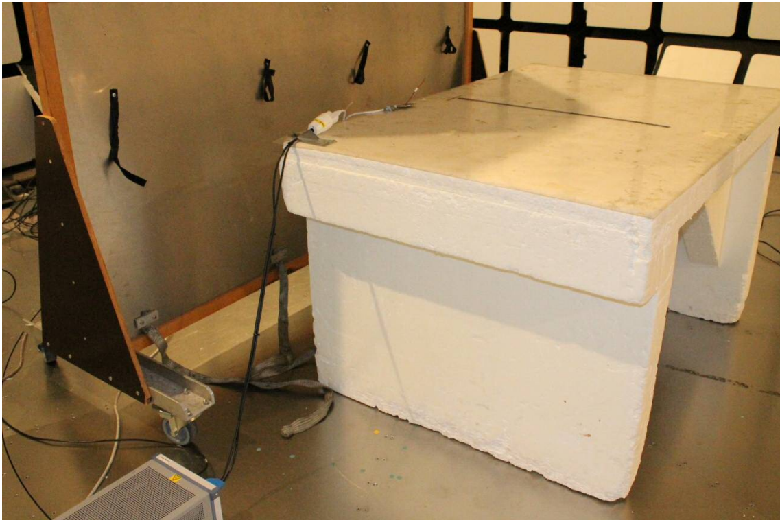
Photograph 5. Conducted Emissions
