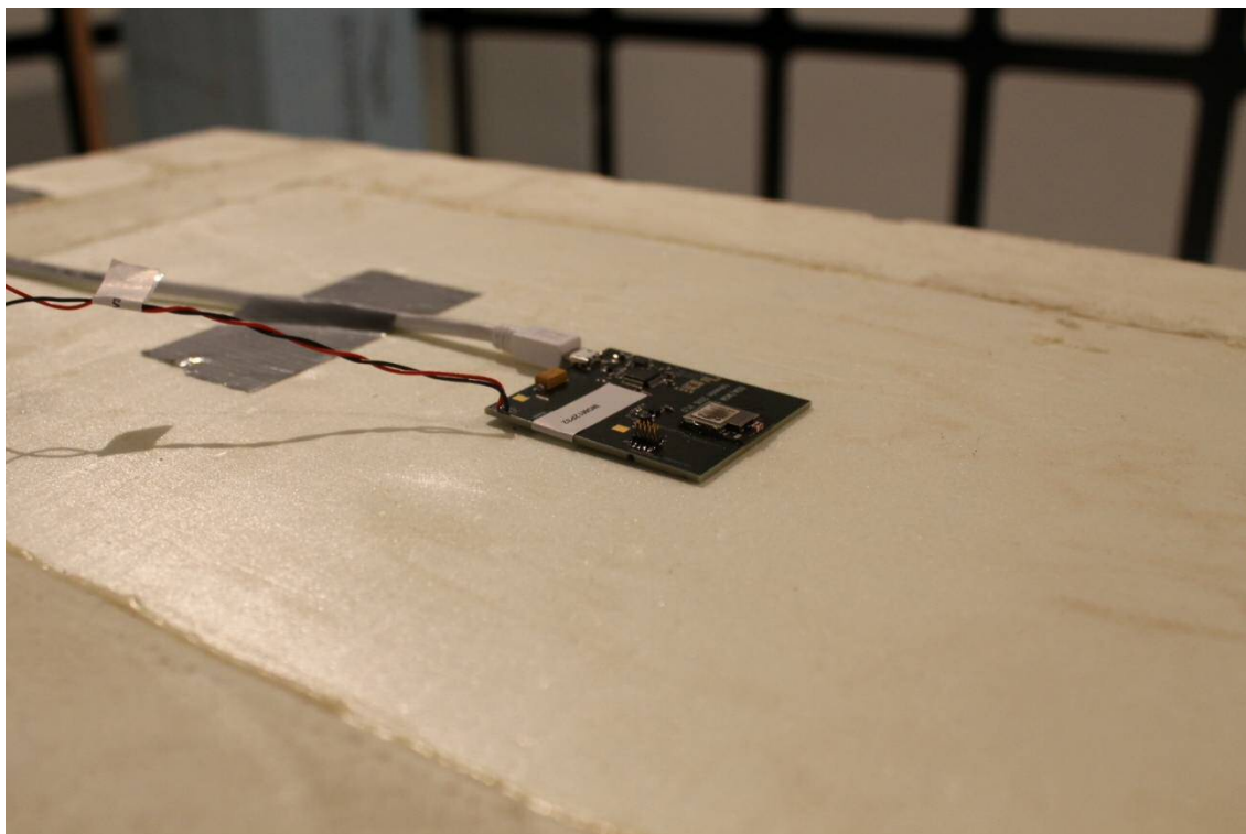
Photograph 4. EUT on table
