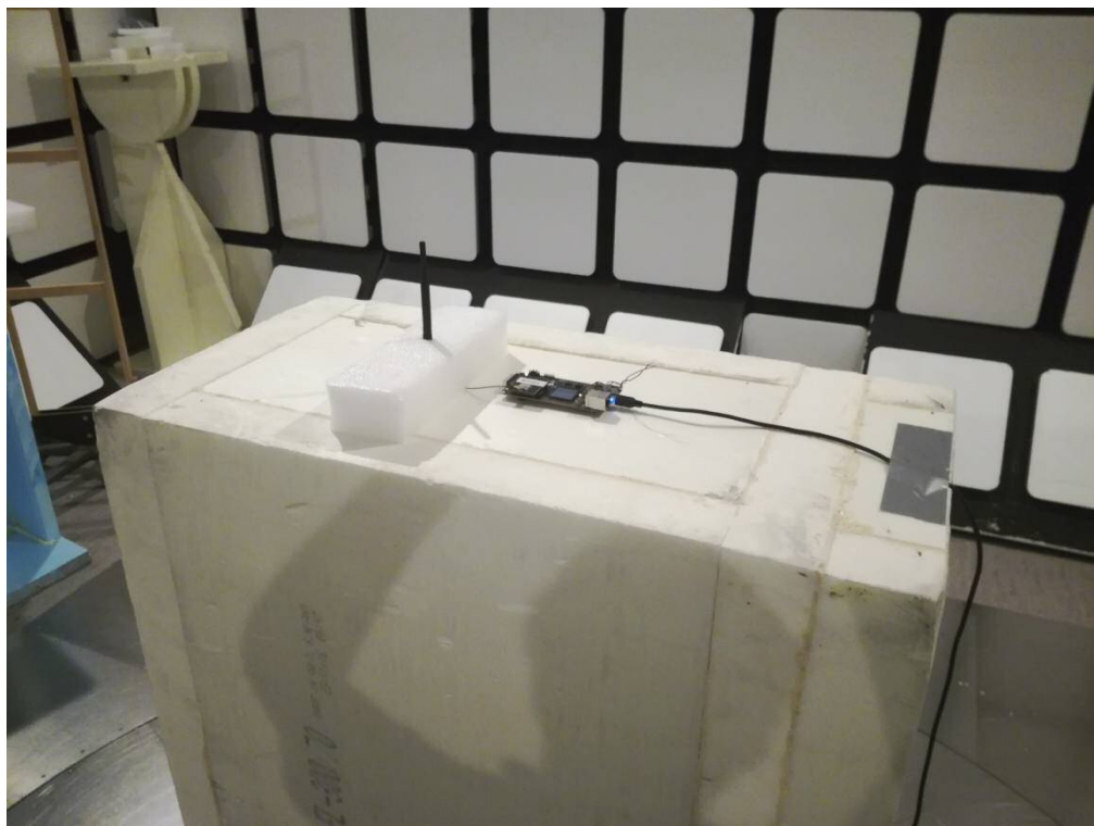
Photograph 6. The EUT on table (E-variant)
