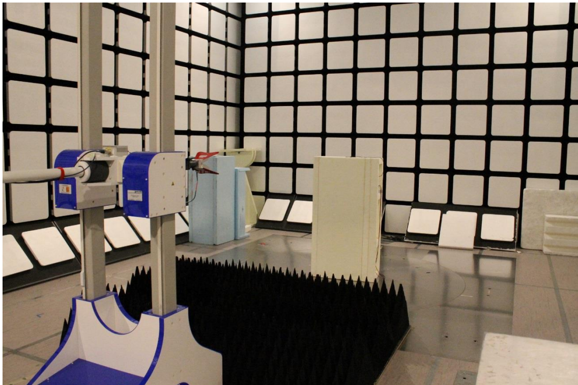
Photograph 2. Radiated Spurious Emissions 1 – 18 GHz
