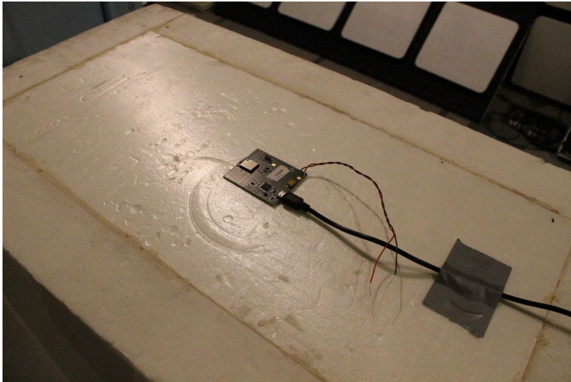
Photograph 5. EUT on table (integral chip antenna)
