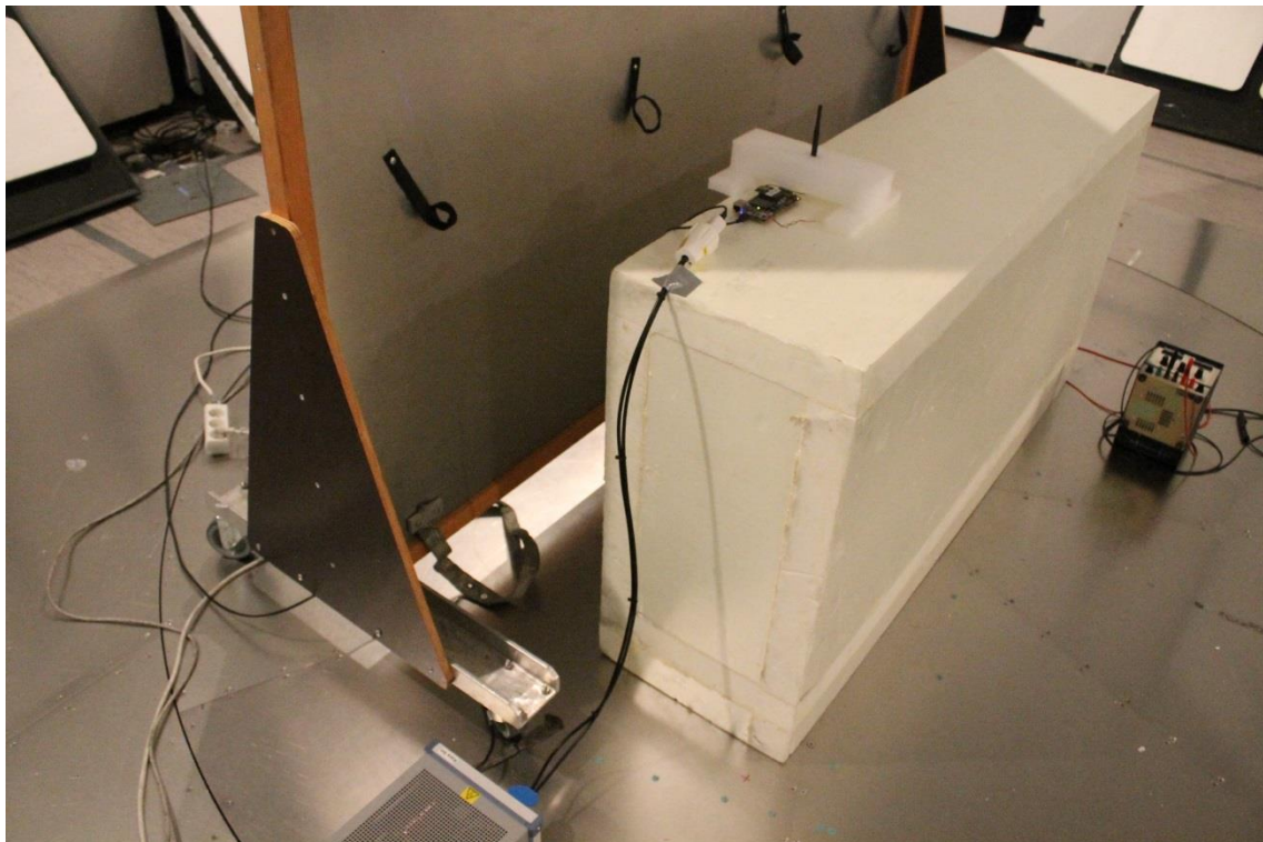
Photograph 6. Conducted Emissions
