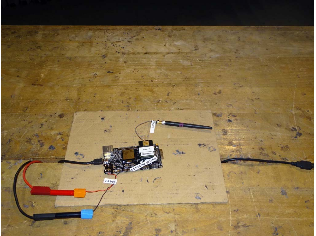
Photo 2: Test setup for radiated measurements below 1 GHz, detailed view
