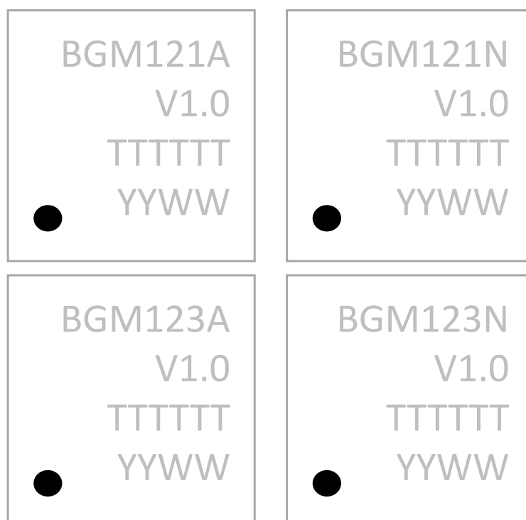
Figure 1: Label of BGM121A, BGM121N, BGM123A and BGM123N
