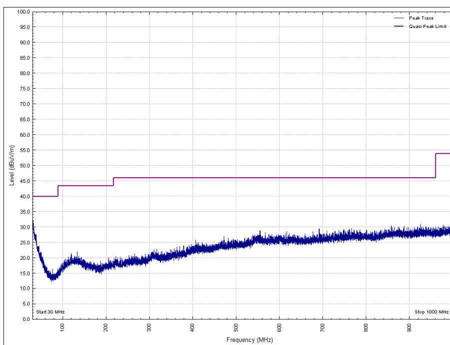
Figure 57 - 30 MHz to 1 GHz, 2440 MHz, Horizontal, EUT Orientation X
