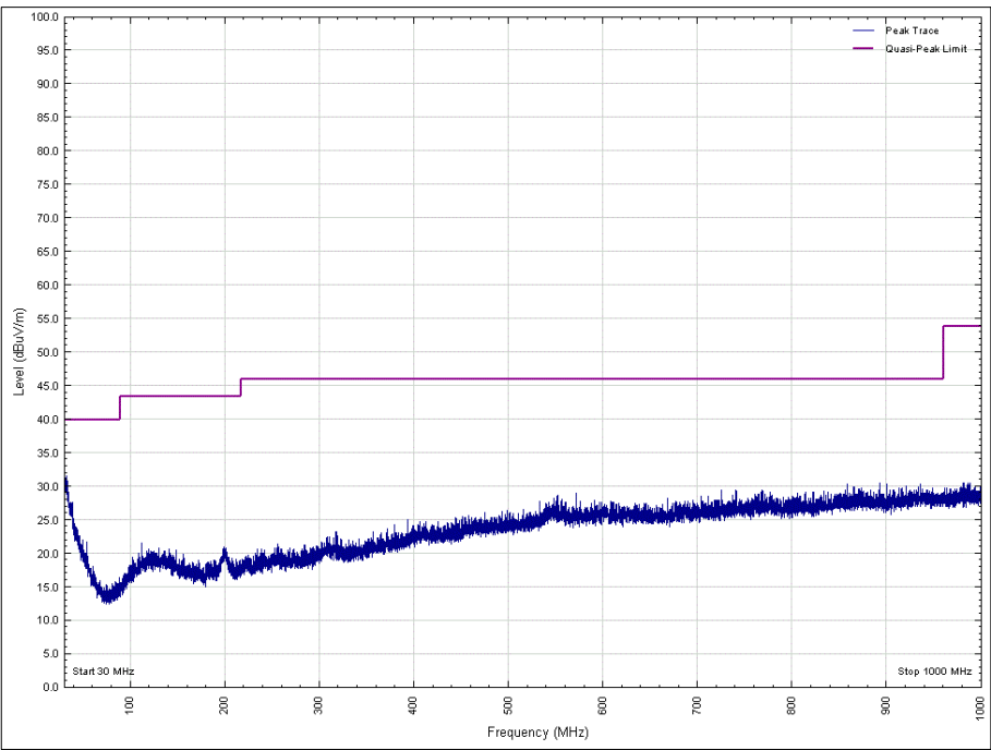
Figure 102 - 30 MHz to 1 GHz, 2402 MHz, Vertical, EUT Orientation X
