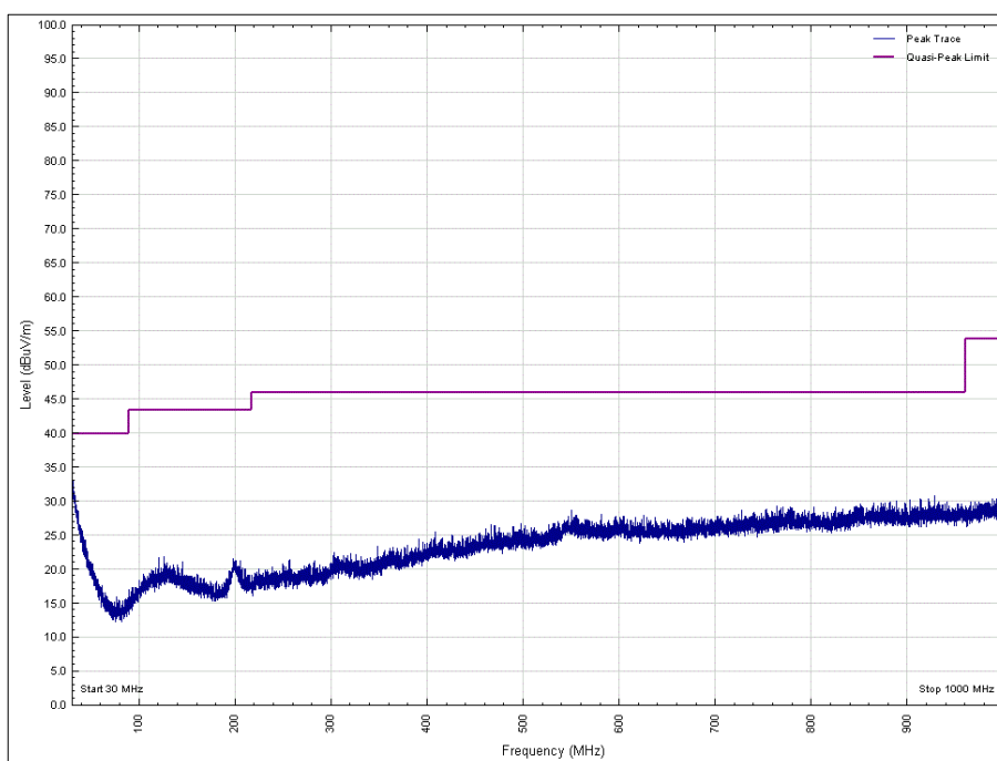
Figure 56 - 30 MHz to 1 GHz, 2440 MHz, Vertical, EUT Orientation X
