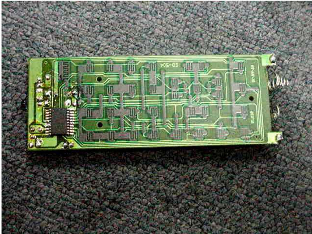
Soldering side of the board
