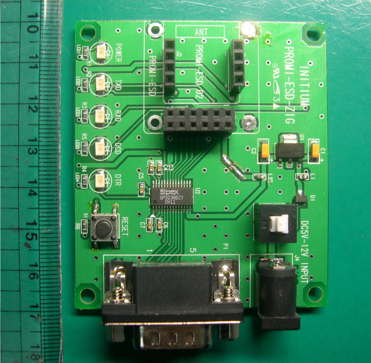
<Photograph 2: TEST JIG, Model Promi-DBS Front View>
