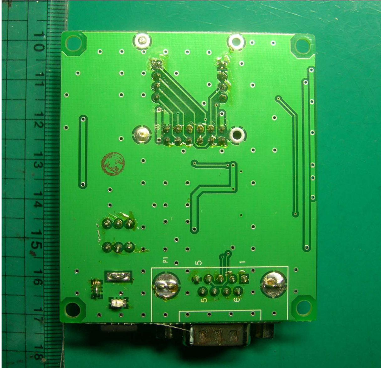
<Photograph 3: TEST JIG, Model Promi-DBS Rear View>
