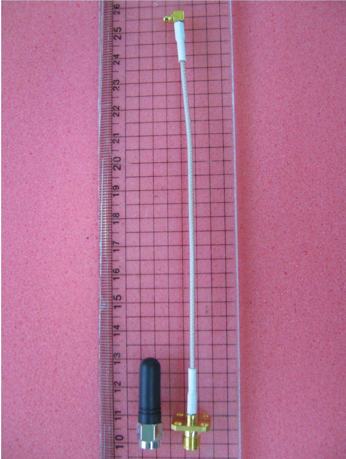
<Photograph 3: Antenna and Cable >
