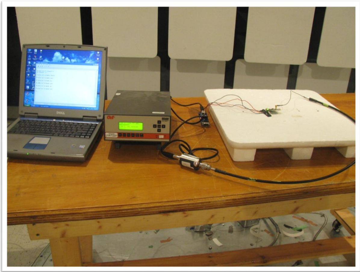
Figure 2 – Conducted RF power measurements
