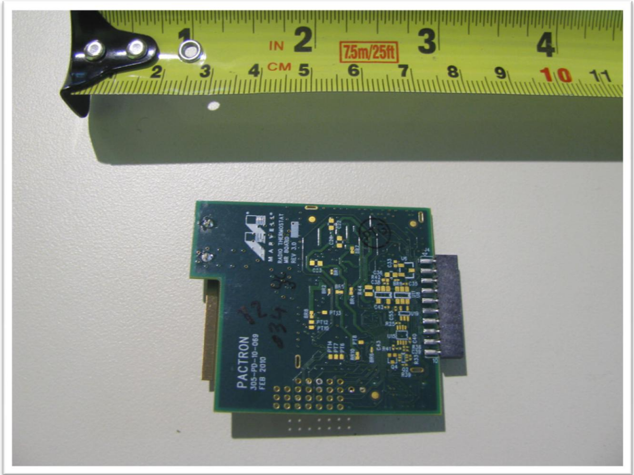
Figure 2 – EUT rear
