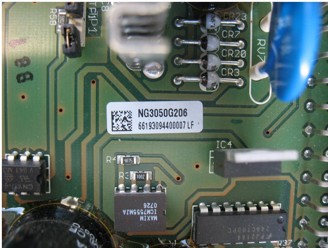
Photo No. 11: pulse modulator, type label
