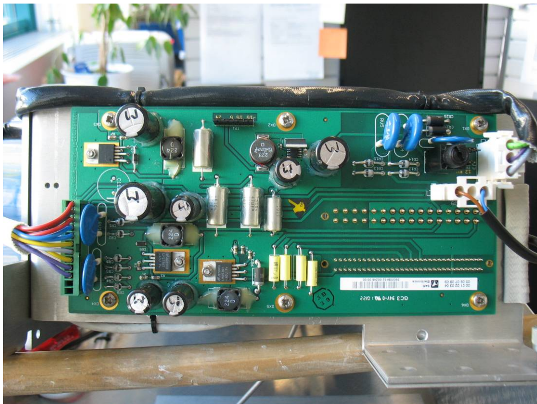
Photo No. 4: PSU board
