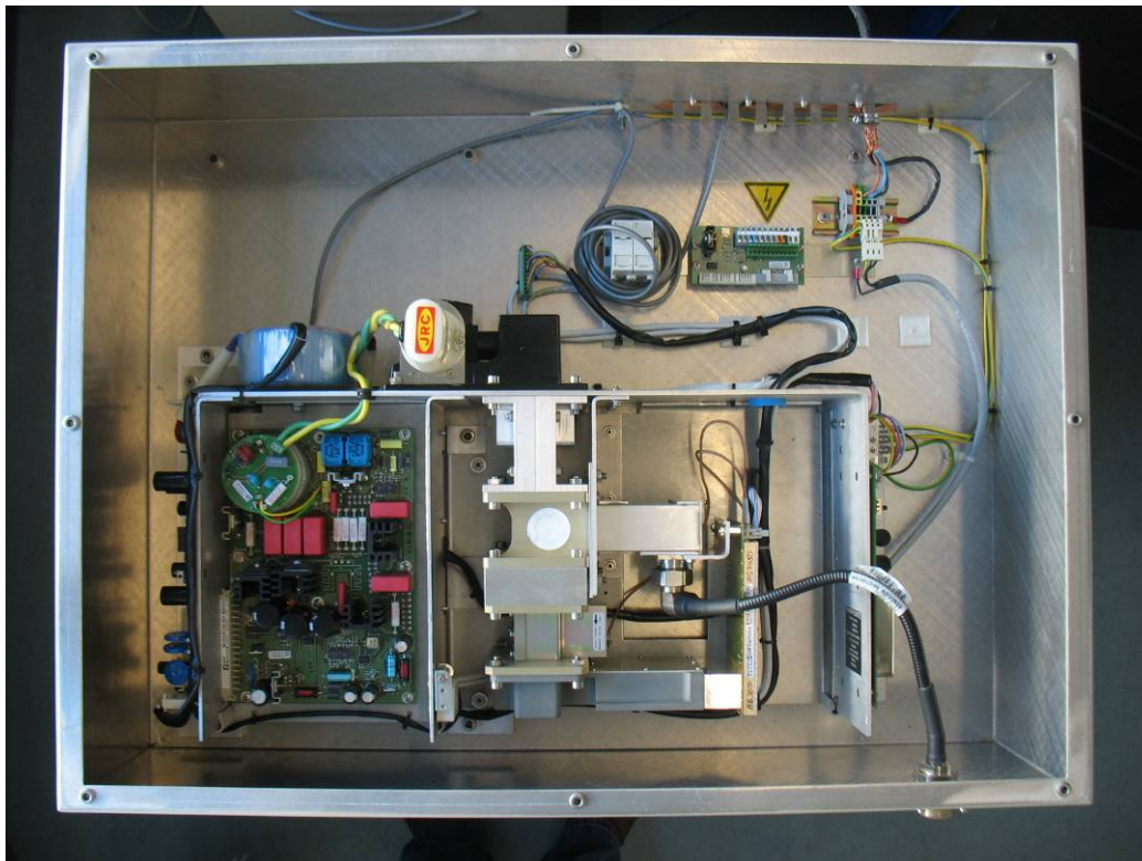
Photo No. 2: 30 kW Magnetron
