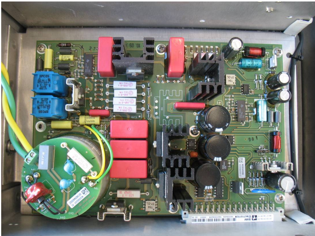
Photo No. 10: pulse modulator
