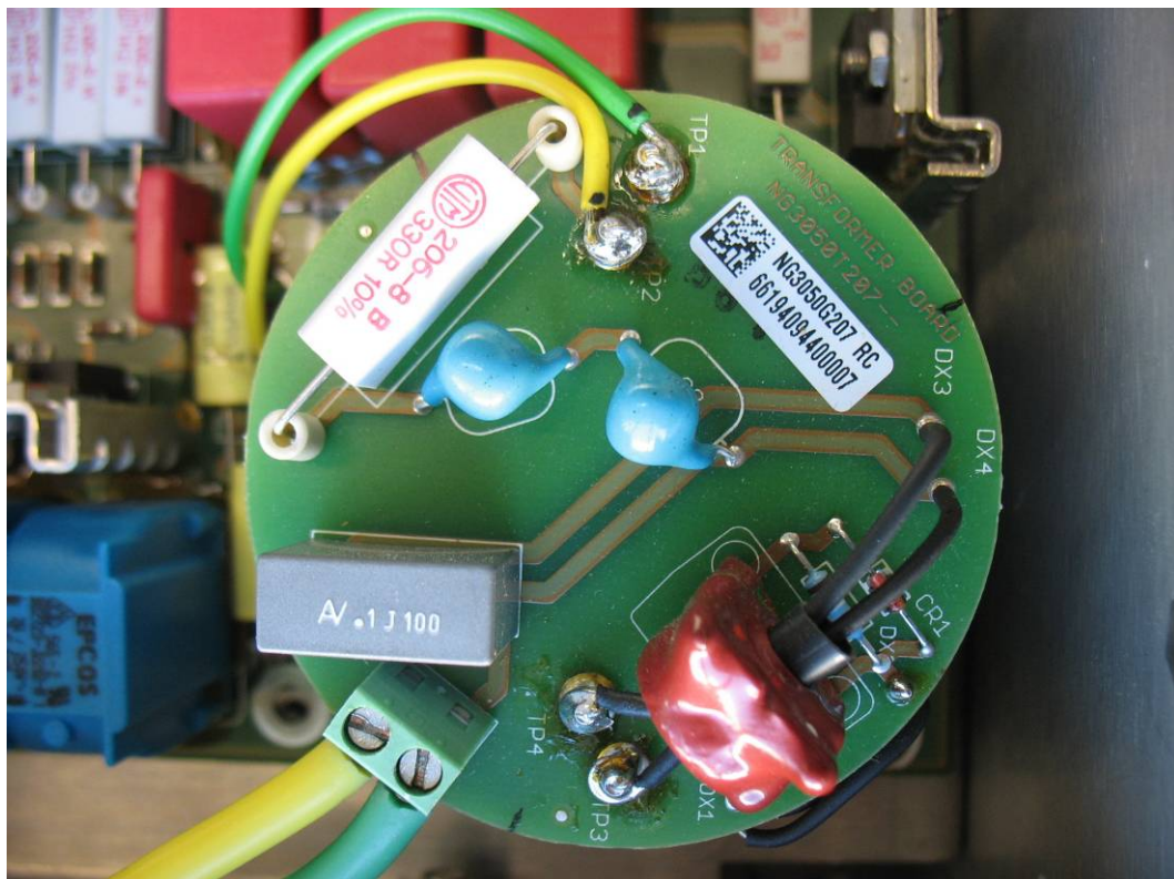
Photo No. 12: HV transformer
