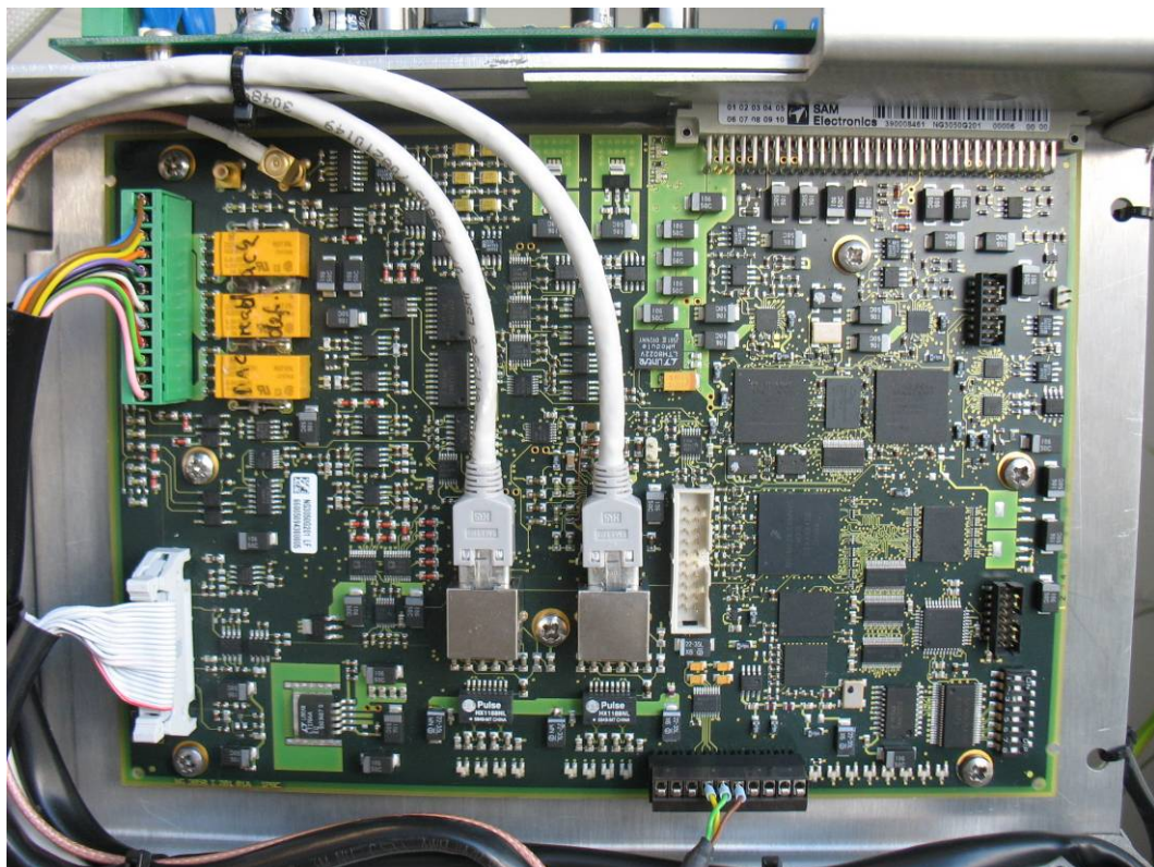
Photo No. 6: IP RADAR Controller (IPRC)
