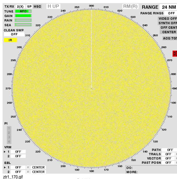
Fig. 4-37 Check RSC Adjust (Gain 100% and GAIN 0%)
