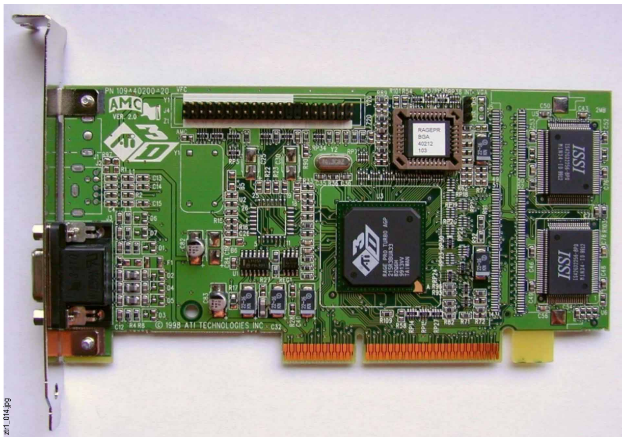
Fig. 4-41 GVP pcb
