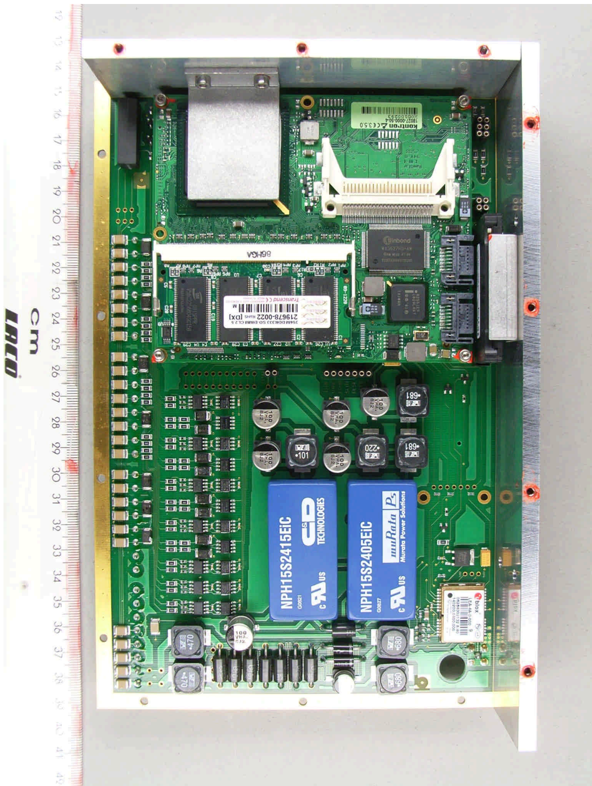
92475eut15.jpg: Main-Power and Computer-PCB, front-view
