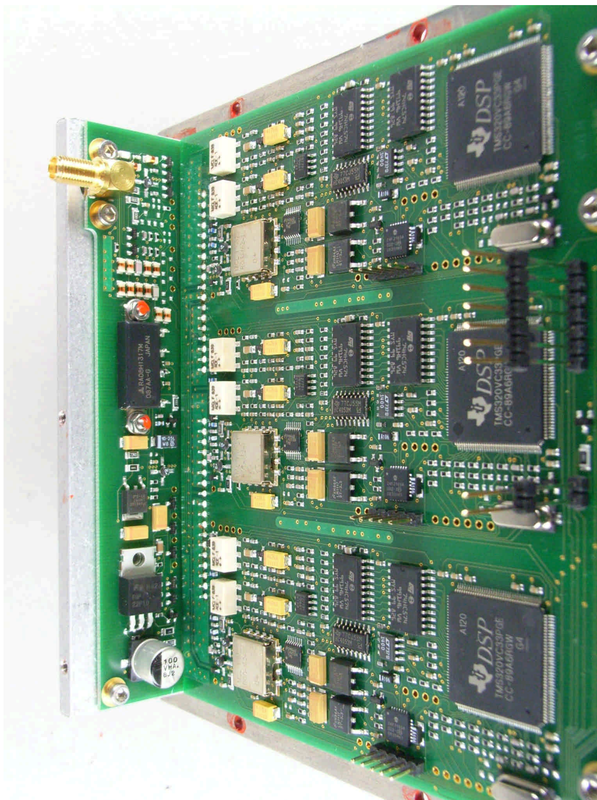
91972pcb7.jpg: Complete RF-PCB
