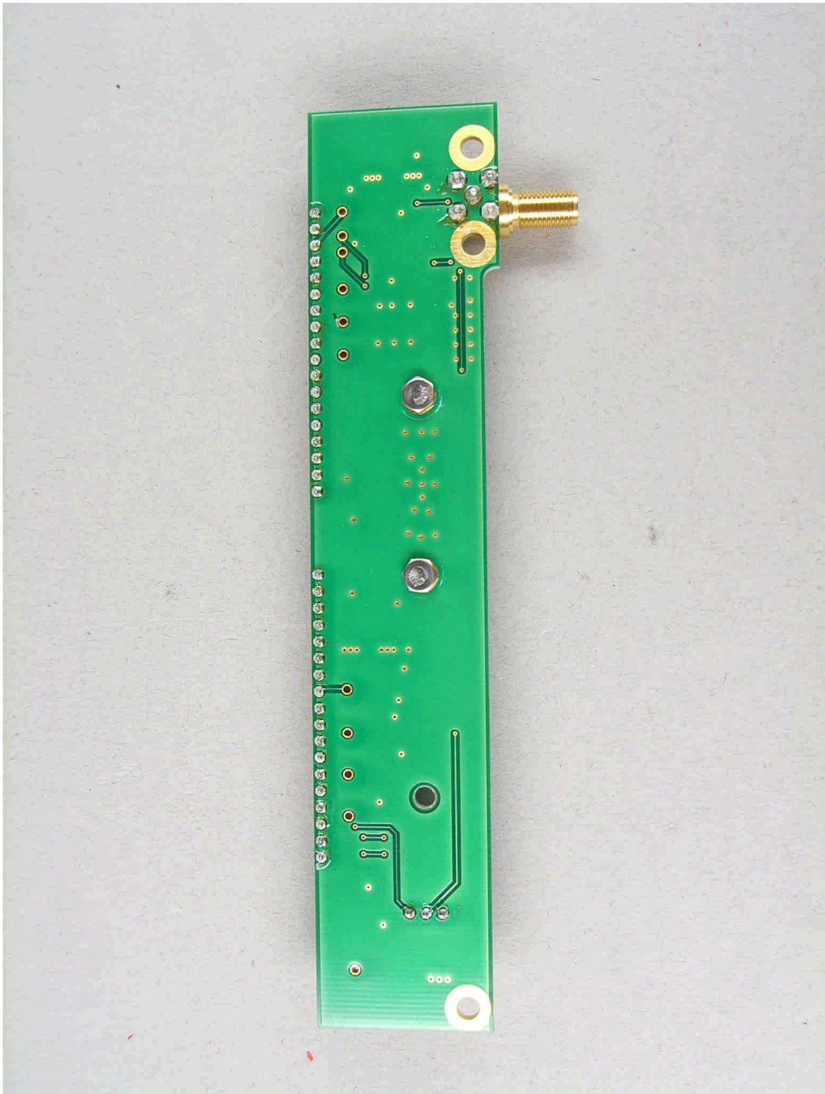
92475eut23.jpg: Antenna-Part, rear-view
