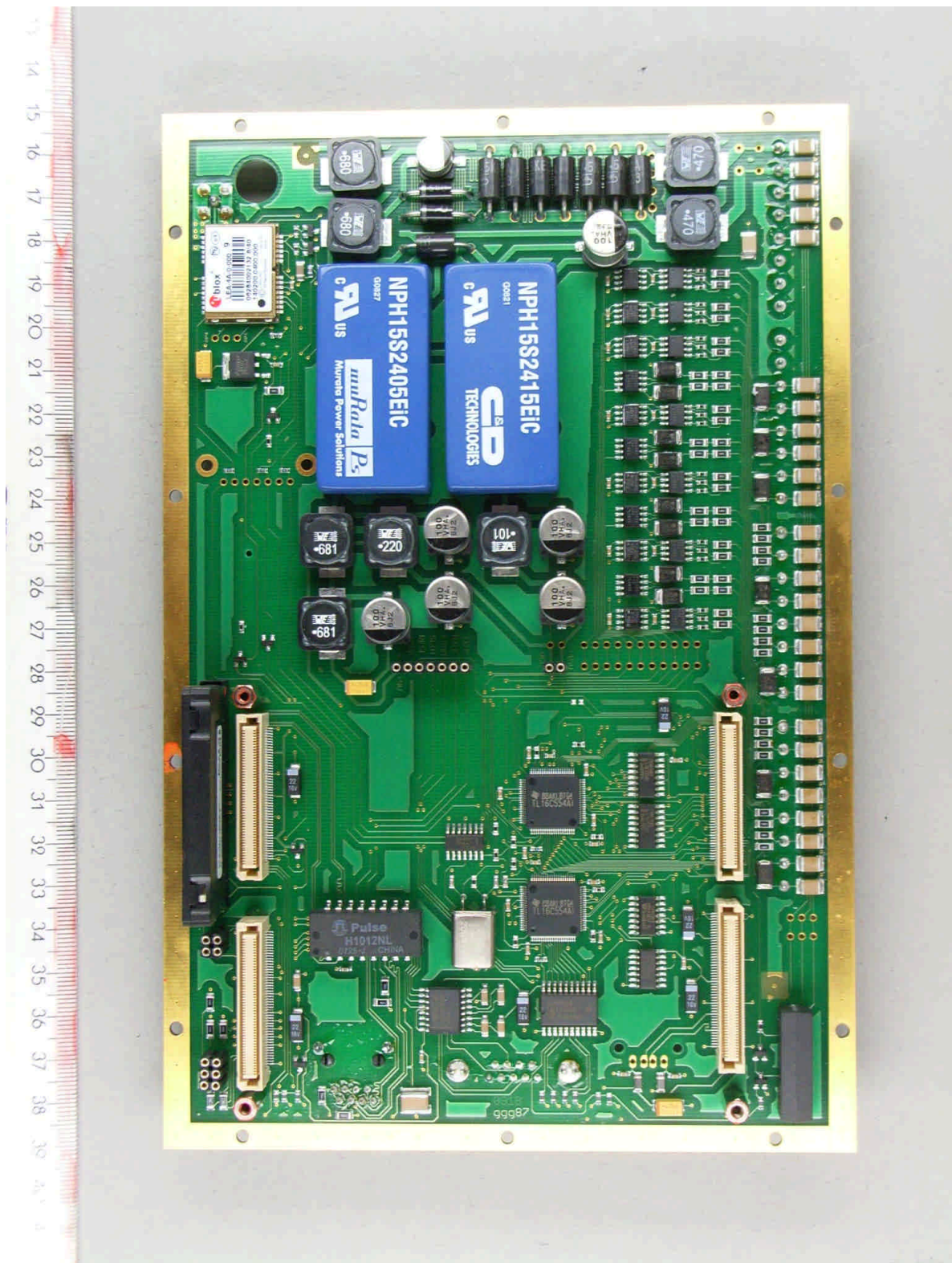
92475eut19.jpg: Main-Power and Computer-PCB, front-view (without PC)
