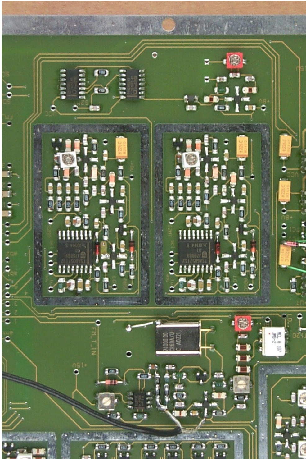
20273eut15.jpg: DEBEG 3400, radio part, PCB, baseband-unit
