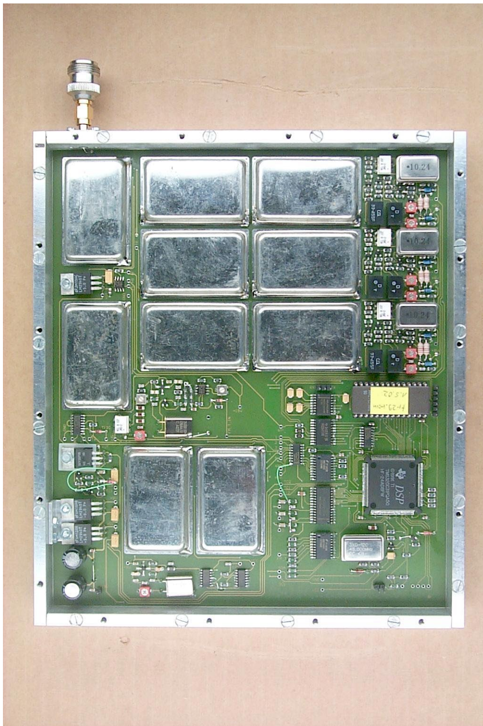
20273eut8.jpg: DEBEG 3400, radio part, PCB, front view
