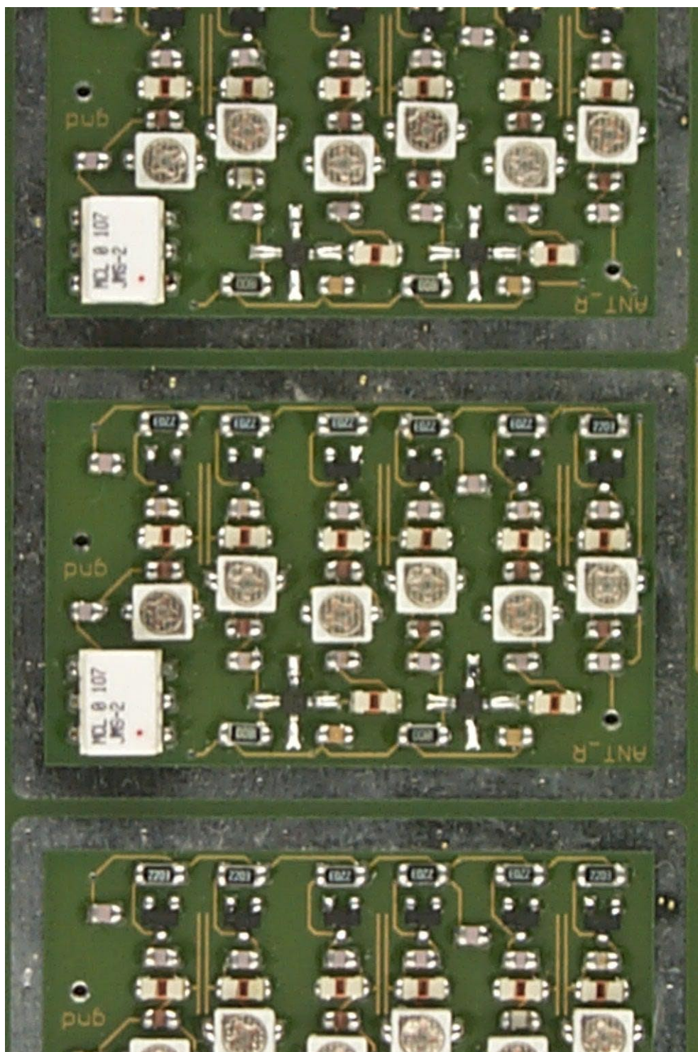
20273eut19.jpg: DEBEG 3400, radio part, PCB, RF-filter-unit
