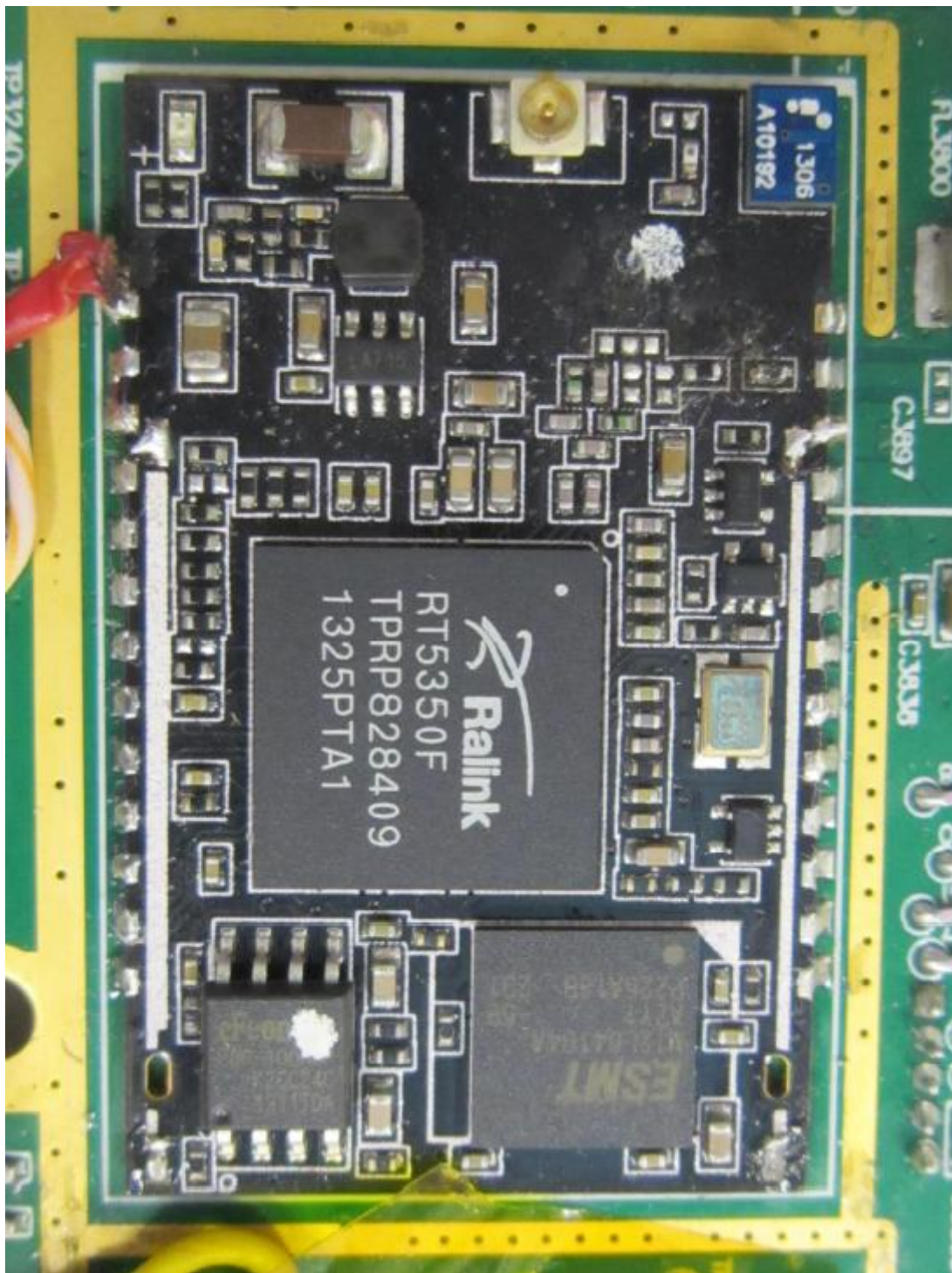
WiFi Module Circuit with RF Shield Removed
