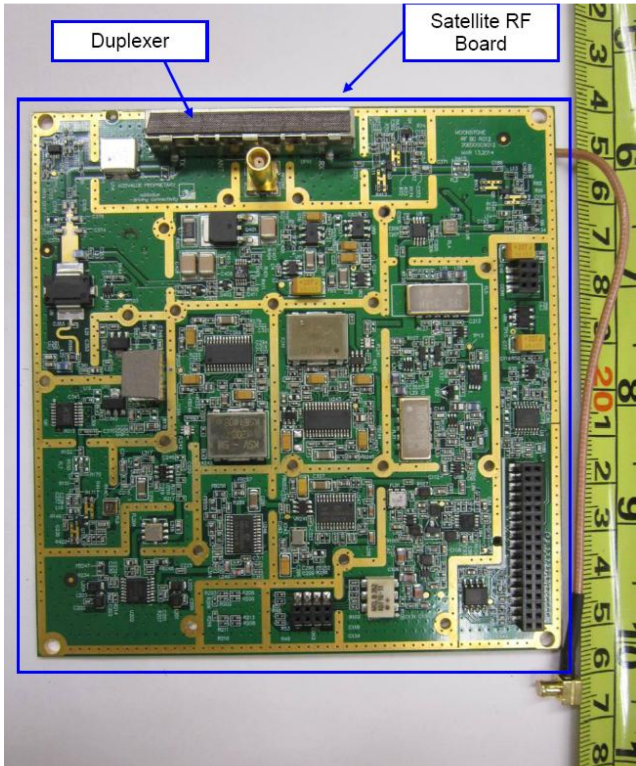
Satellite RF PCBA Component Side
