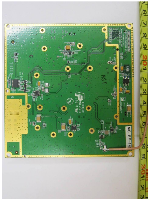
RF Module Circuit with RF Shield Removed
