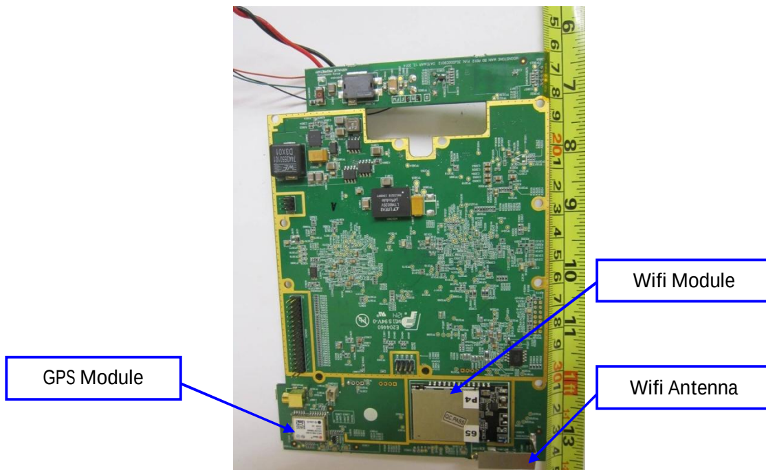
Base-Band & WiFi Module Circuit with RF Shield Removed
