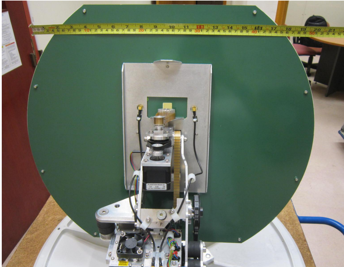
Antenna Unit Main-Board PCB Trace Side
