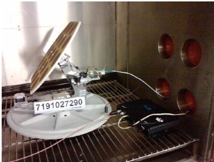
Frequency Stability (Voltage Variation) Test Setup
