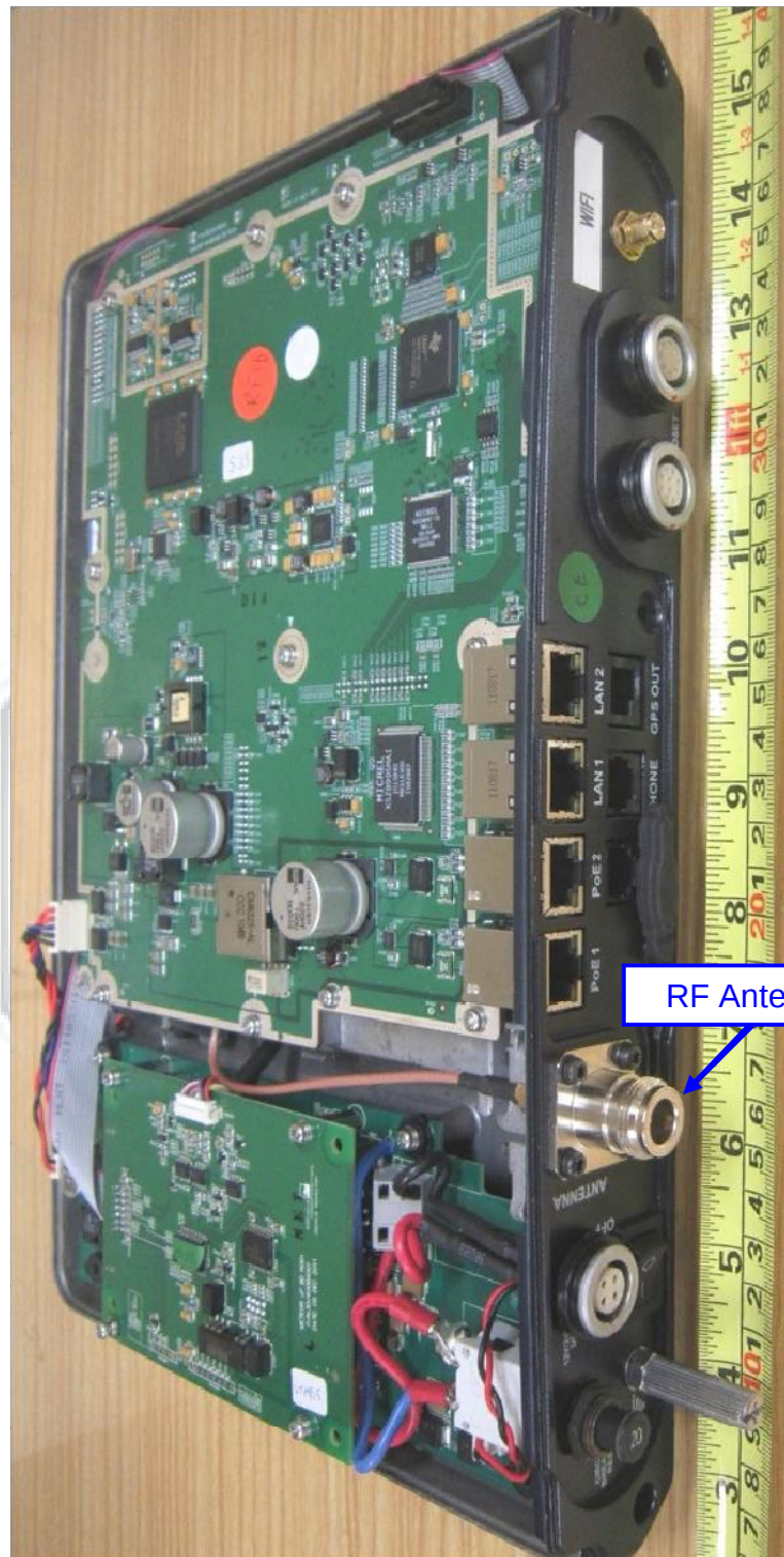
Internal View
