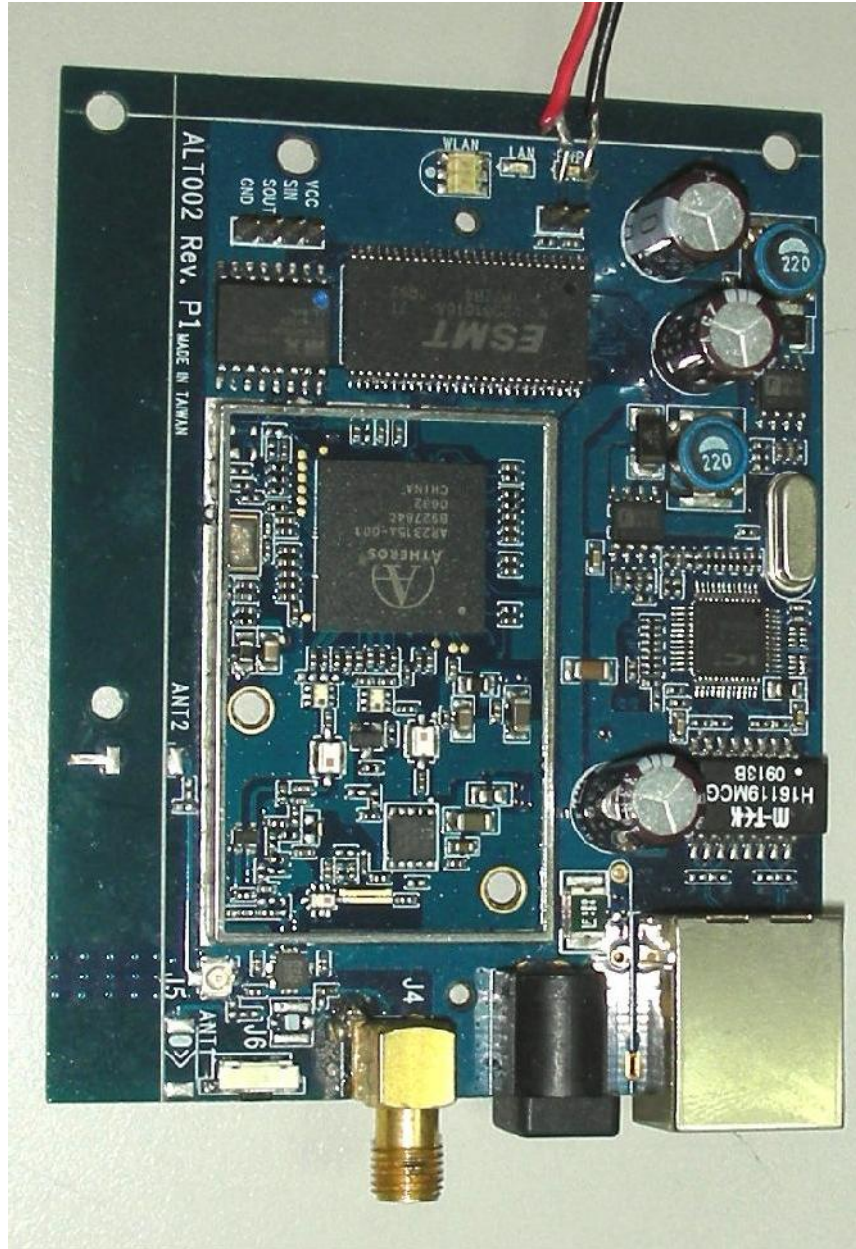
WiFi Module Circuit with RF Shield Removed Component Side
