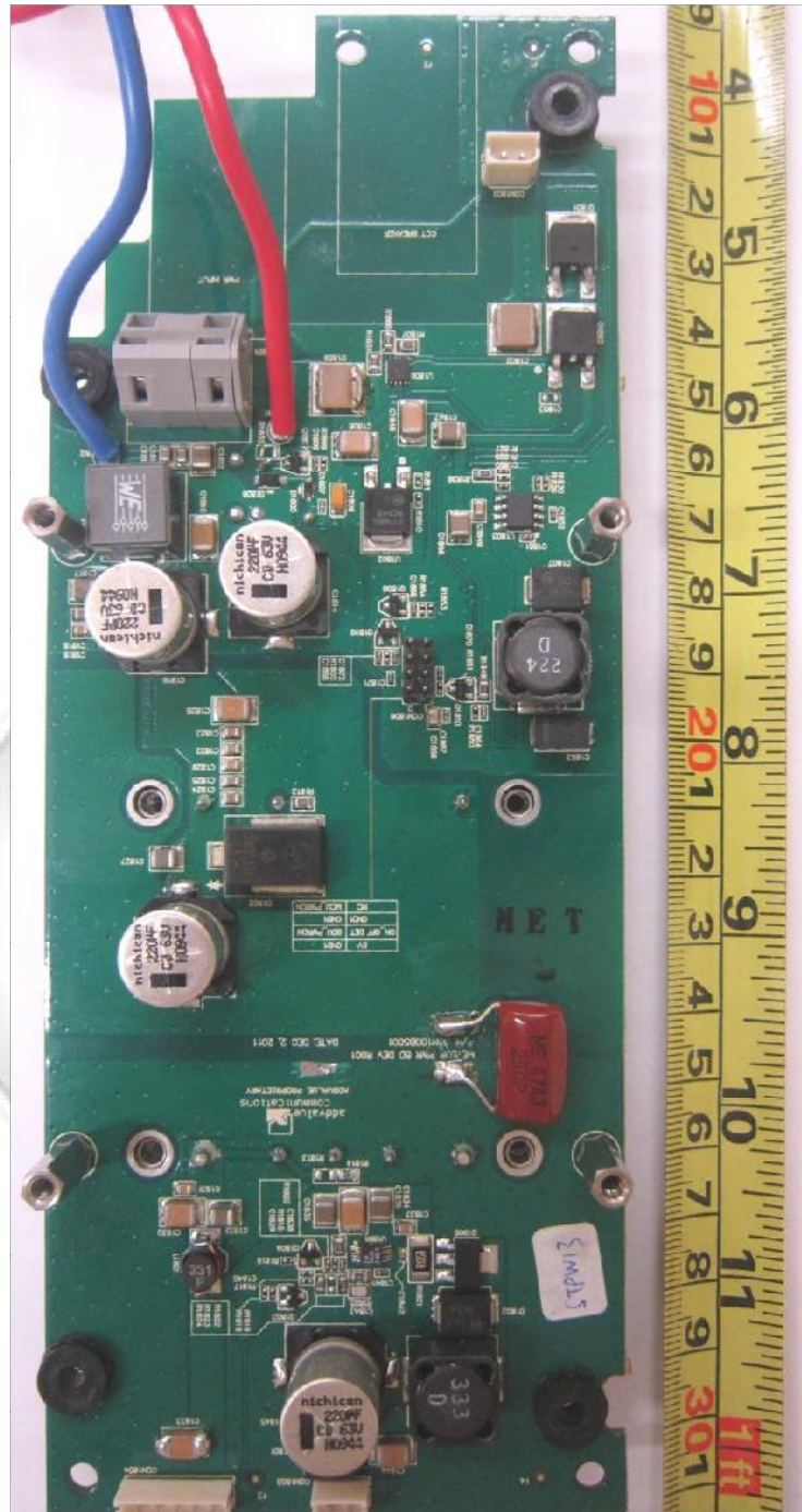
Power Supply PCB Component Side
