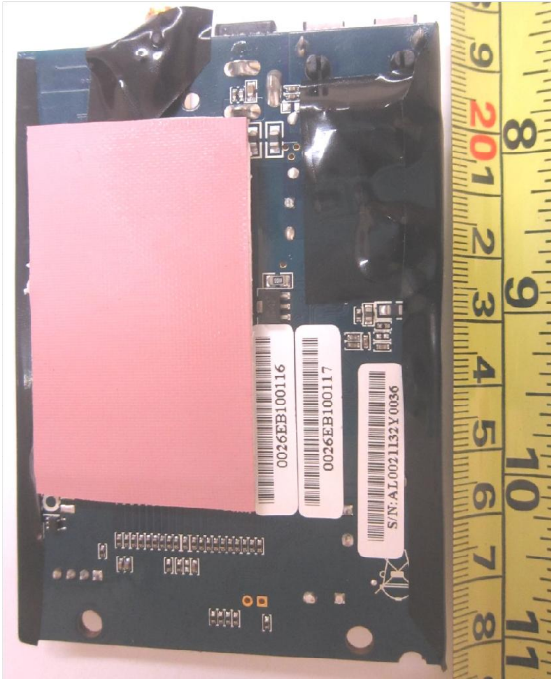
WiFi Module PCB Trace Side
