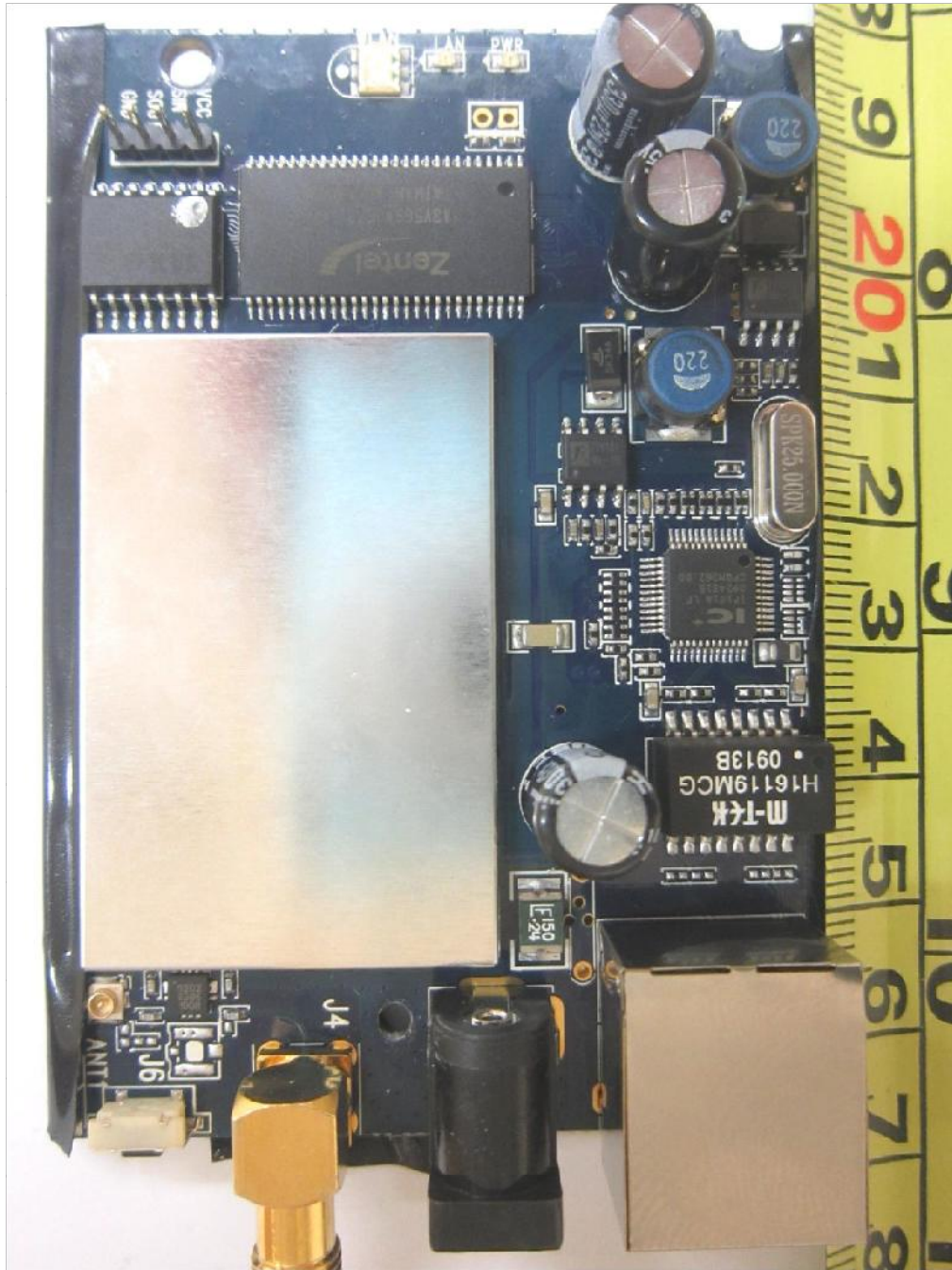
WiFi Module PCB Component Side
