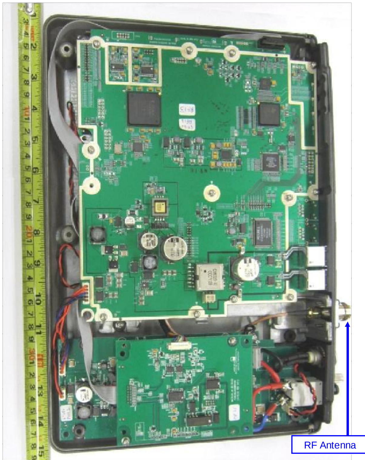
Internal View
