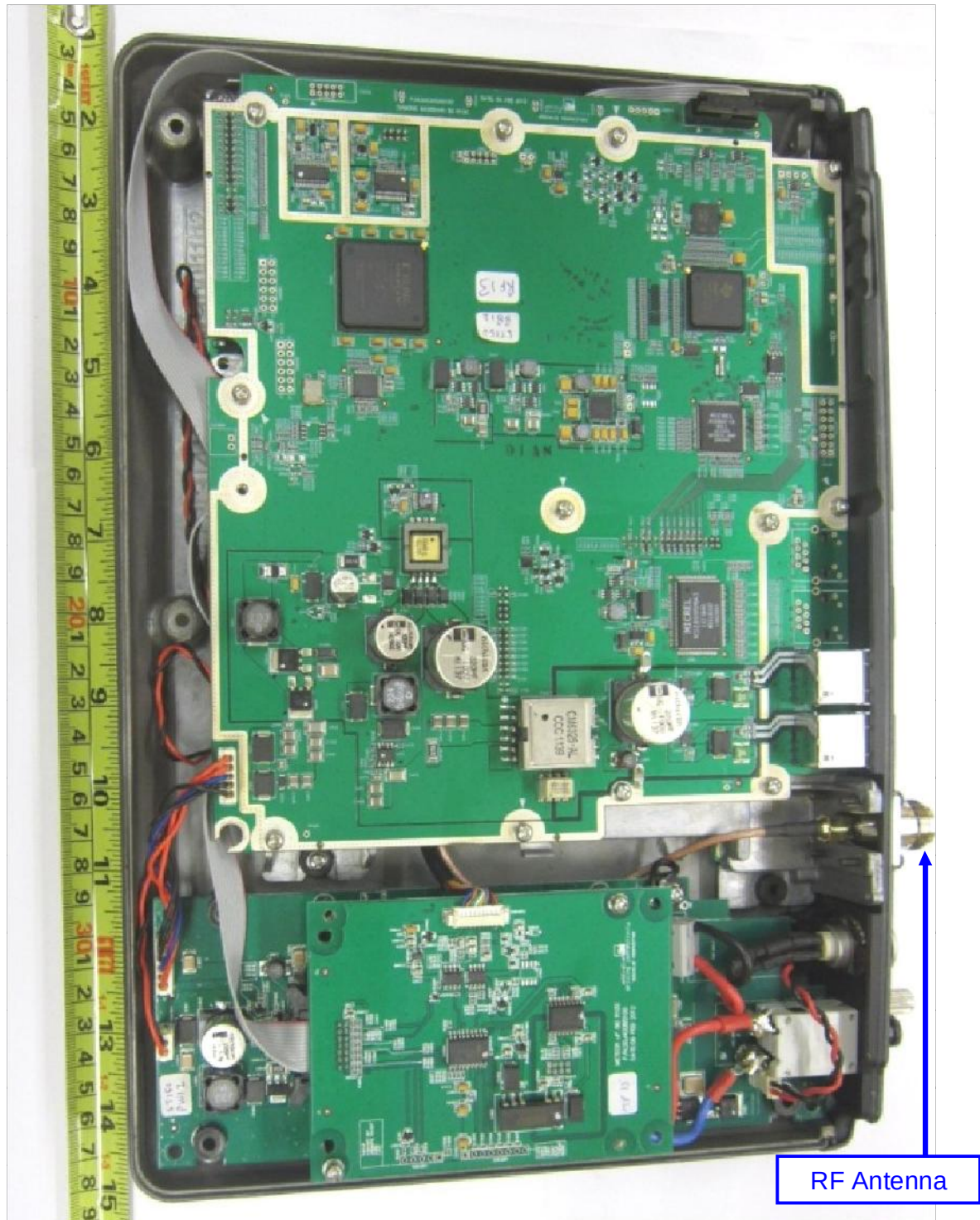
Internal View
