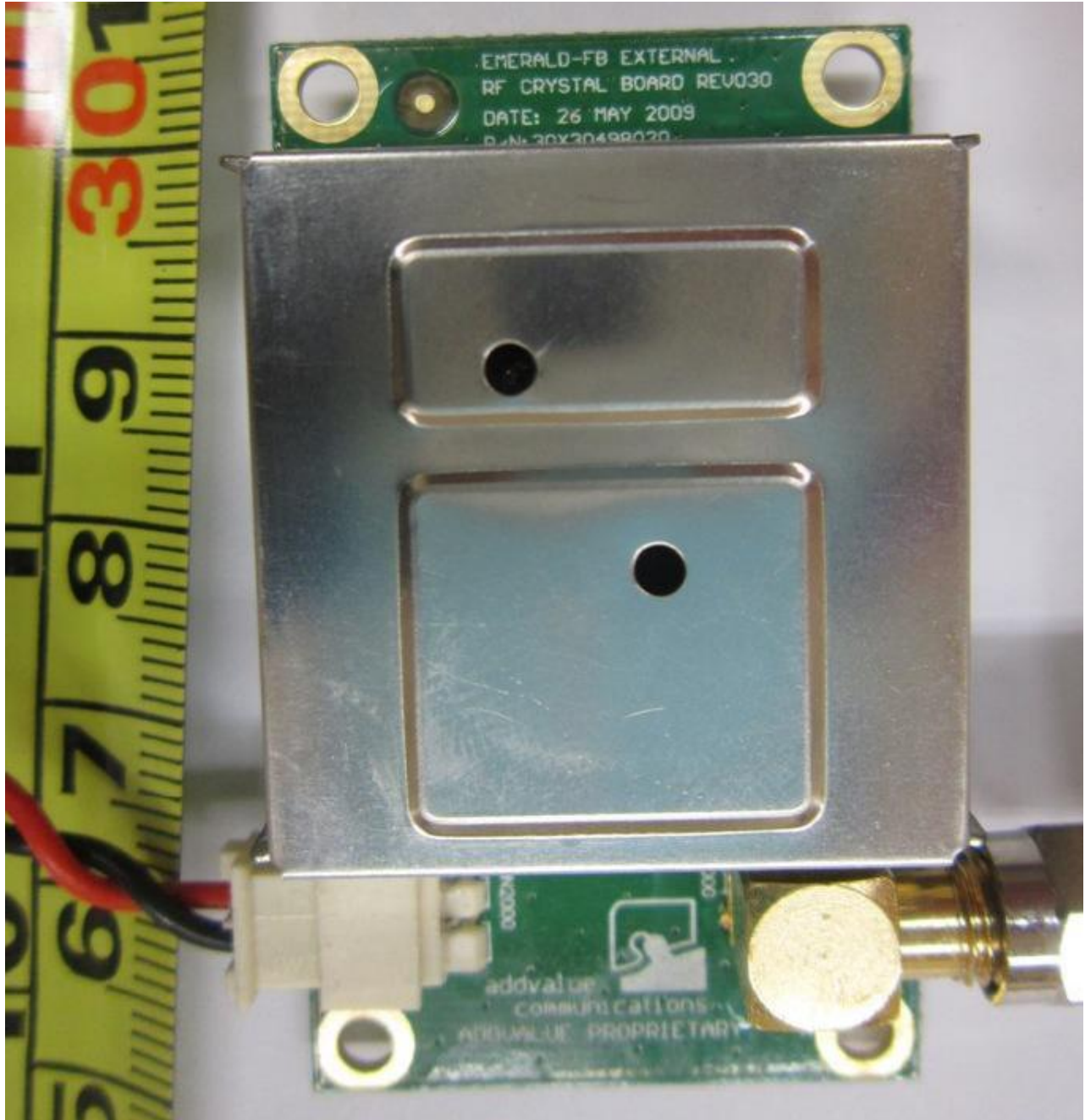
Crystal Board PCB Component Side
