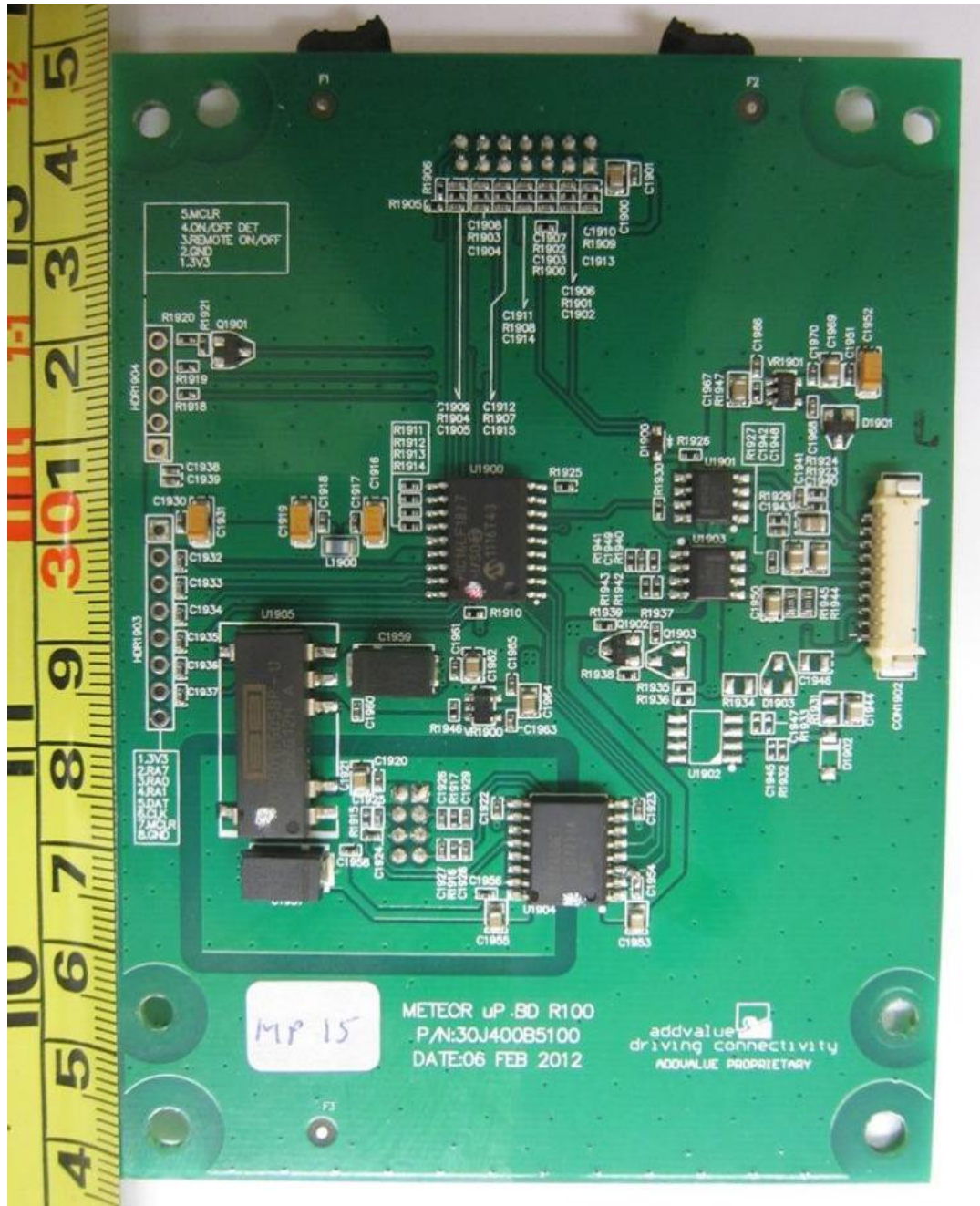
Microprocessor Board PCB Component Side
