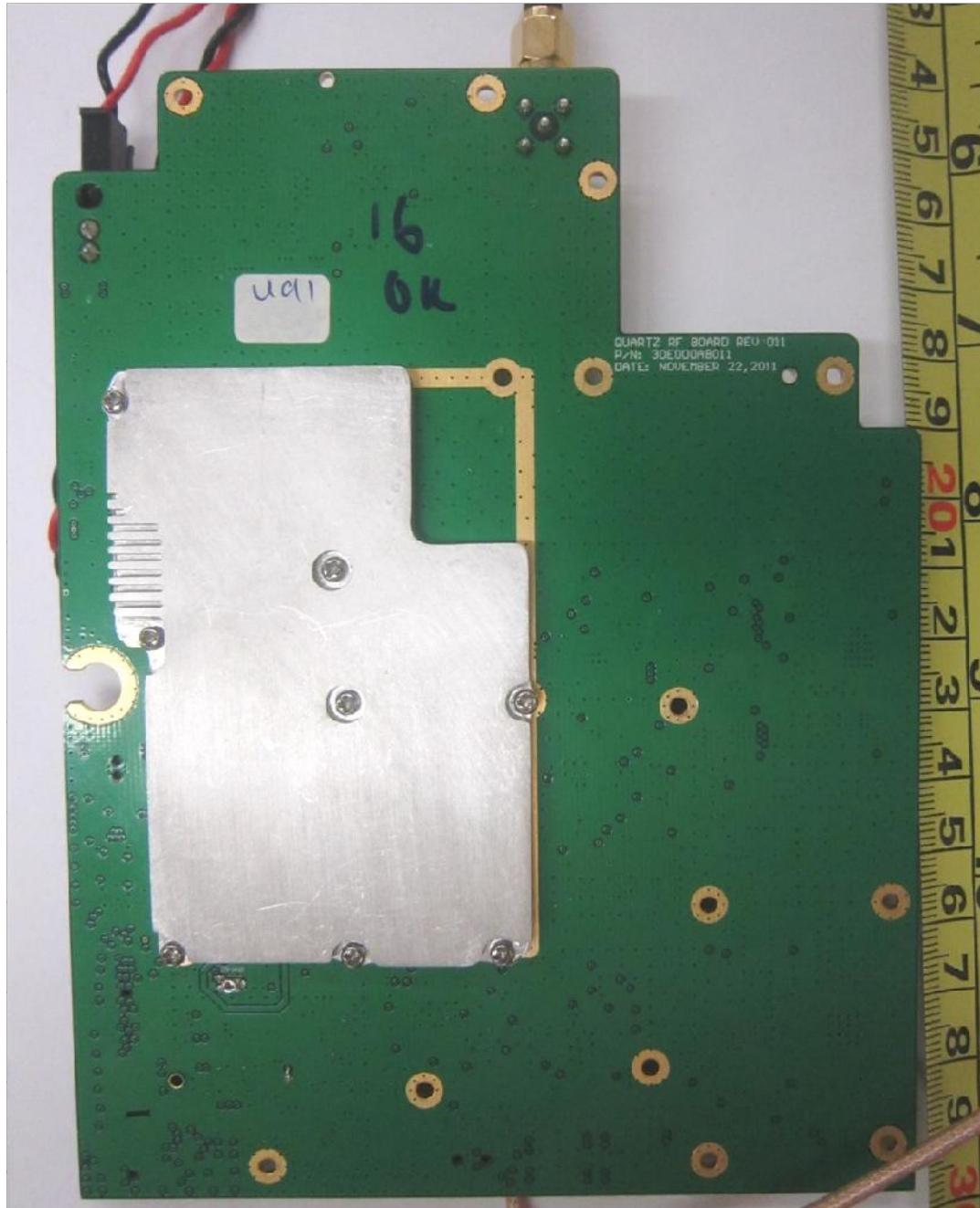
RF Module PCB Trace Side
