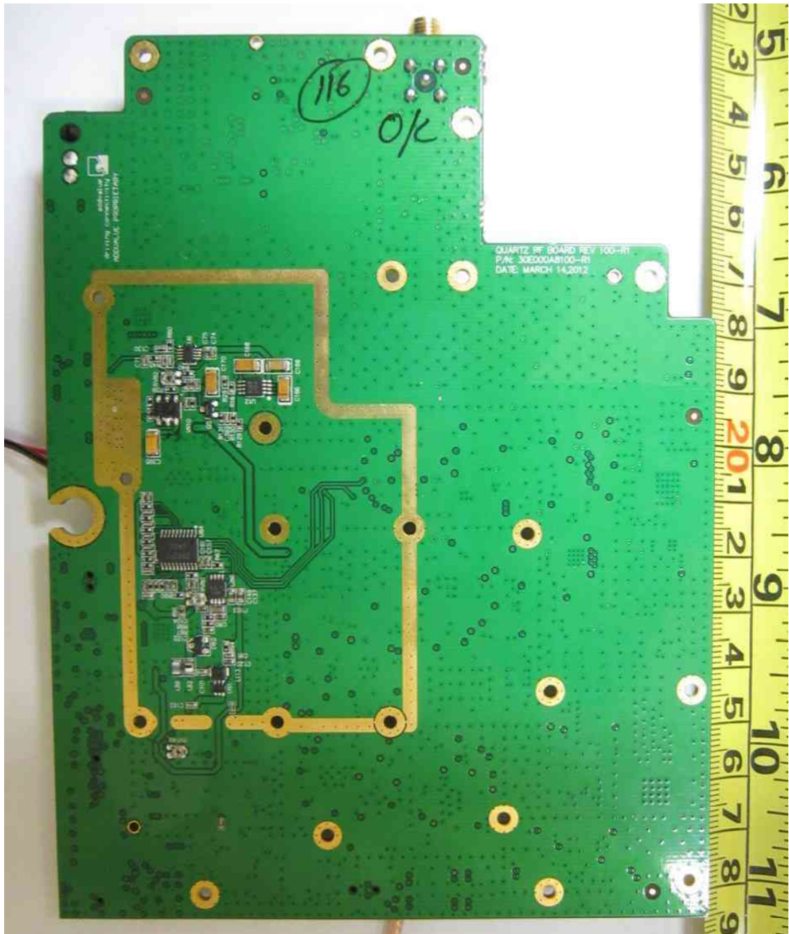
RF Module Board PCB Trace Side
