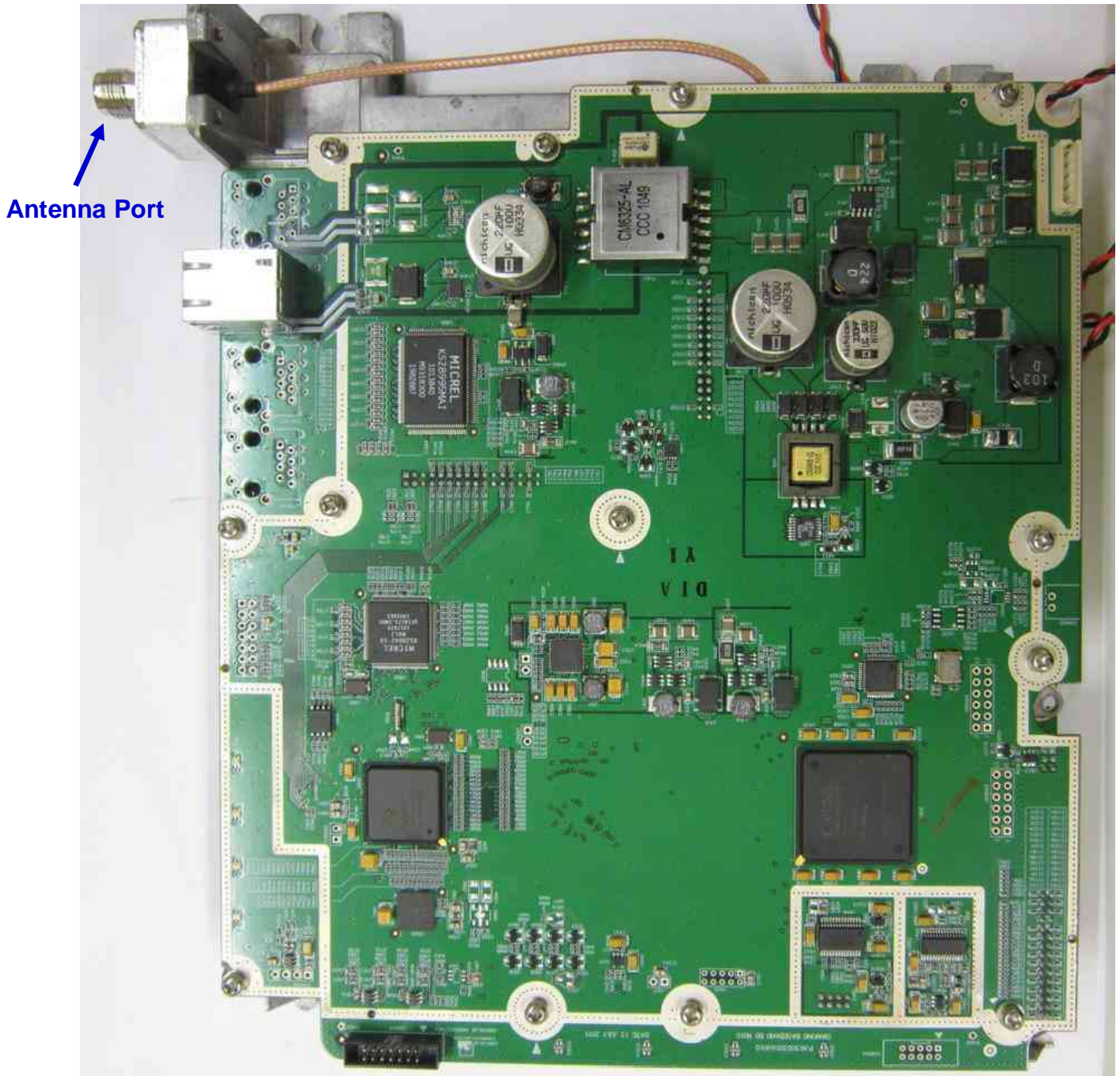
Base-Band Board PCB Component Side
