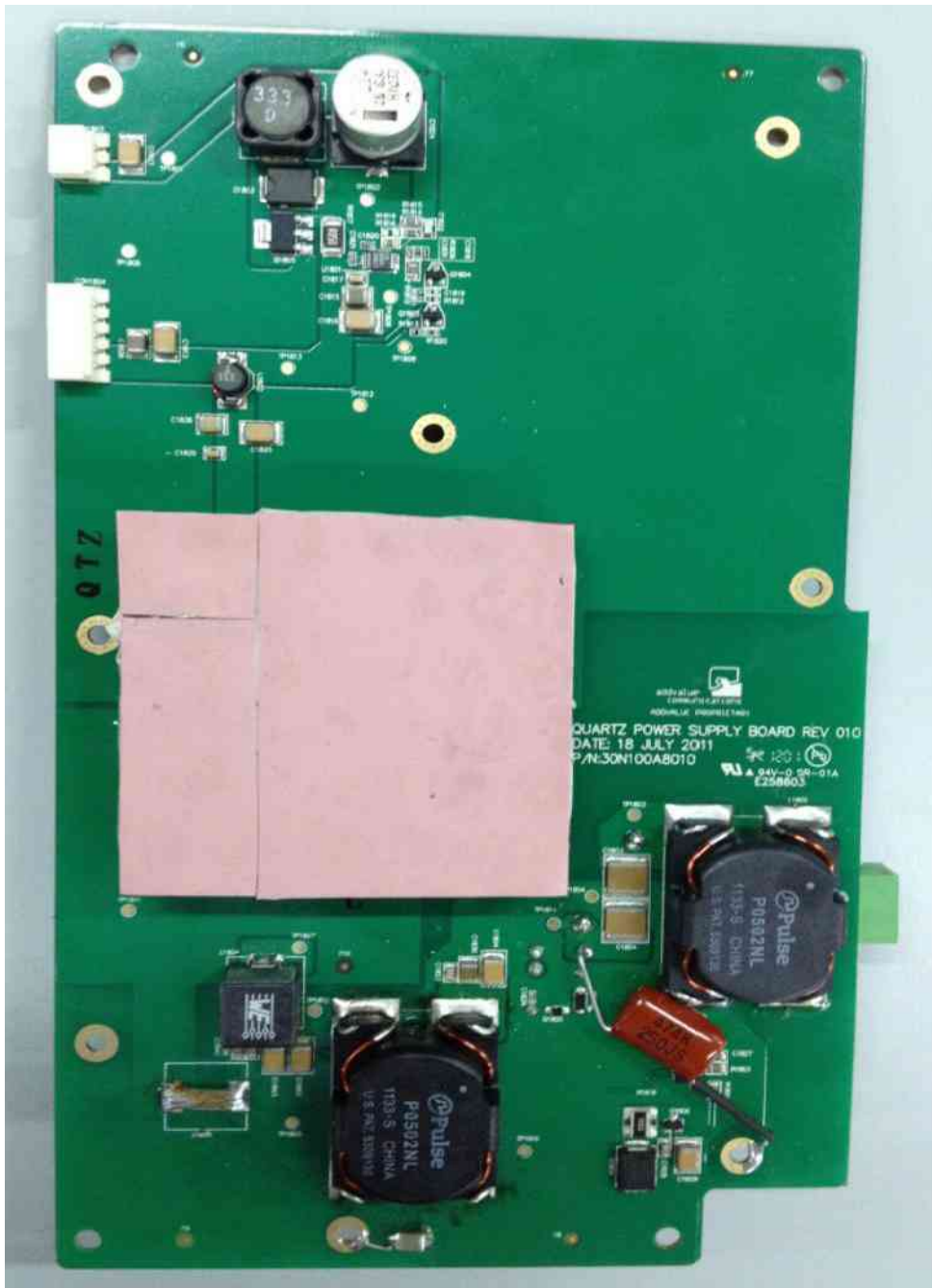
Power Supply Board PCB Trace Side
