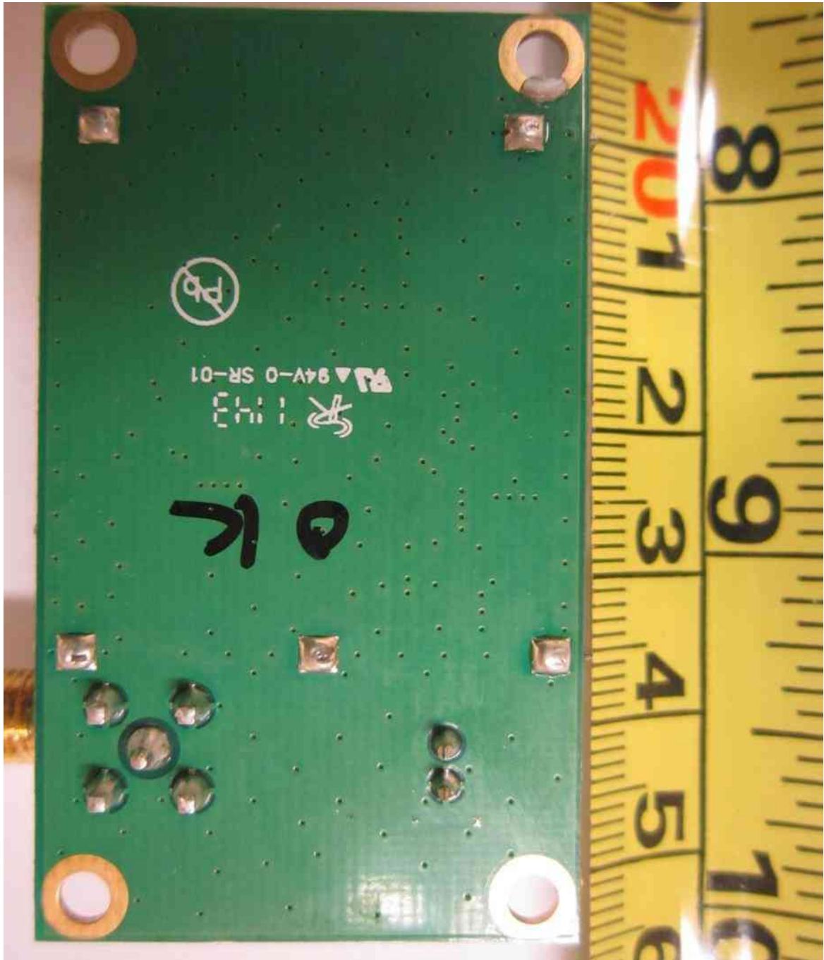
Crystal Board PCB Trace Side
