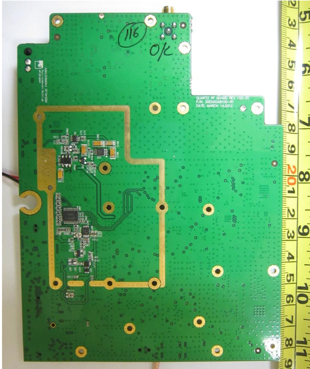
RF Module Circuit with RF Shield Removed
