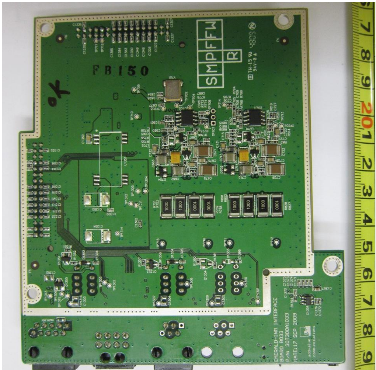
Interface Board PCB Trace Side
