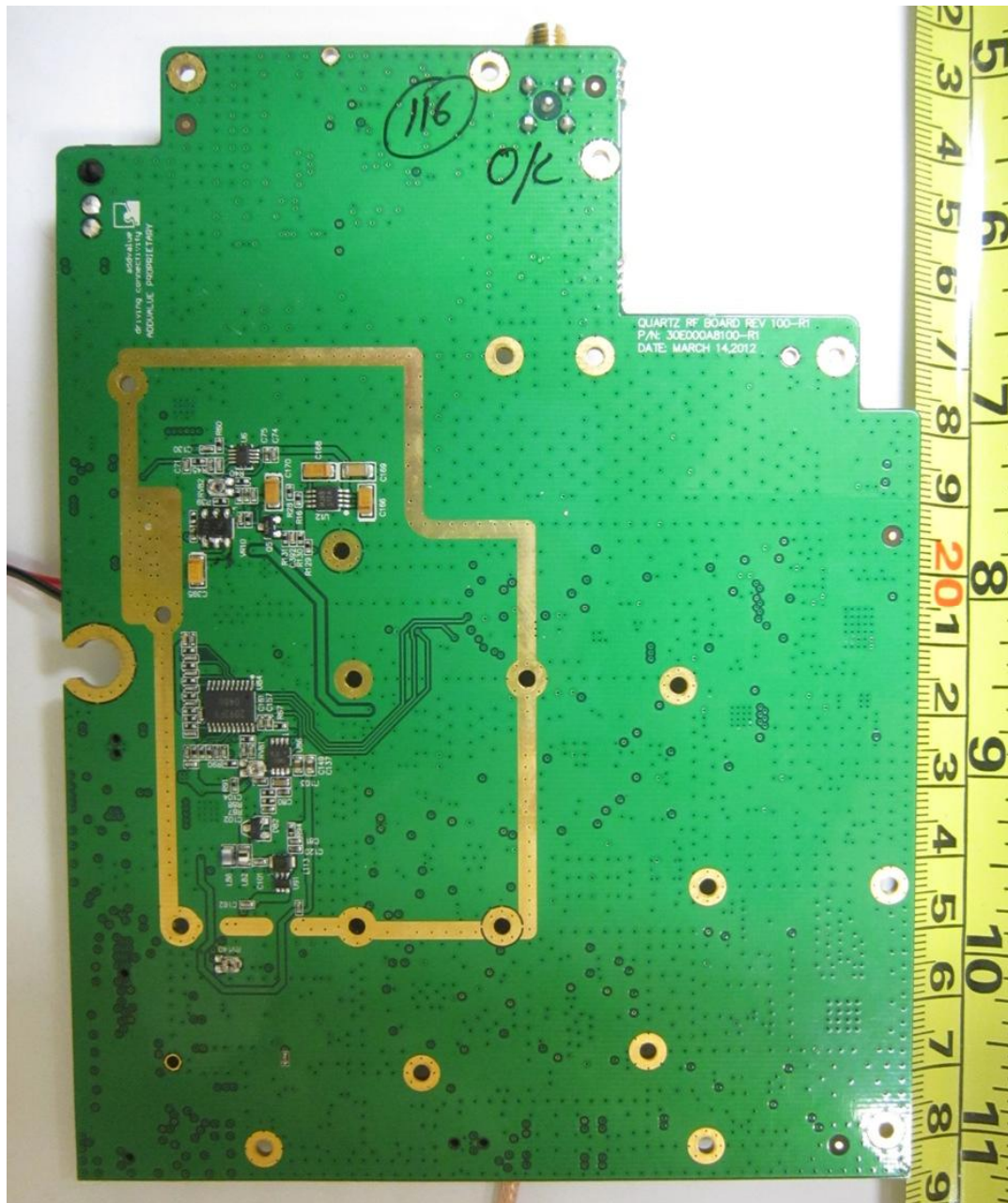
RF Module Board PCB Trace Side
