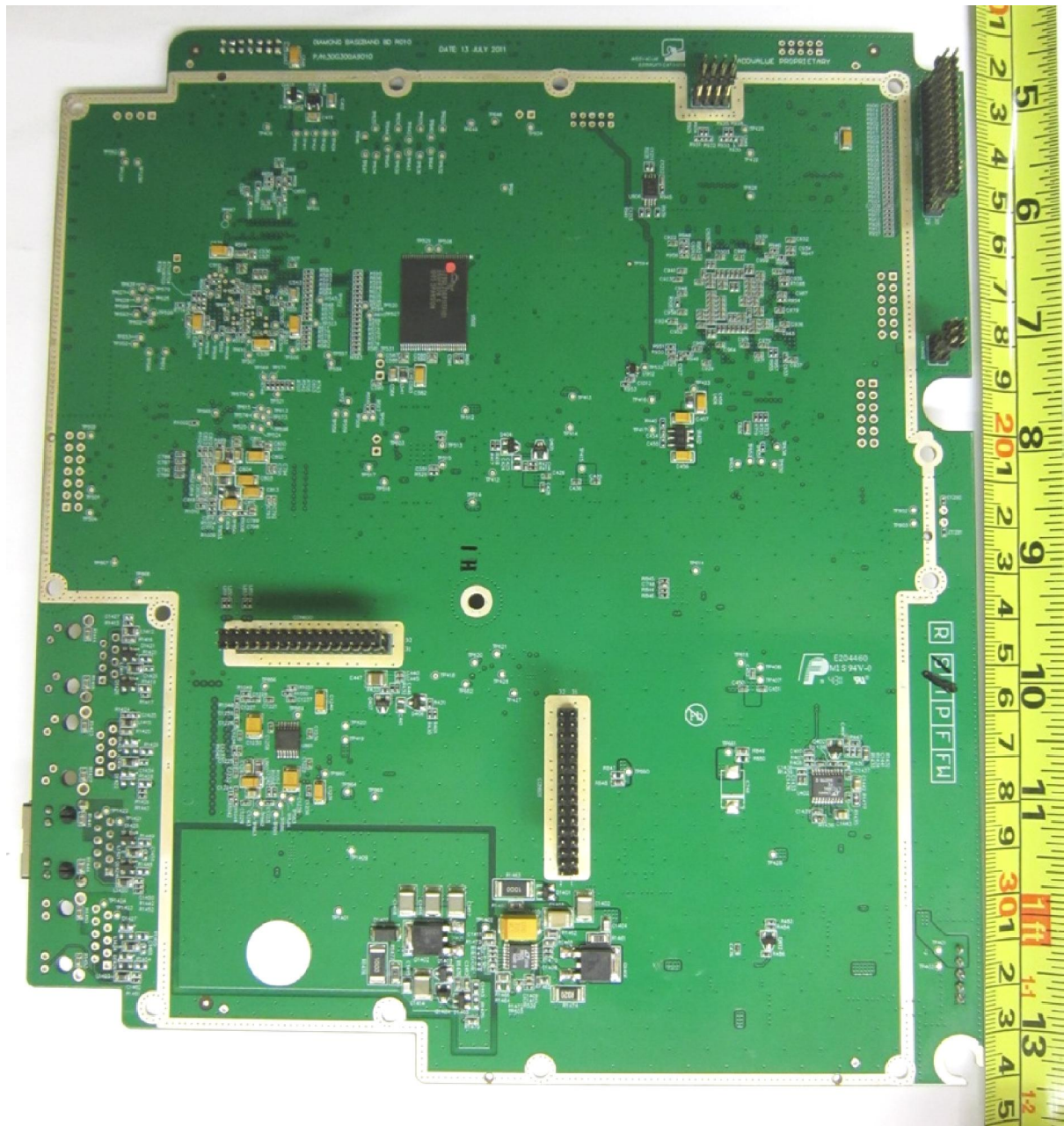
Base-Band Board PCB Trace Side
