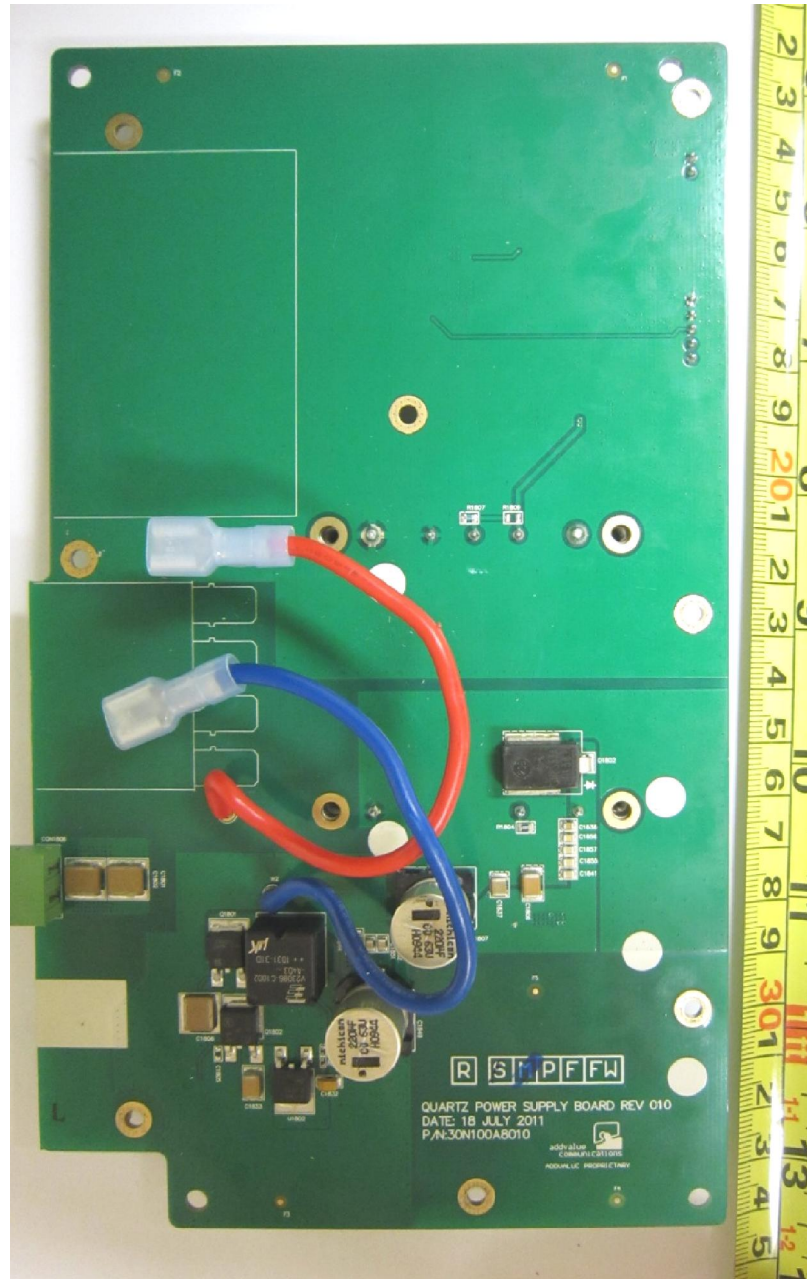
Power Supply Board PCB Component Side
