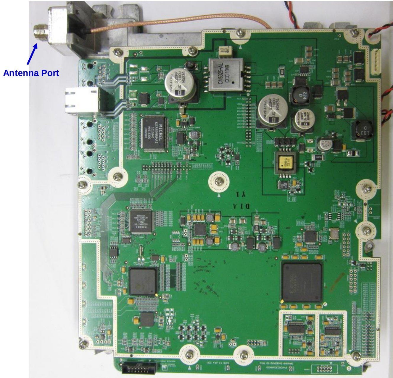
Base-Band Board PCB Component Side
