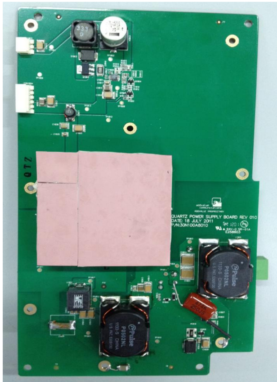
Power Supply Board PCB Trace Side
