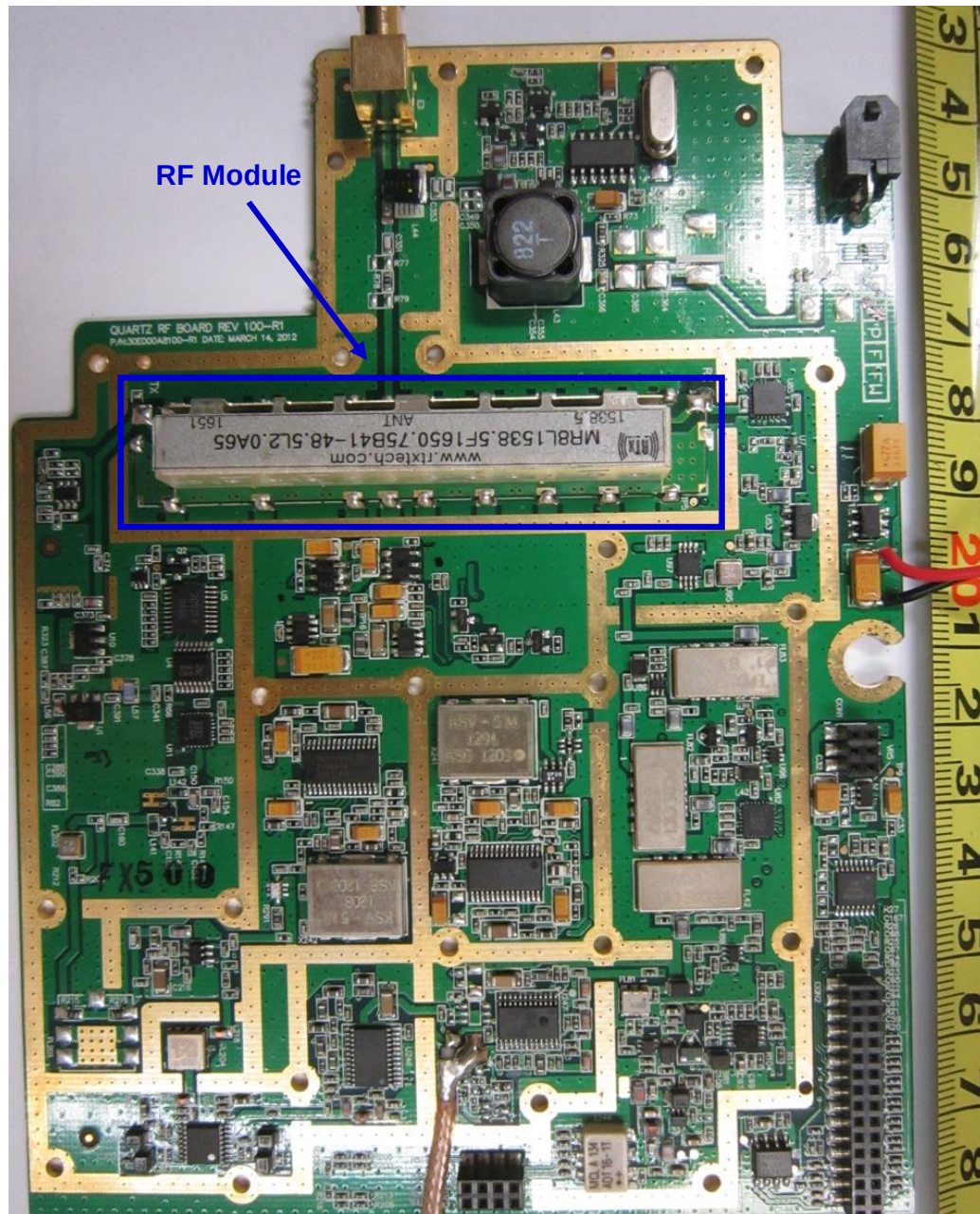
RF Module Board PCB Component Side
