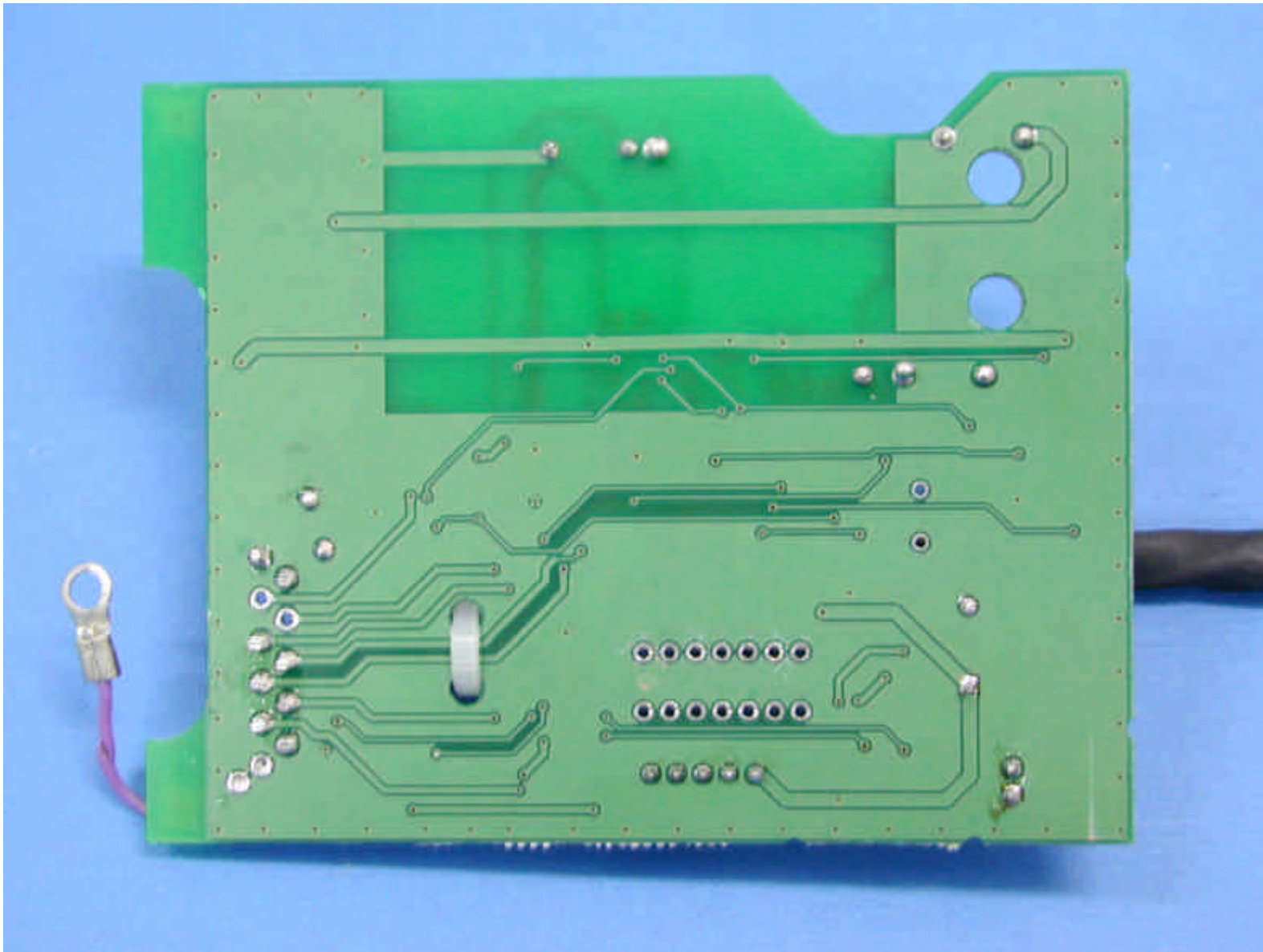
Middle PCB second side
