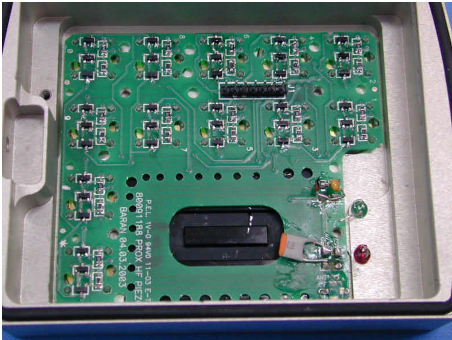
Bottom PCB first side
