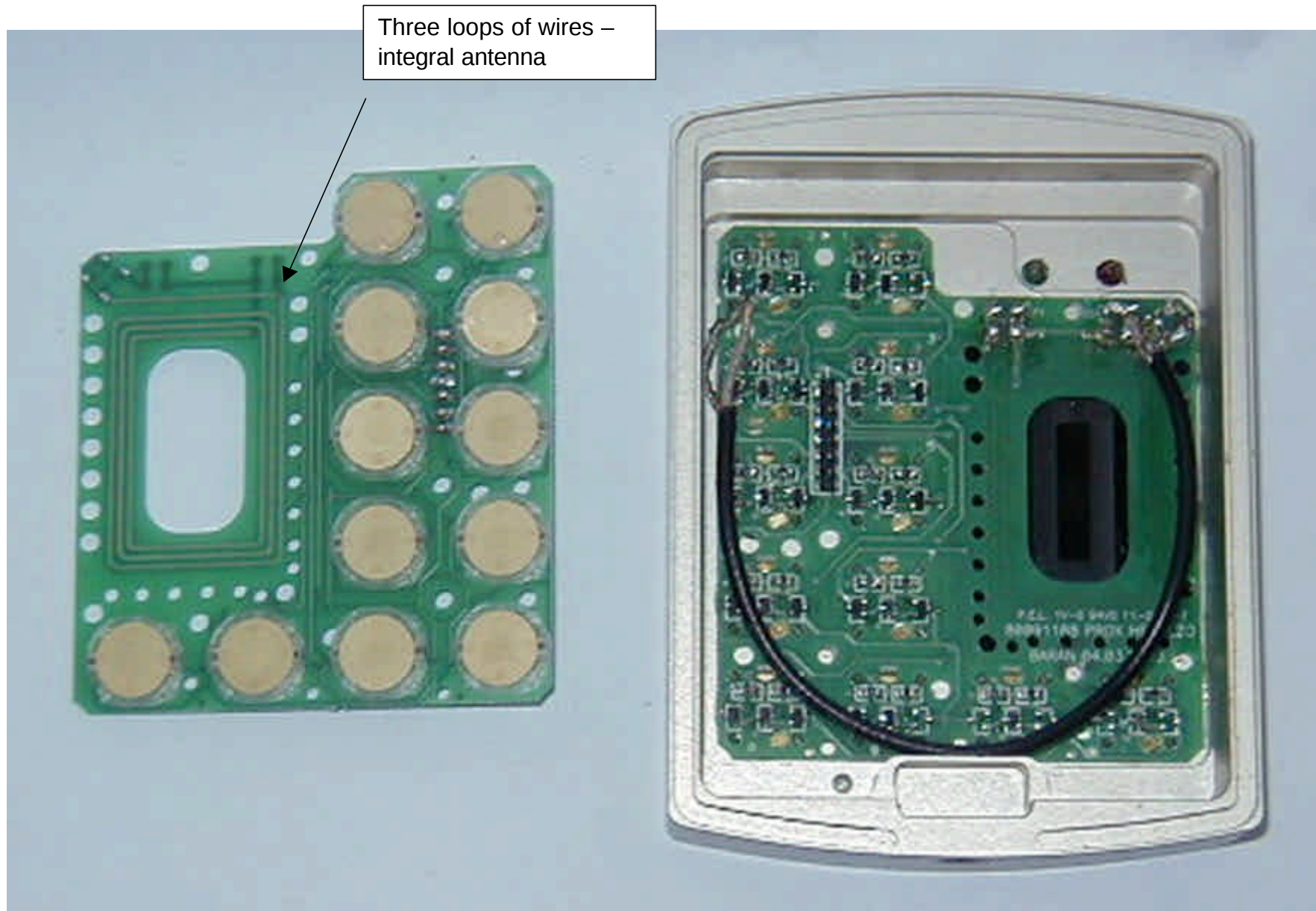
Bottom PCB second side
