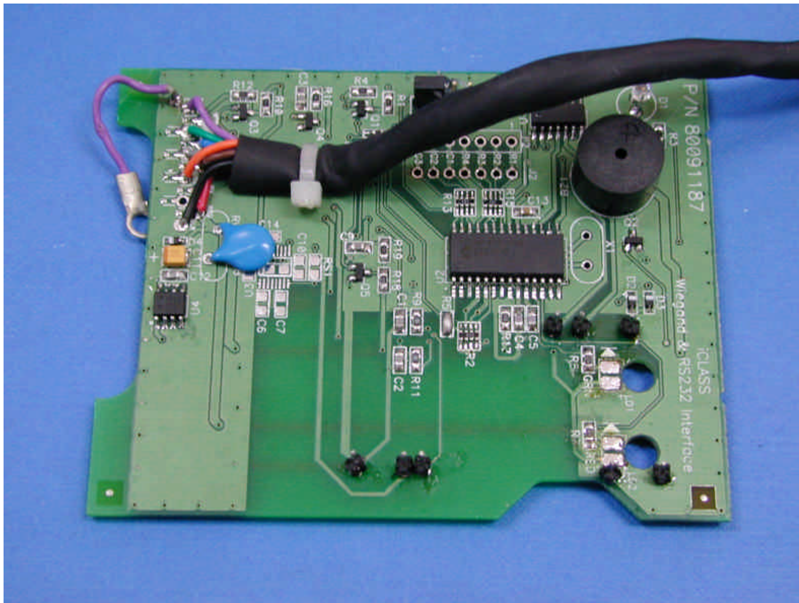
Middle PCB first side_2
