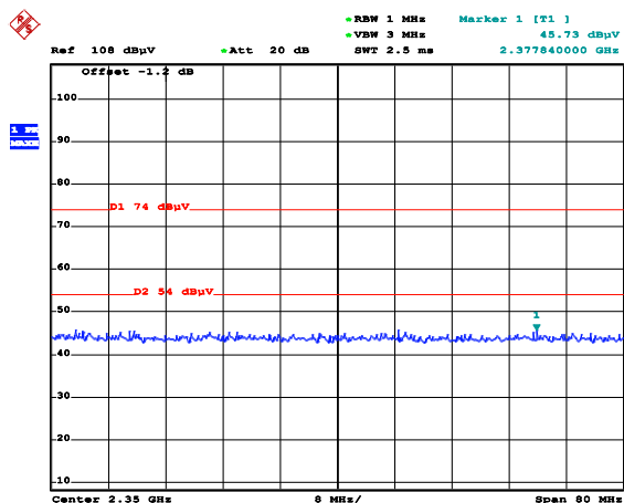
Figure 5. Plot of the Band Edge (Radiated) 802.11b
