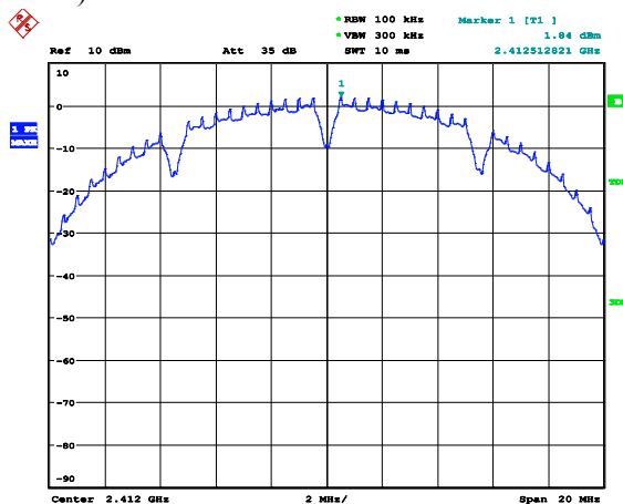
Figure 2. Plot of the Power Density (Conducted)
