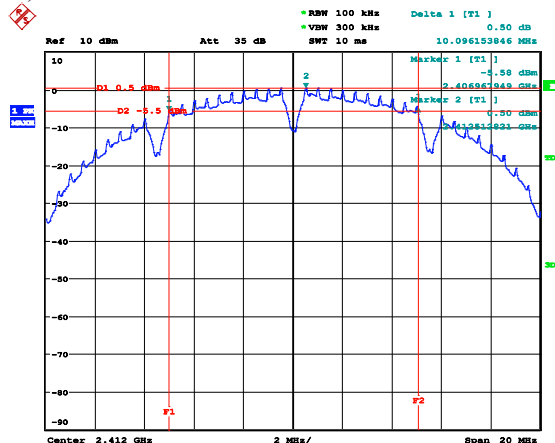
Figure 3. Plot of the 6dB Bandwidth (Conducted) 802.11b
