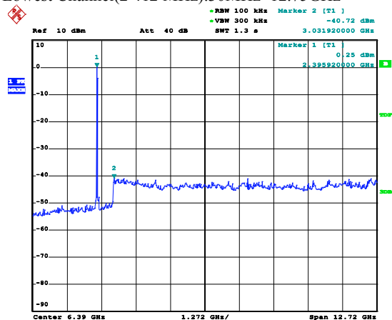
Figure 6. Plot of the Spurious RF conducted emissions 802.11b
