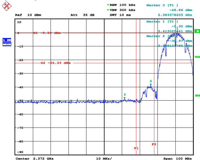
Figure 4. Plot of the Band Edge (Conducted) 802.11b
