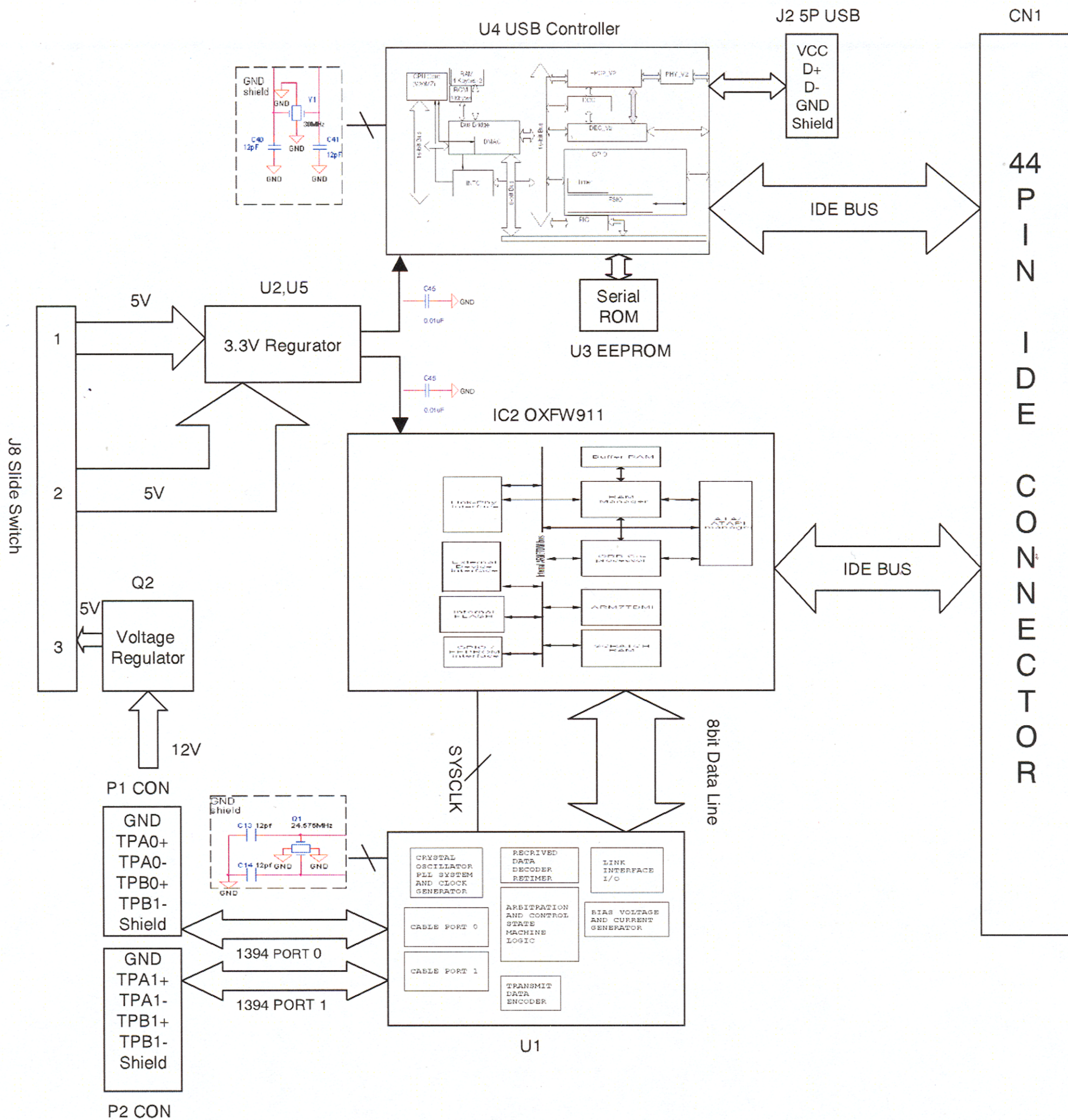
Block Diagram
