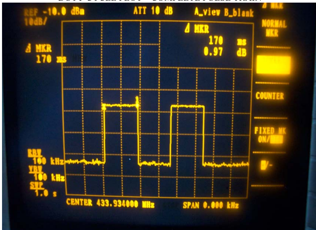
DUTY CYCLE PLOT – COMPLETE PULSE TRAIN
