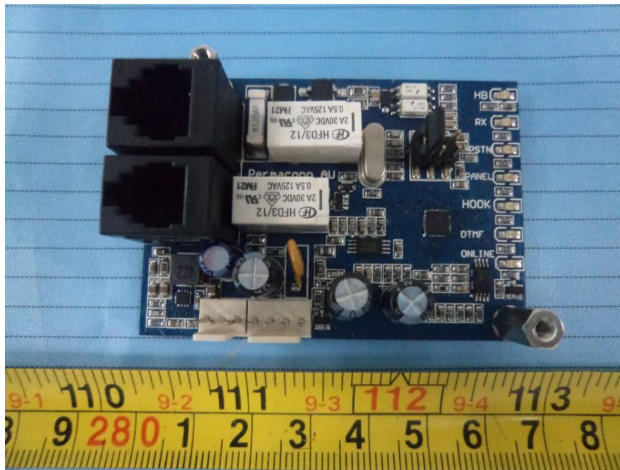
EUT – DI300 Main Board Top View
