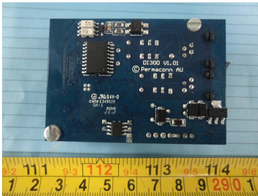
EUT – DI300 Main Board Bottom View
