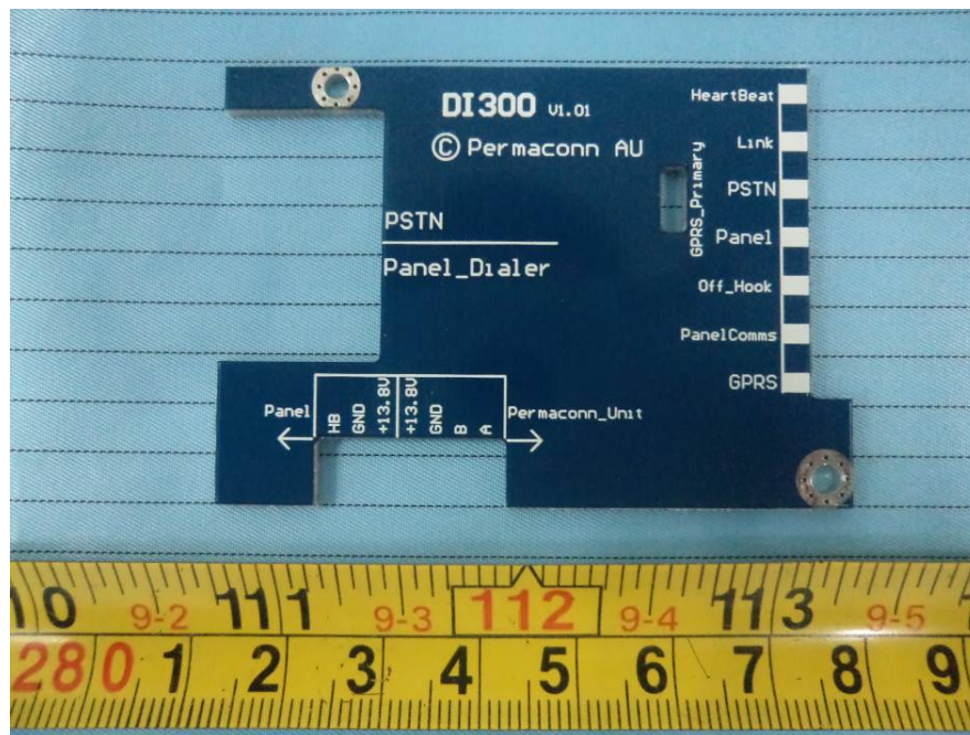
EUT – DI300 Extra Board Top View
