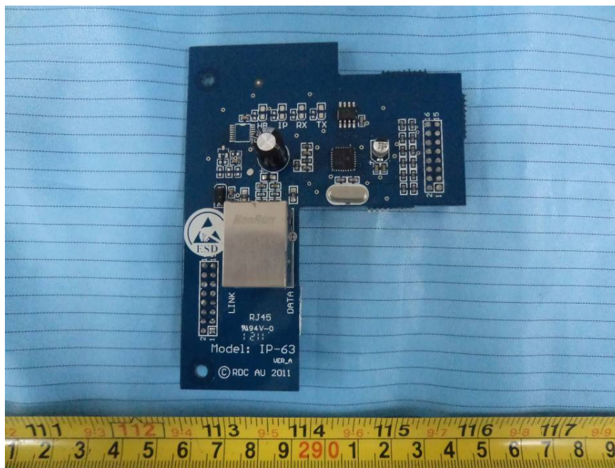
EUT – IP-63 Board Top View
