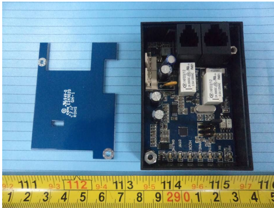
EUT – DI300 Cover off View
