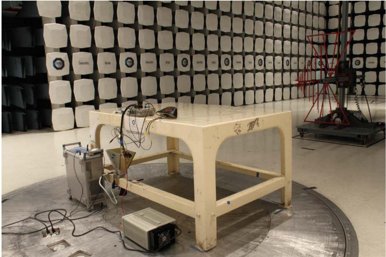
Licensed Radiated Emissions Test Setup (below 1GHz)
