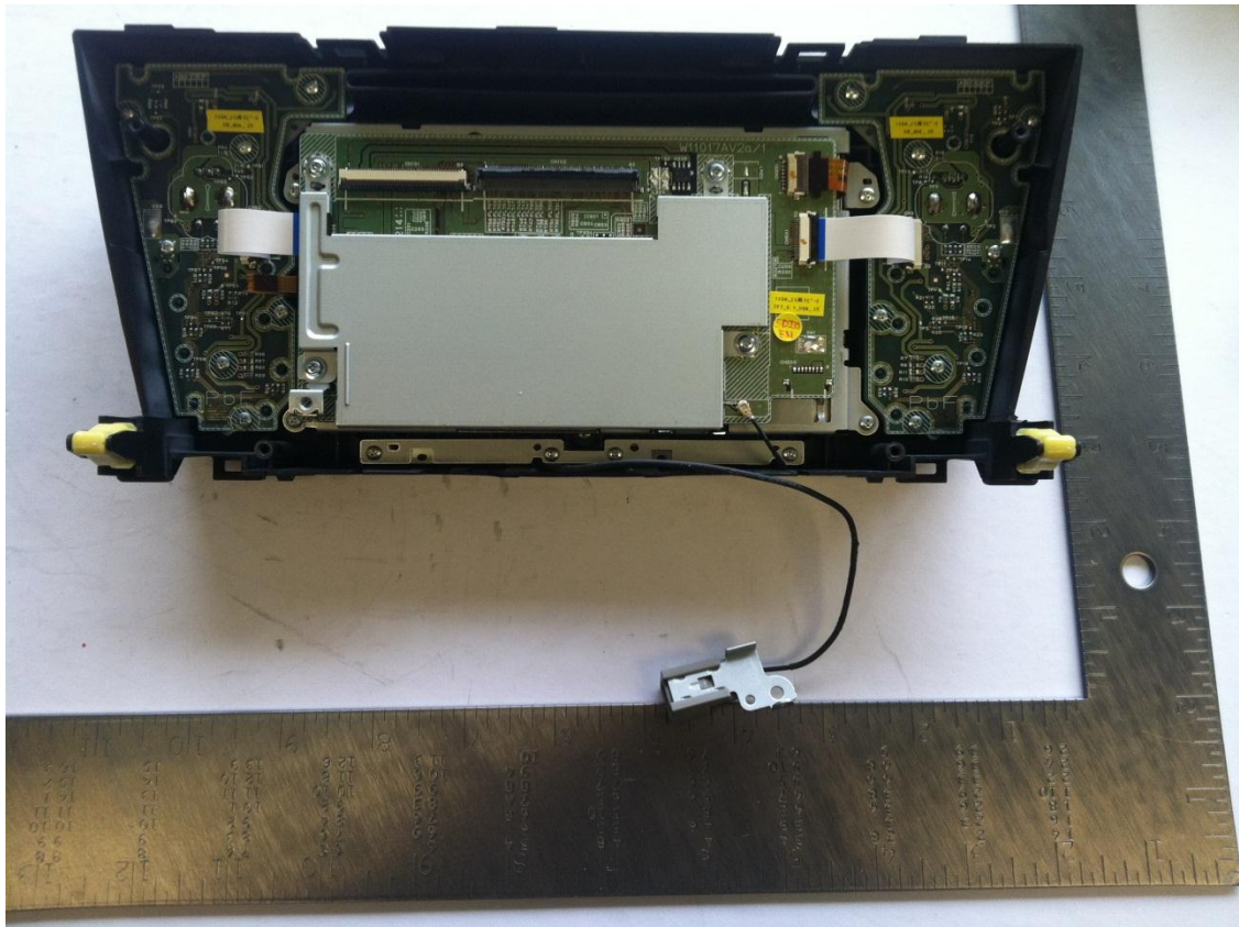
BT antenna at the bottom of the AE 1 (head unit)
