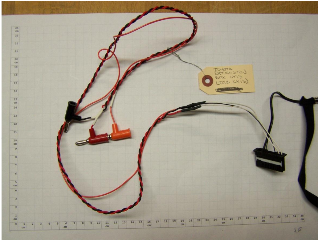
Cable 1 (power supply cable of EUT A)
