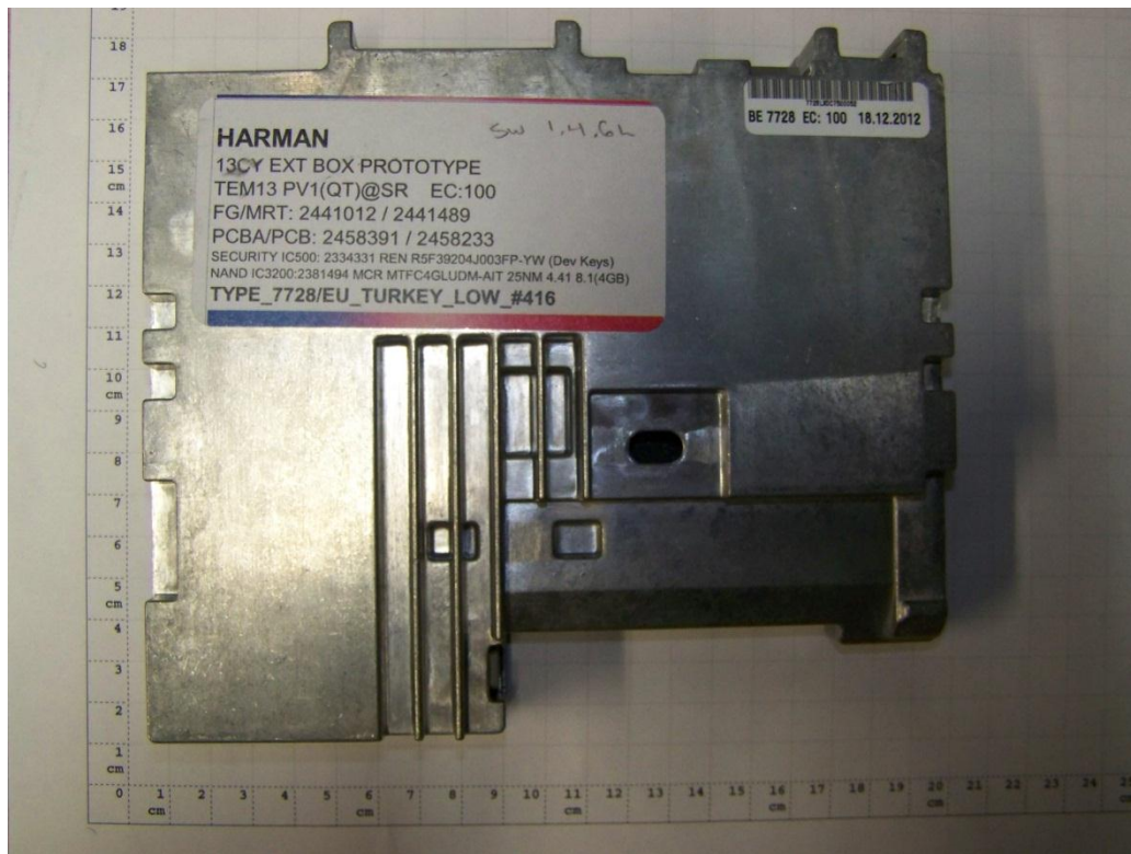
EUT A (top side)
