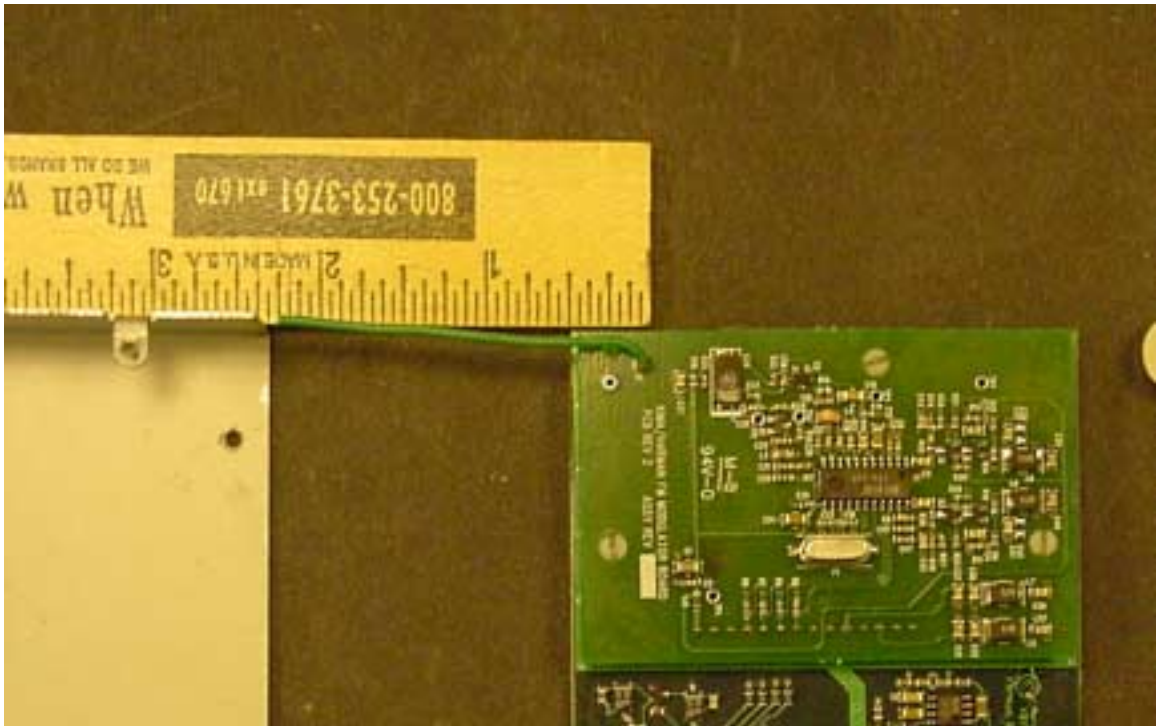
QNG-02001 photo of modulator board assembled to motherboard. Also showing antenna length of 2.25 inches.
