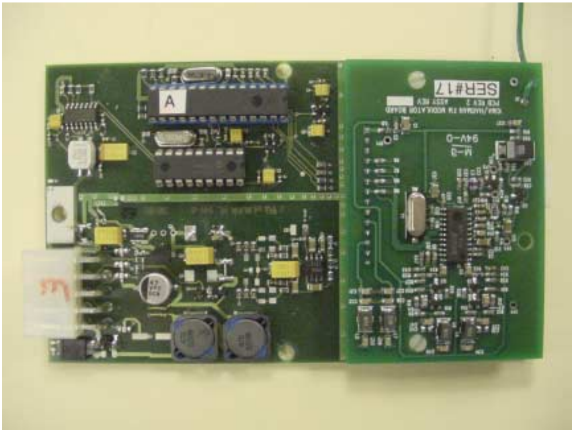
QNG-02001 Component side of motherboard attached to modulator/Tx board.
