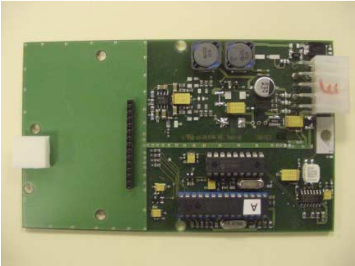
QNG-02001 Component Side of motherboard.
