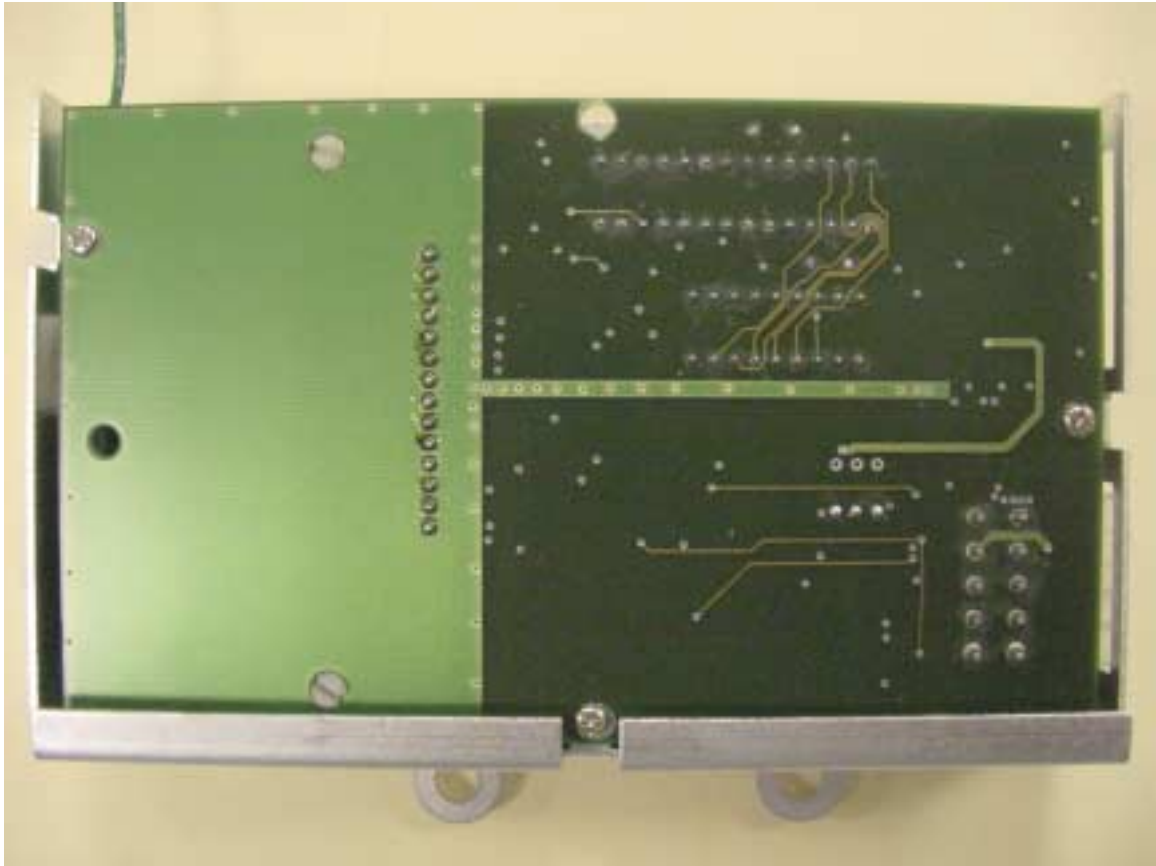
QNG-02001 Solder side of motherboard as installed in the housing.
