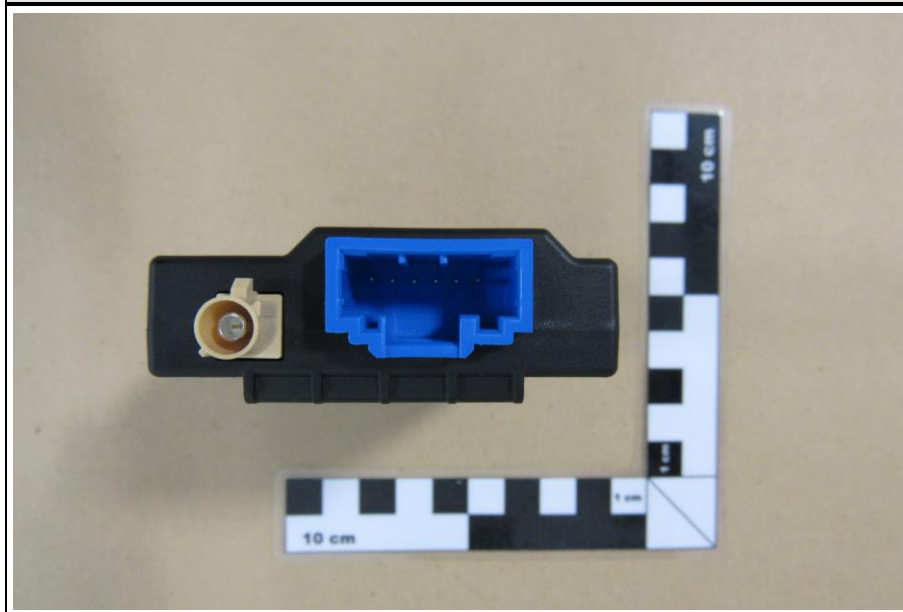
EUT Connector Side
