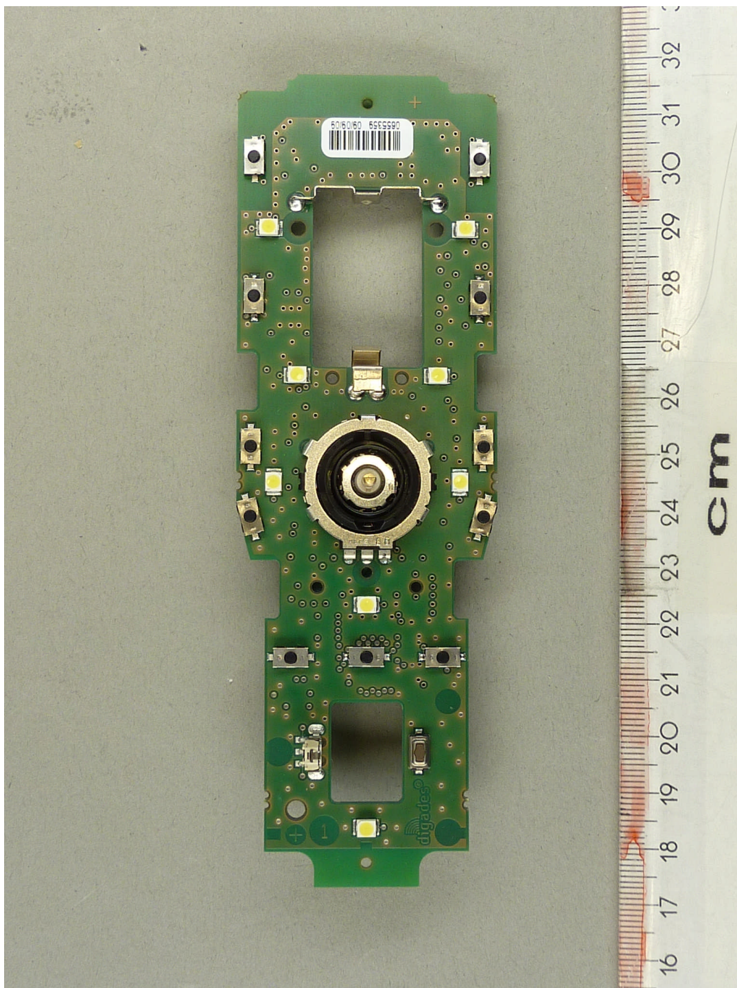
93032_24.jpg BY83x Remote Control , PCB, top view
