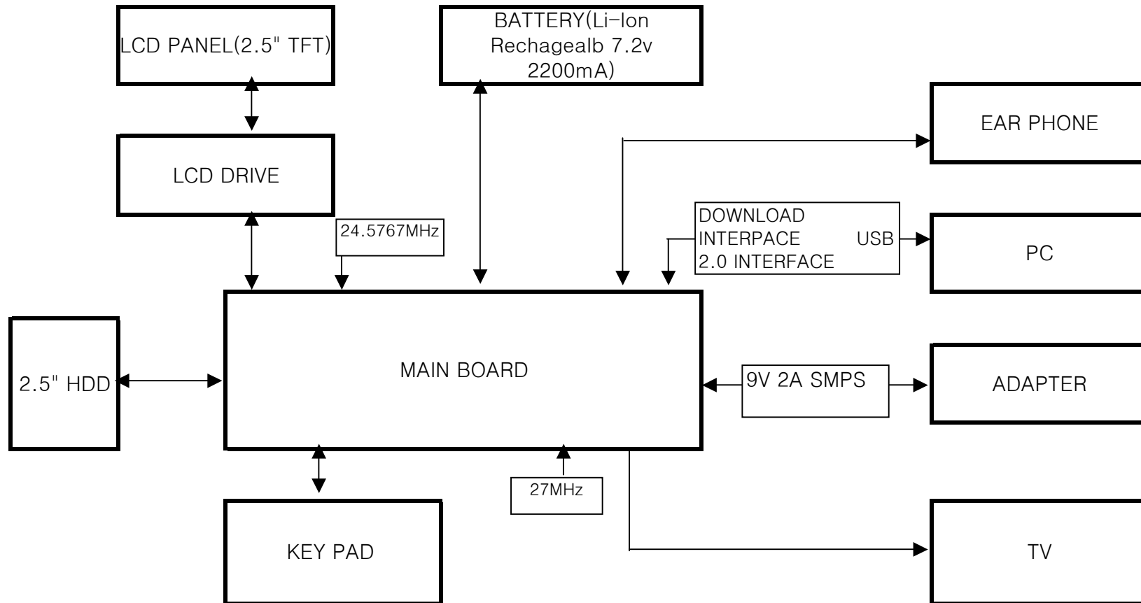
DDP- 1000 BLOCK DIAGRAM
